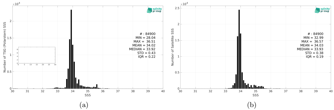
Figure 2: Histograms of SSS from TSG (Polarstern) (a) and SMOS SSS L4 v1 - Weekly (CMEMS-CNR) (b) considering all match-up pairs per bins of 0.1 over the Roaring Forties and Furious Fifties Pi-MEP region and for the full satellite product period.
