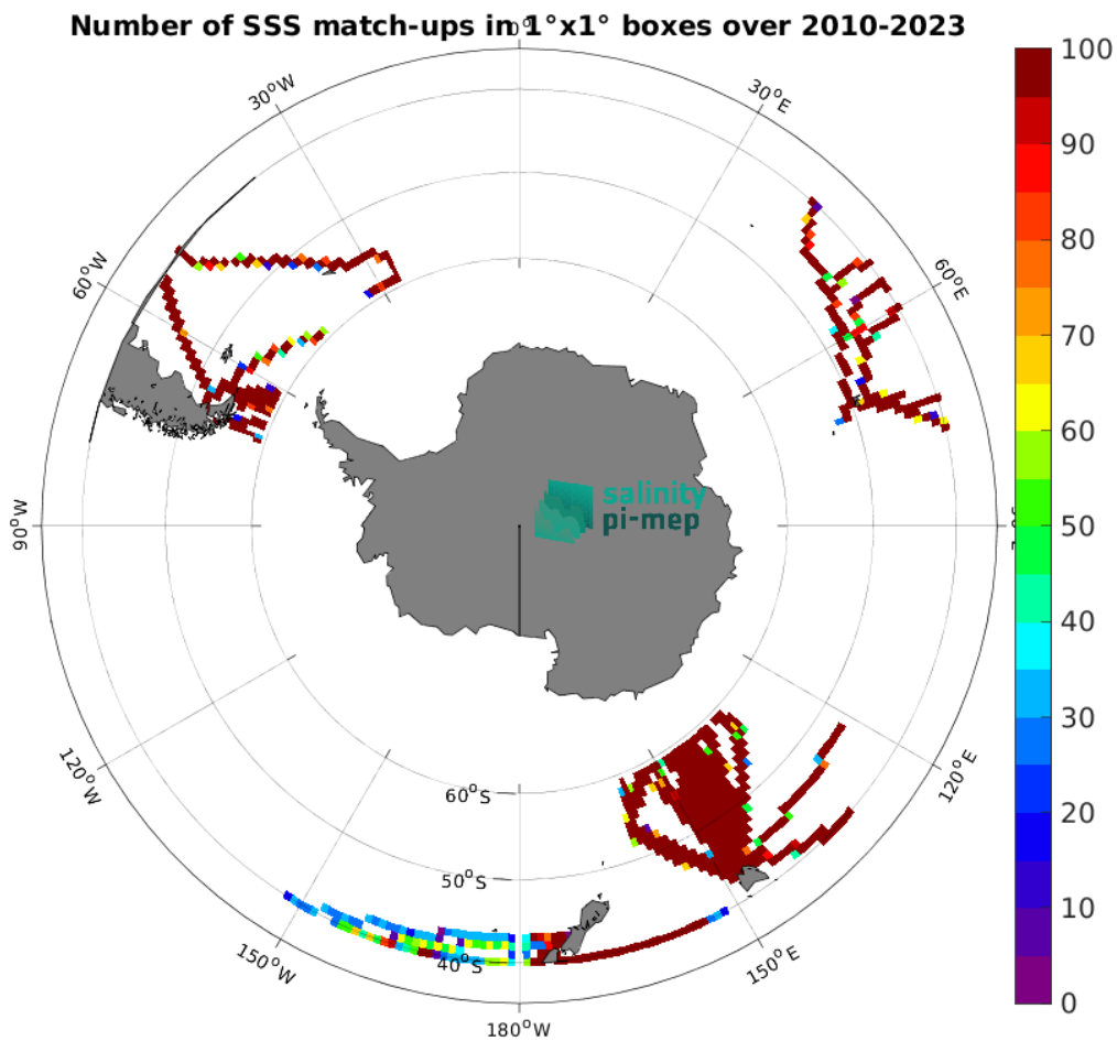
Figure 4: Number of SSS match-ups between TSG (LEGOS-DM) SSS and the SMOS SSS L4 v1 - Weekly (CMEMS-CNR) SSS product for the Roaring Forties and Furious Fifties Pi-MEP region over 1^\circ \times 1^\circ boxes and for the full satellite product period.
