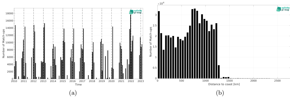
Figure 1: Number of match-ups between TSG (LEGOS-DM) and SMOS SSS L4 v1 - Weekly (CMEMS-CNR) SSS as a function of time (a) and as function of the distance to coast (b) over the Roaring Forties and Furious Fifties Pi-MEP region and for the full satellite product period.
