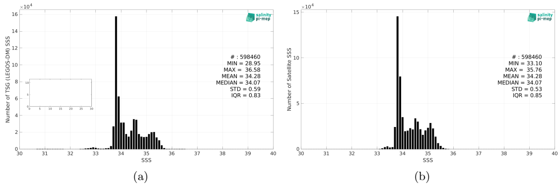
Figure 2: Histograms of SSS from TSG (LEGOS-DM) (a) and SMOS SSS L4 v1 - Weekly (CMEMS-CNR) (b) considering all match-up pairs per bins of 0.1 over the Roaring Forties and Furious Fifties Pi-MEP region and for the full satellite product period.
