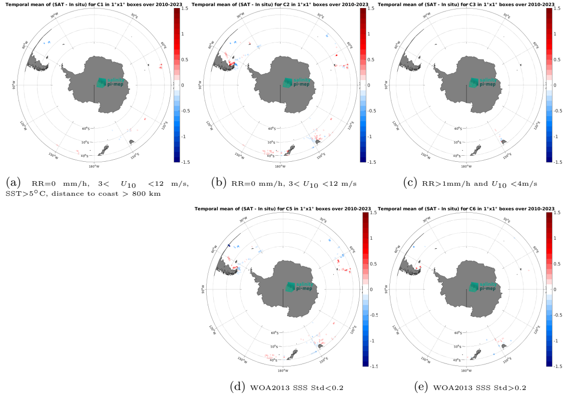
Figure 12: Temporal mean gridded over spatial boxes of size 1^{\circ}\times 1^{\circ} of \Delta\text{SSS} (SMOS SSS L4 v1 - Weekly (CMEMS-CNR) - TSG (LEGOS-DM)) for 5 different subdatasets corresponding to:RR=0 mm/h, 3 < U_{10} < 12 m/s, SST >5^{\circ}\text{C} , distance to coast > 800 km (a), RR=0 mm/h, 3 < U_{10} < 12 m/s (b), RR >1 mm/h and U_{10} < 4 m/s (c), WOA2013 SSS Std <0.2 (d), WOA2013 SSS Std >0.2 (e).
