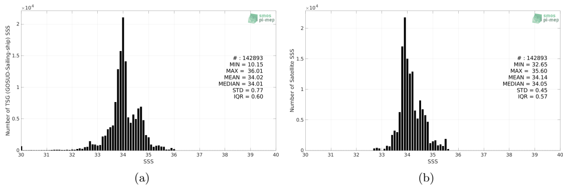
Figure 2: Histograms of SSS from TSG (GOSUD-Sailing-ship) (a) and SMOS SSS L4 v1 - Weekly (CMEMS-CNR) (b) considering all match-up pairs per bins of 0.1 over the Roaring Forties and Furious Fifties Pi-MEP region and for the full satellite product period.
