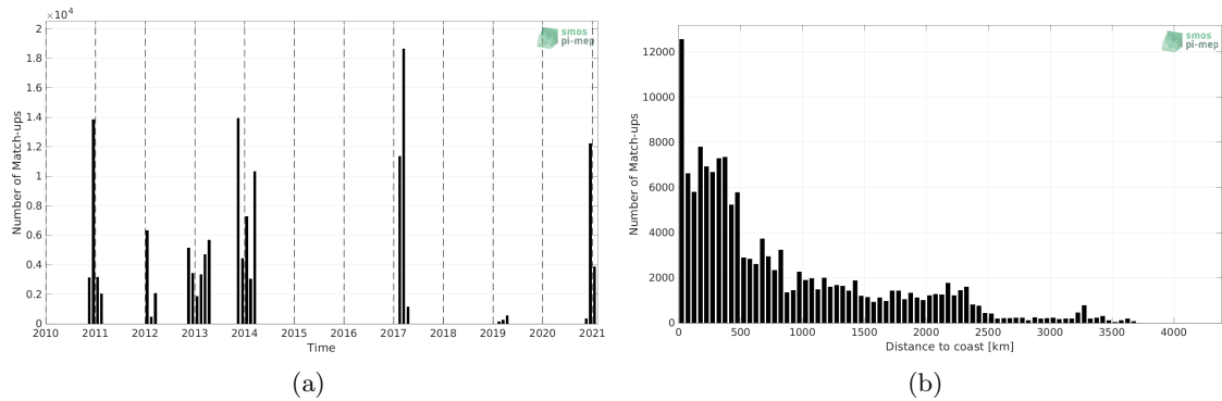
Figure 1: Number of match-ups between TSG (GOSUD-Sailing-ship) and SMOS SSS L4 v1 - Weekly (CMEMS-CNR) SSS as a function of time (a) and as function of the distance to coast (b) over the Roaring Forties and Furious Fifties Pi-MEP region and for the full satellite product period.
