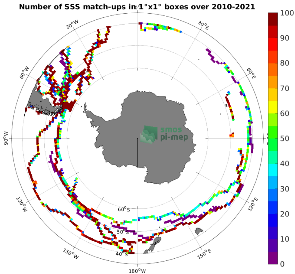
Figure 4: Number of SSS match-ups between TSG (GOSUD-Sailing-ship) SSS and the SMOS SSS L4 v1 - Weekly (CMEMS-CNR) SSS product for the Roaring Forties and Furious Fifties Pi-MEP region over 1^\circ \times 1^\circ boxes and for the full satellite product period.
