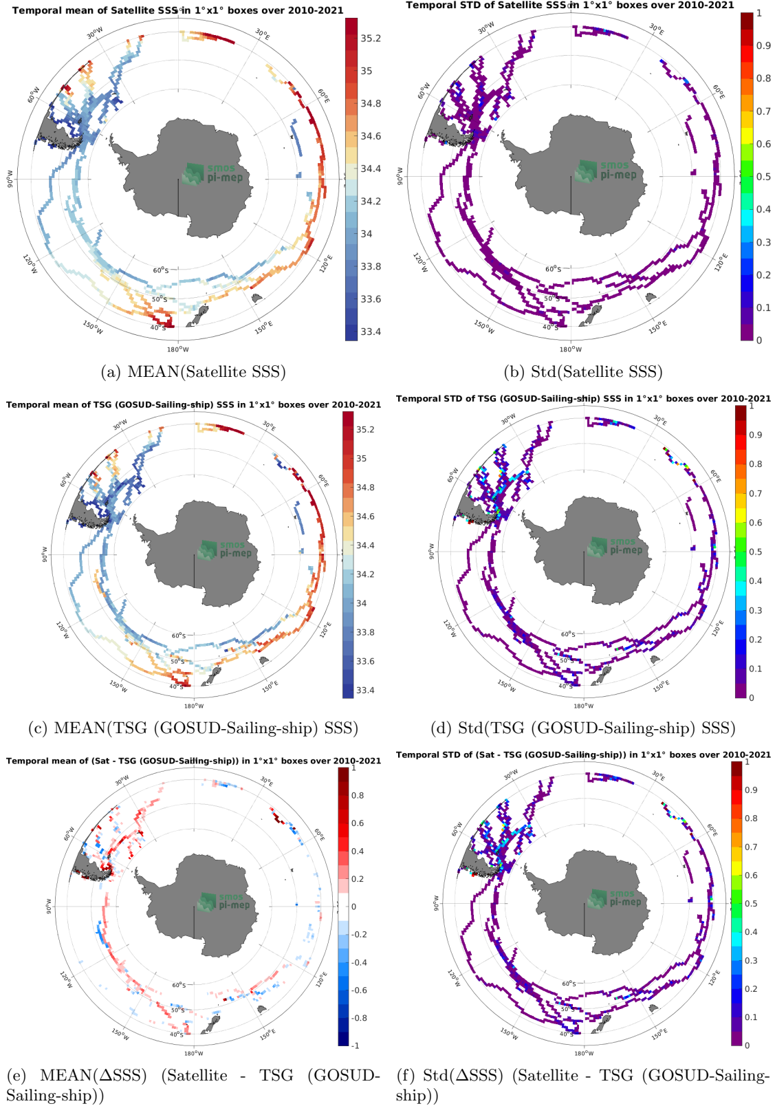
Figure 6: Temporal mean (left) and Std (right) of SSS from SMOS SSS L4 v1 - Weekly (CMEMS-CNR) (top), TSG (GOSUD-Sailing-ship) (middle), and of \Delta SSS (Satellite - TSG (GOSUD-Sailing-ship)). Only match-up pairs are used to generate these maps.
