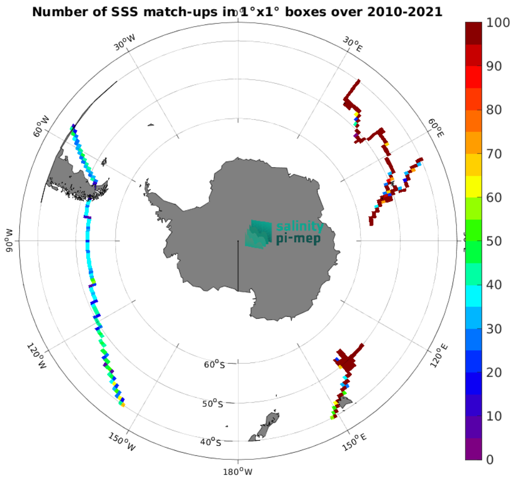
Figure 4: Number of SSS match-ups between TSG (GOSUD-Research-vessel) SSS and the SMOS SSS L4 v1 - Weekly (CMEMS-CNR) SSS product for the Roaring Forties and Furious Fifties Pi-MEP region over 1^\circ \times 1^\circ boxes and for the full satellite product period.
