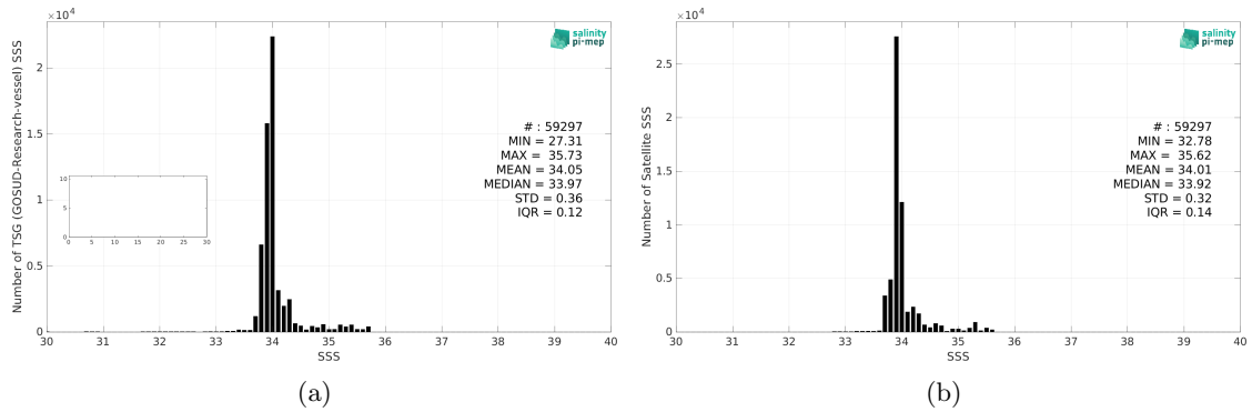
Figure 2: Histograms of SSS from TSG (GOSUD-Research-vessel) (a) and SMOS SSS L4 v1 - Weekly (CMEMS-CNR) (b) considering all match-up pairs per bins of 0.1 over the Roaring Forties and Furious Fifties Pi-MEP region and for the full satellite product period.
