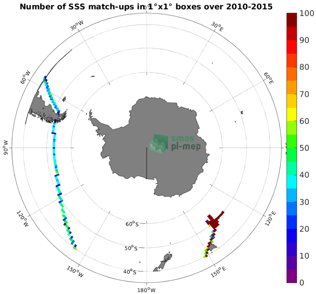
Figure 4: Number of SSS match-ups between TSG (GOSUD-Research-vessel) SSS and the SMOS SSS L4 v1 - Weekly (CMEMS-CNR) SSS product for the Roaring Forties and Furious Fifties Pi-MEP region over 1^{\circ} \times 1^{\circ} boxes and for the full satellite product period.
