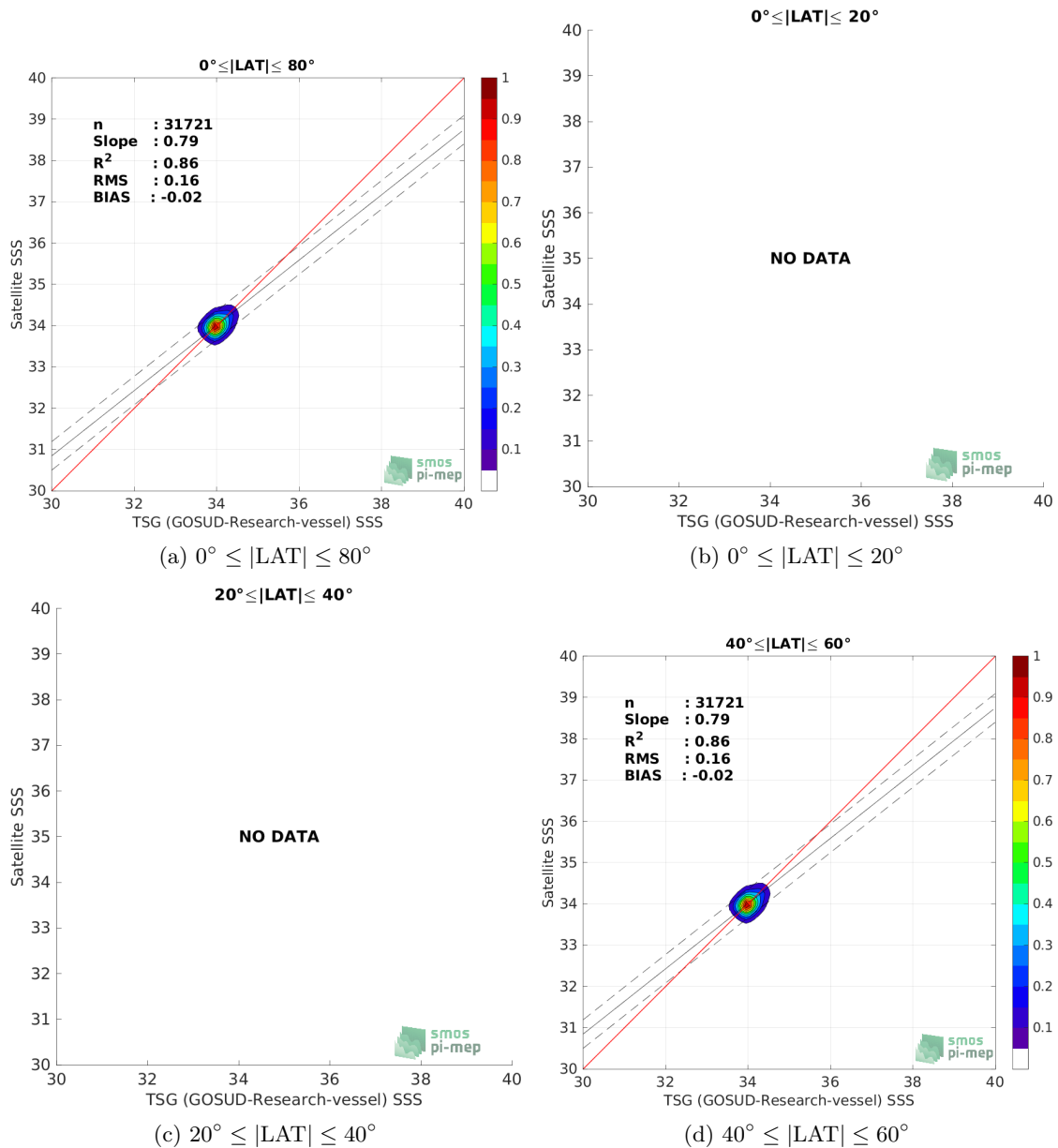
Figure 9: Contour maps of the concentration of SMOS SSS L4 v1 - Weekly (CMEMS-CNR) SSS (y-axis) versus TSG (GOSUD-Research-vessel) SSS (x-axis) at match-up pairs for different latitude bands. For each plot, the red line shows x=y . The black thin and dashed lines indicate a linear fit through the data cloud and the \pm 95\% confidence levels, respectively. The number match-up pairs n , the slope and R^2 coefficient of the linear fit, the root mean square (RMS) and the mean bias between satellite and in situ data are indicated for each latitude band in each plots.
