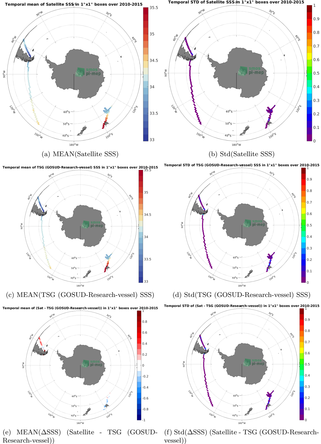
Figure 6: Temporal mean (left) and Std (right) of SSS from SMOS SSS L4 v1 - Weekly (CMEMS-CNR) (top), TSG (GOSUD-Research-vessel) (middle), and of \Delta SSS (Satellite - TSG (GOSUD-Research-vessel)). Only match-up pairs are used to generate these maps.
