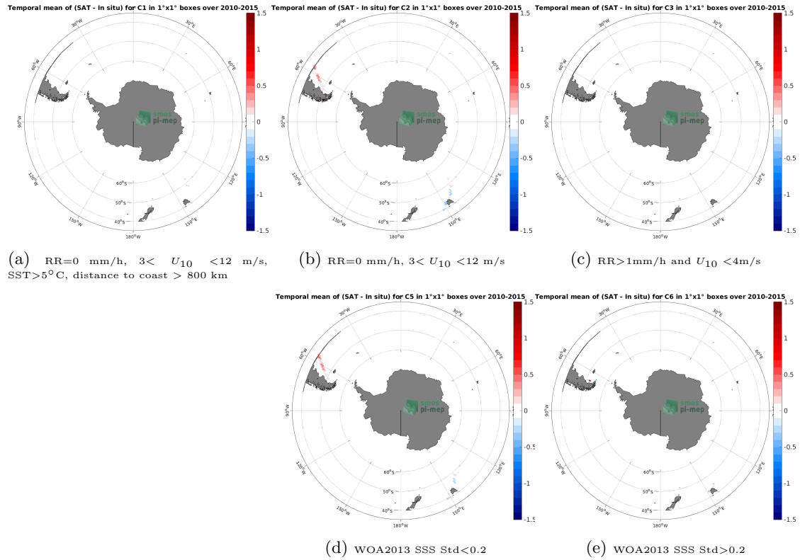
Figure 12: Temporal mean gridded over spatial boxes of size 1^\circ \times 1^\circ of \Delta\text{SSS} (SMOS SSS L4 v1 - Weekly (CMEMS-CNR) - TSG (GOSUD-Research-vessel)) for 5 different subdatasets corresponding to: RR=0 mm/h, 3 < U_{10} < 12 m/s, SST > 5^\circ\text{C} , distance to coast > 800 km (a), RR=0 mm/h, 3 < U_{10} < 12 m/s (b), RR > 1 mm/h and U_{10} < 4 m/s (c), WOA2013 SSS Std <0.2 (d), WOA2013 SSS Std >0.2 (e).
