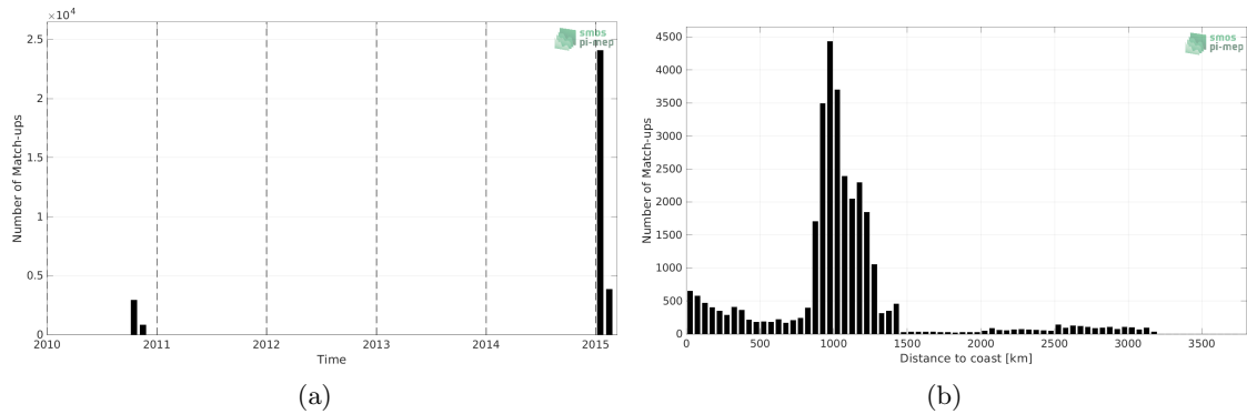
Figure 1: Number of match-ups between TSG (GOSUD-Research-vessel) and SMOS SSS L4 v1 - Weekly (CMEMS-CNR) SSS as a function of time (a) and as function of the distance to coast (b) over the Roaring Forties and Furious Fifties Pi-MEP region and for the full satellite product period.
