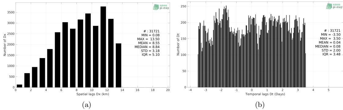
Figure 5: Histograms of the spatial (a) and temporal (b) lags between the location/time of the TSG (GOSUD-Research-vessel) measurement and the date of the corresponding SMOS SSS L4 v1 - Weekly (CMEMS-CNR) SSS pixel.
