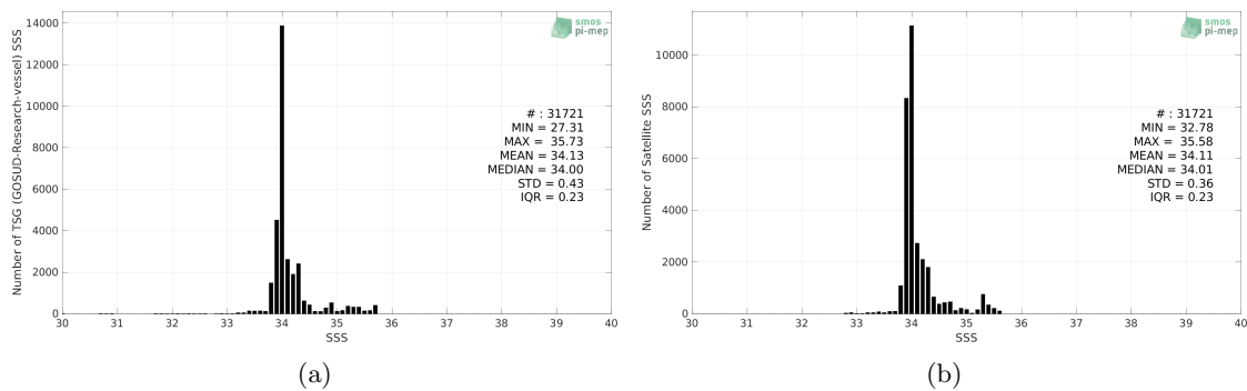
Figure 2: Histograms of SSS from TSG (GOSUD-Research-vessel) (a) and SMOS SSS L4 v1 - Weekly (CMEMS-CNR) (b) considering all match-up pairs per bins of 0.1 over the Roaring Forties and Furious Fifties Pi-MEP region and for the full satellite product period.
