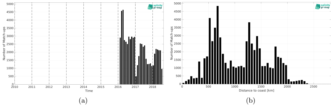
Figure 1: Number of match-ups between Surface drifters and SMOS SSS L4 v1 - Weekly (CMEMS-CNR) SSS as a function of time (a) and as function of the distance to coast (b) over the Roaring Forties and Furious Fifties Pi-MEP region and for the full satellite product period.
