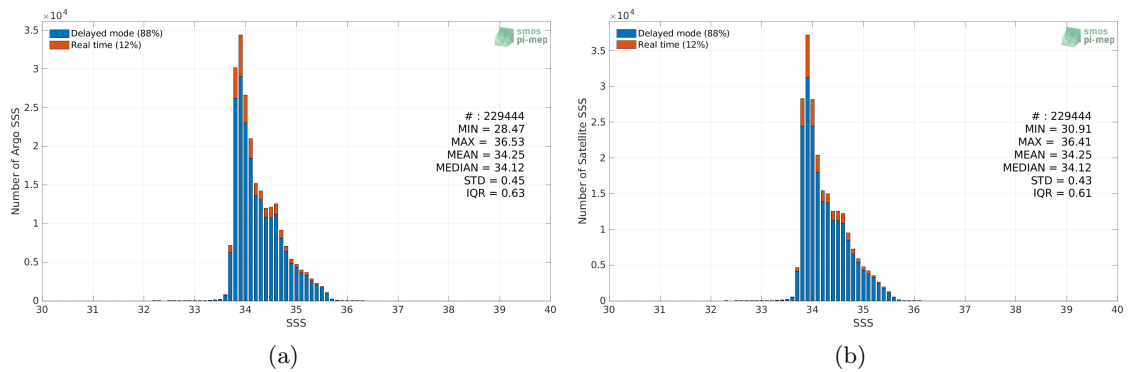
Figure 2: Histograms of SSS from Argo (a) and SMOS SSS L4 v1 - Weekly (CMEMS-CNR) (b) considering all match-up pairs per bins of 0.1 over the Roaring Forties and Furious Fifties Pi-MEP region and for the full satellite product period.
