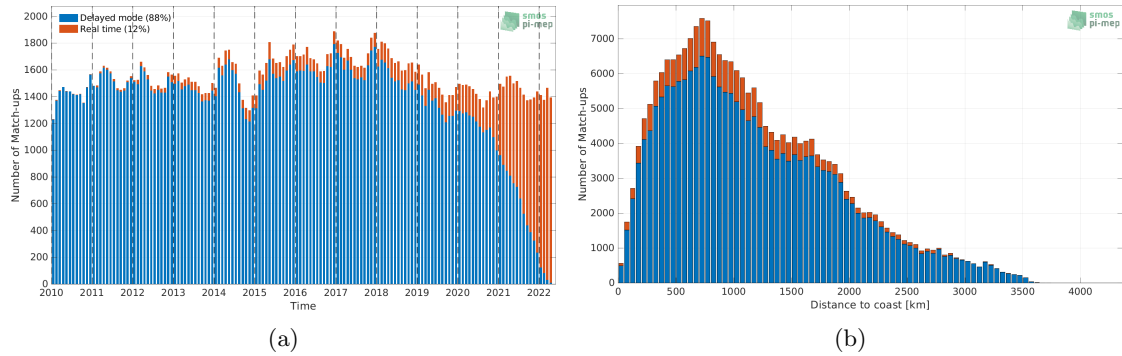
Figure 1: Number of match-ups between Argo and SMOS SSS L4 v1 - Weekly (CMEMS-CNR) SSS as a function of time (a) and as function of the distance to coast (b) over the Roaring Forties and Furious Fifties Pi-MEP region and for the full satellite product period.
