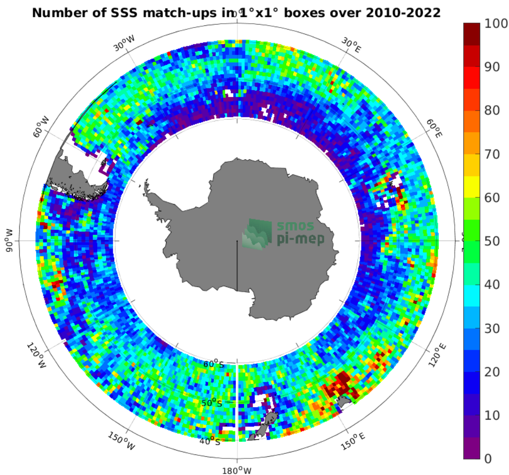
Figure 4: Number of SSS match-ups between Argo SSS and the SMOS SSS L4 v1 - Weekly (CMEMS-CNR) SSS product for the Roaring Forties and Furious Fifties Pi-MEP region over 1^\circ \times 1^\circ boxes and for the full satellite product period.
