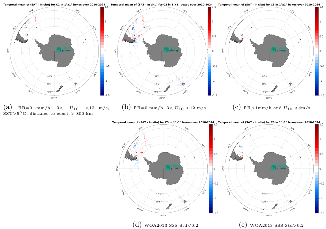
Figure 14: Temporal mean gridded over spatial boxes of size 1^\circ \times 1^\circ of \Delta SSS (SMOS SSS L4 v1 - Monthly (CMEMS-CNR) - TSG (SAMOS)) for 5 different subdatasets corresponding to:RR=0 mm/h, 3 < U_{10} < 12 m/s, SST>5°C, distance to coast > 800 km (a), RR=0 mm/h, 3 < U_{10} < 12 m/s (b), RR>1mm/h and U_{10} < 4 m/s (c), WOA2013 SSS Std<0.2 (d), WOA2013 SSS Std>0.2 (e).
