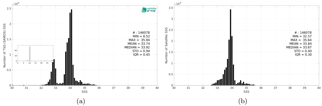
Figure 3: Histograms of SSS from TSG (SAMOS) (a) and SMOS SSS L4 v1 - Monthly (CMEMS-CNR) (b) considering all match-up pairs per bins of 0.1 over the Roaring Forties and Furious Fifties Pi-MEP region and for the full satellite product period.
