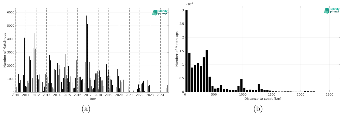
Figure 2: Number of match-ups between TSG (SAMOS) and SMOS SSS L4 v1 - Monthly (CMEMS-CNR) SSS as a function of time (a) and as function of the distance to coast (b) over the Roaring Forties and Furious Fifties Pi-MEP region and for the full satellite product period.
