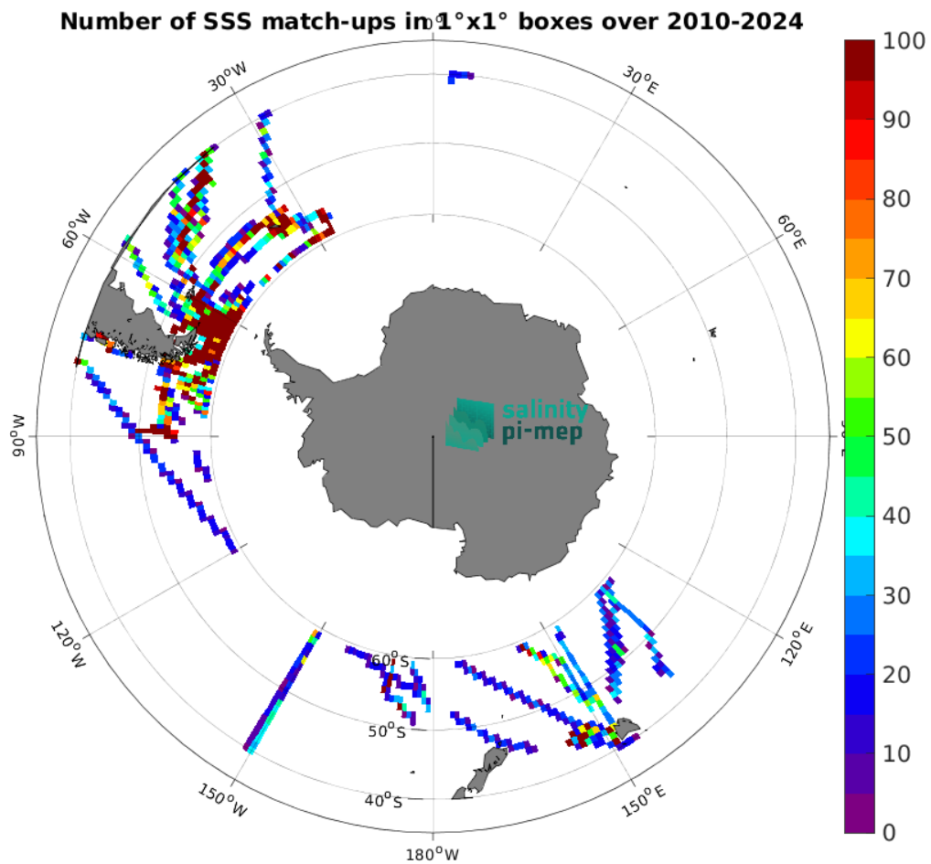
Figure 5: Number of SSS match-ups between TSG (SAMOS) SSS and the SMOS SSS L4 v1 - Monthly (CMEMS-CNR) SSS product for the Roaring Forties and Furious Fifties Pi-MEP region over 1^\circ \times 1^\circ boxes and for the full satellite product period.
