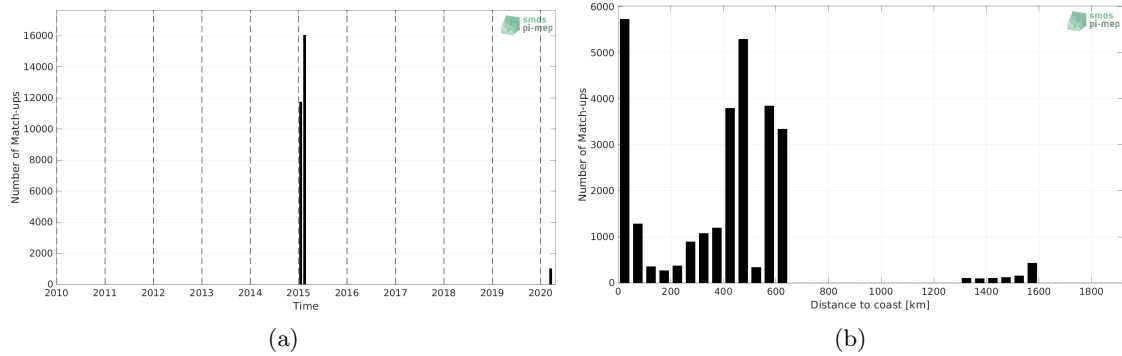
Figure 1: Number of match-ups between TSG (SAMOS) and SMOS SSS L4 v1 - Monthly (CMEMS-CNR) SSS as a function of time (a) and as function of the distance to coast (b) over the Roaring Forties and Furious Fifties Pi-MEP region and for the full satellite product period.
