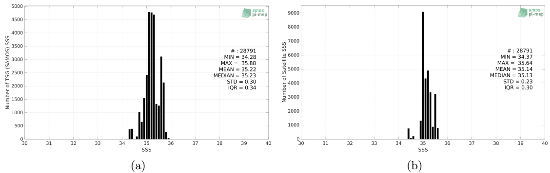
Figure 2: Histograms of SSS from TSG (SAMOS) (a) and SMOS SSS L4 v1 - Monthly (CMEMS-CNR) (b) considering all match-up pairs per bins of 0.1 over the Roaring Forties and Furious Fifties Pi-MEP region and for the full satellite product period.
