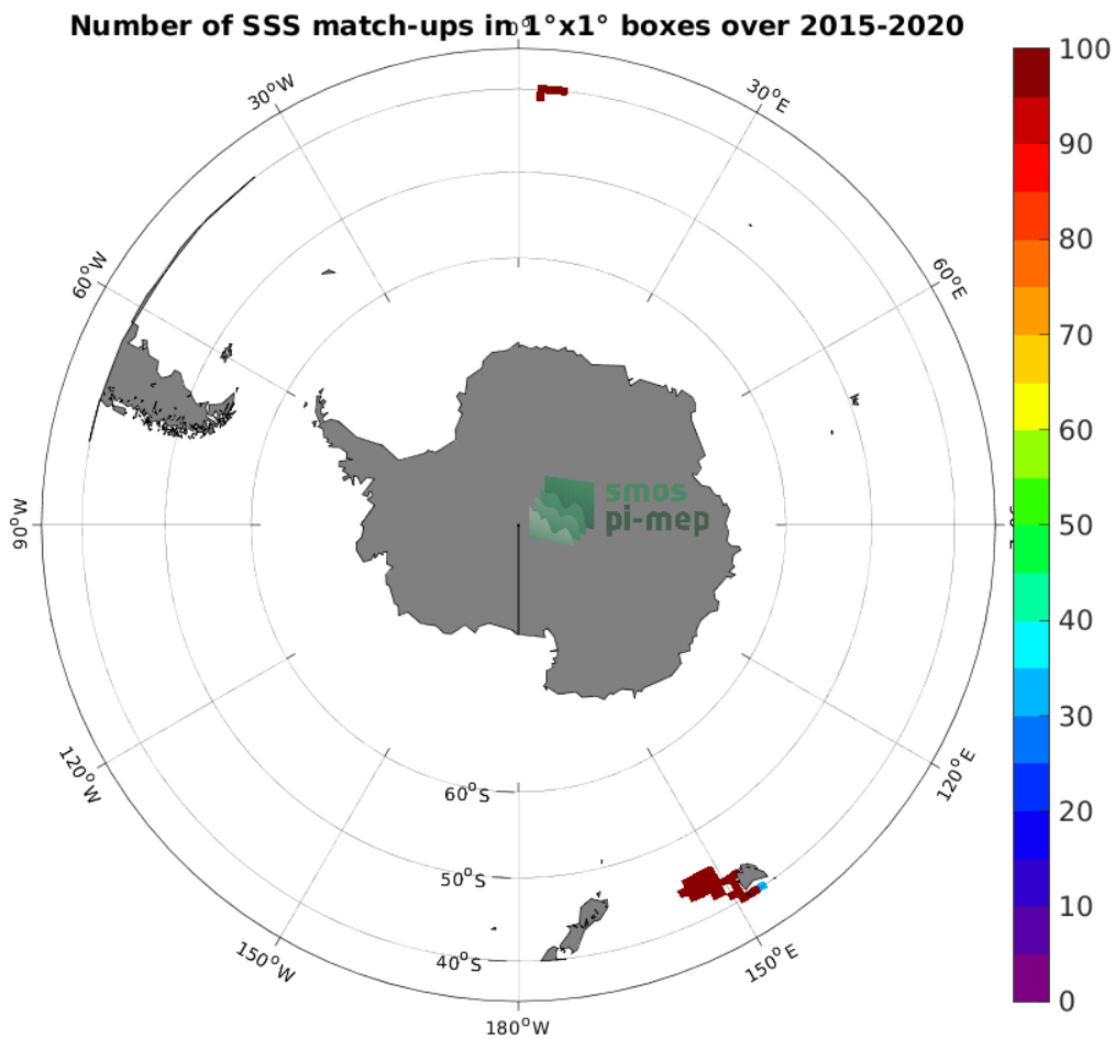
Figure 4: Number of SSS match-ups between TSG (SAMOS) SSS and the SMOS SSS L4 v1 - Monthly (CMEMS-CNR) SSS product for the Roaring Forties and Furious Fifties Pi-MEP region over 1^\circ \times 1^\circ boxes and for the full satellite product period.
