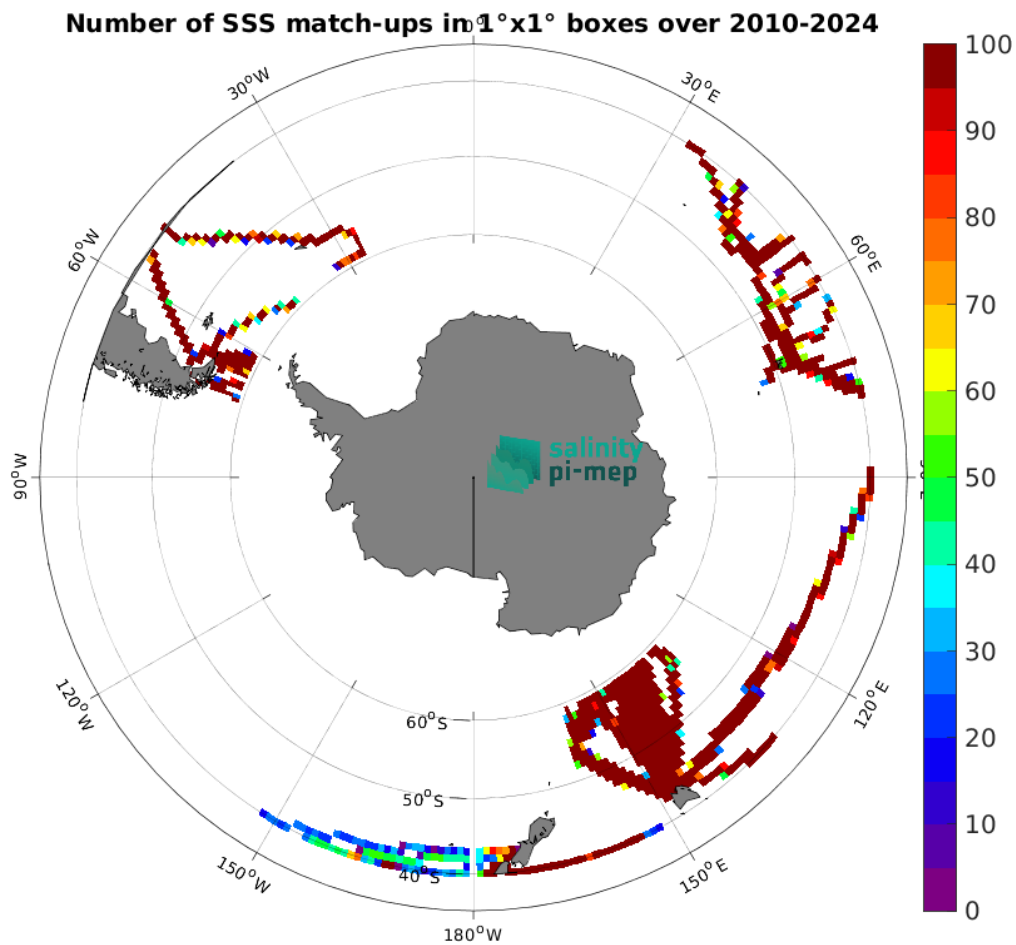
Figure 5: Number of SSS match-ups between TSG (LEGOS-DM) SSS and the SMOS SSS L4 v1 - Monthly (CMEMS-CNR) SSS product for the Roaring Forties and Furious Fifties Pi-MEP region over 1^\circ \times 1^\circ boxes and for the full satellite product period.
