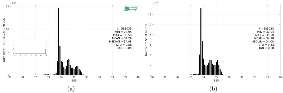
Figure 3: Histograms of SSS from TSG (LEGOS-DM) (a) and SMOS SSS L4 v1 - Monthly (CMEMS-CNR) (b) considering all match-up pairs per bins of 0.1 over the Roaring Forties and Furious Fifties Pi-MEP region and for the full satellite product period.
