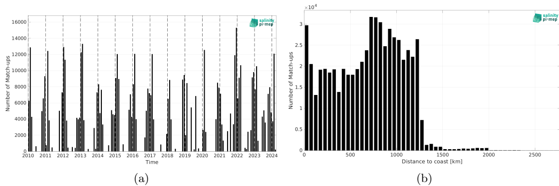
Figure 2: Number of match-ups between TSG (LEGOS-DM) and SMOS SSS L4 v1 - Monthly (CMEMS-CNR) SSS as a function of time (a) and as function of the distance to coast (b) over the Roaring Forties and Furious Fifties Pi-MEP region and for the full satellite product period.
