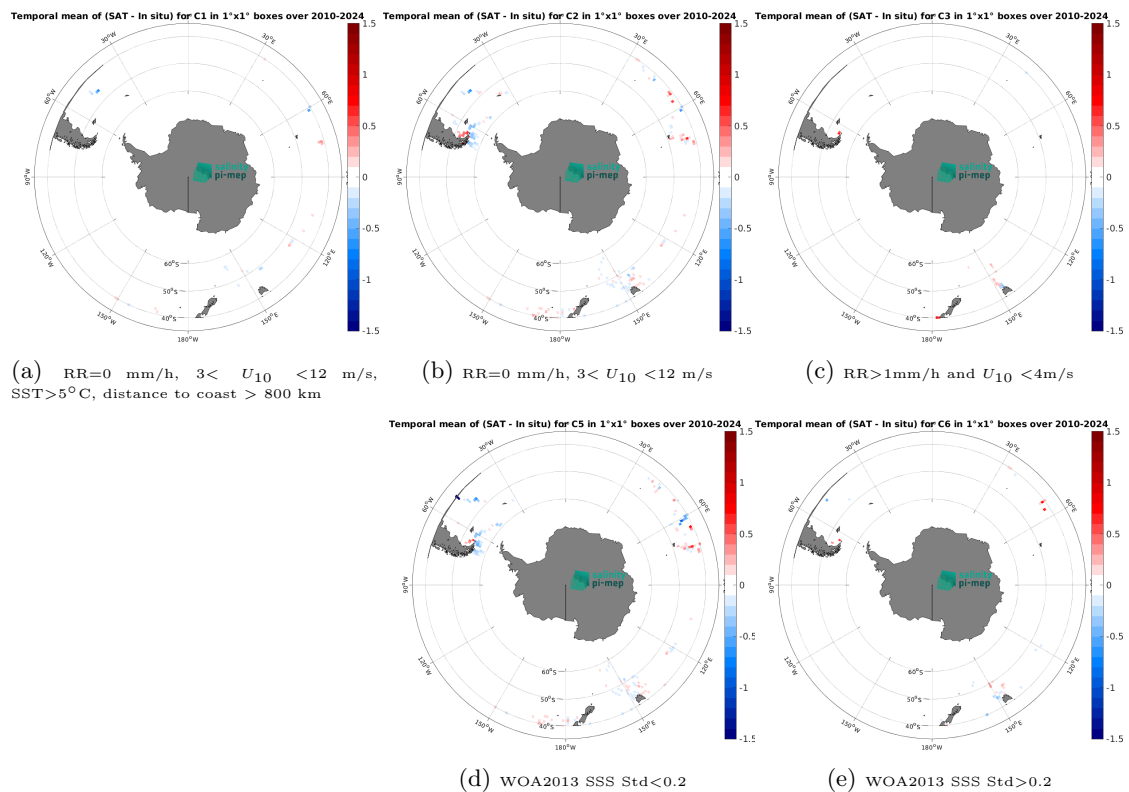
Figure 14: Temporal mean gridded over spatial boxes of size 1^\circ \times 1^\circ of \Delta SSS (SMOS SSS L4 v1 - Monthly (CMEMS-CNR) - TSG (LEGOS-DM)) for 5 different subdatasets corresponding to: RR=0 mm/h, 3 < U_{10} < 12 m/s, SST > 5^\circ\text{C} , distance to coast > 800 km (a), RR=0 mm/h, 3 < U_{10} < 12 m/s (b), RR > 1 mm/h and U_{10} < 4 m/s (c), WOA2013 SSS Std < 0.2 (d), WOA2013 SSS Std > 0.2 (e).
