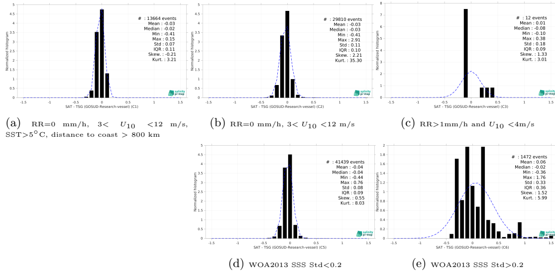
Figure 15: Normalized histogram of \Delta\text{SSS} (SMOS SSS L4 v1 - Monthly (CMEMS-CNR) - TSG (GOSUD-Research-vessel)) for 5 different subdatasets corresponding to: RR=0 mm/h, 3 < U_{10} < 12 m/s, SST > 5^\circ\text{C} , distance to coast > 800 km (a), RR=0 mm/h, 3 < U_{10} < 12 m/s (b), RR > 1\text{mm/h} and U_{10} < 4\text{m/s} (c), WOA2013 SSS Std < 0.2 (d), WOA2013 SSS Std > 0.2 (e).
