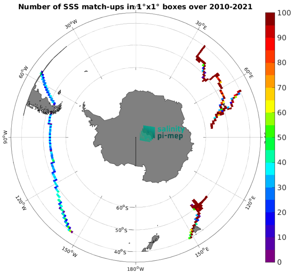
Figure 5: Number of SSS match-ups between TSG (GOSUD-Research-vessel) SSS and the SMOS SSS L4 v1 - Monthly (CMEMS-CNR) SSS product for the Roaring Forties and Furious Fifties Pi-MEP region over 1^\circ \times 1^\circ boxes and for the full satellite product period.
