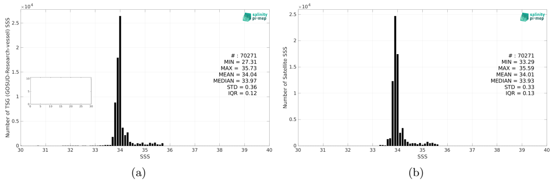
Figure 2: Histograms of SSS from TSG (GOSUD-Research-vessel) (a) and SMOS SSS L4 v1 - Monthly (CMEMS-CNR) (b) considering all match-up pairs per bins of 0.1 over the Roaring Forties and Furious Fifties Pi-MEP region and for the full satellite product period.
