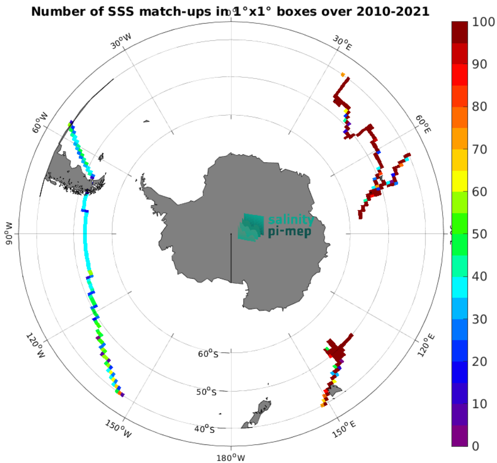
Figure 4: Number of SSS match-ups between TSG (GOSUD-Research-vessel) SSS and the SMOS SSS L4 v1 - Monthly (CMEMS-CNR) SSS product for the Roaring Forties and Furious Fifties Pi-MEP region over 1^{\circ} \times 1^{\circ} boxes and for the full satellite product period.
