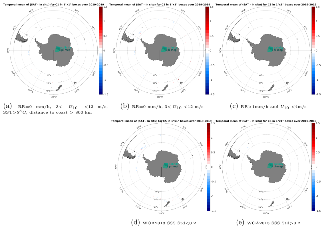
Figure 14: Temporal mean gridded over spatial boxes of size 1^\circ \times 1^\circ of \Delta\text{SSS} (SMOS SSS L4 v1 - Monthly (CMEMS-CNR) - Saildrone) for 5 different subdatasets corresponding to:RR=0 mm/h, 3 < U_{10} < 12 m/s, SST>5°C, distance to coast > 800 km (a), RR=0 mm/h, 3 < U_{10} < 12 m/s (b), RR>1mm/h and U_{10} < 4 m/s (c), WOA2013 SSS Std<0.2 (d), WOA2013 SSS Std>0.2 (e).
