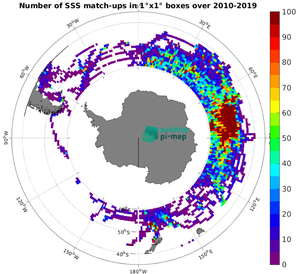
Figure 4: Number of SSS match-ups between Marine mammals SSS and the SMOS SSS L4 v1 - Monthly (CMEMS-CNR) SSS product for the Roaring Forties and Furious Fifties Pi-MEP region over 1^\circ \times 1^\circ boxes and for the full satellite product period.
