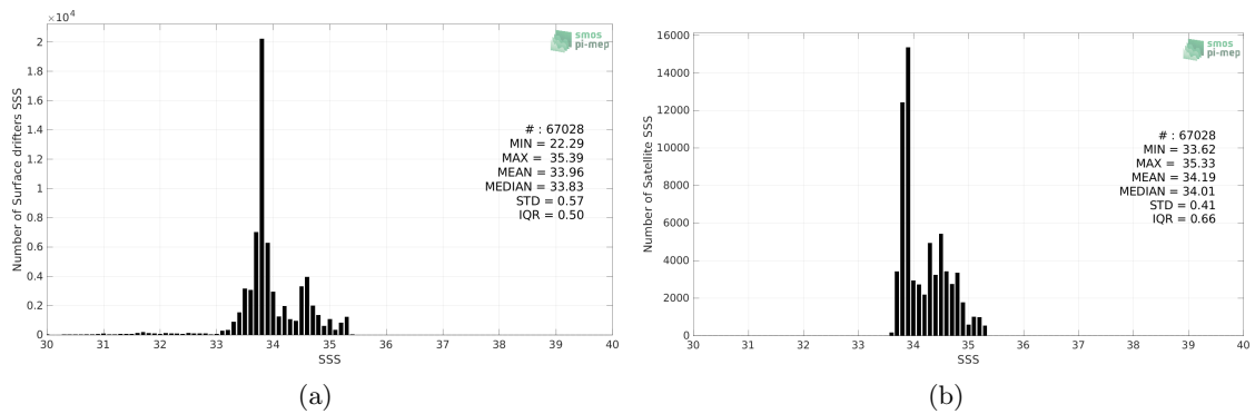
Figure 2: Histograms of SSS from Surface drifters (a) and SMOS SSS L4 v1 - Monthly (CMEMS-CNR) (b) considering all match-up pairs per bins of 0.1 over the Roaring Forties and Furious Fifties Pi-MEP region and for the full satellite product period.
