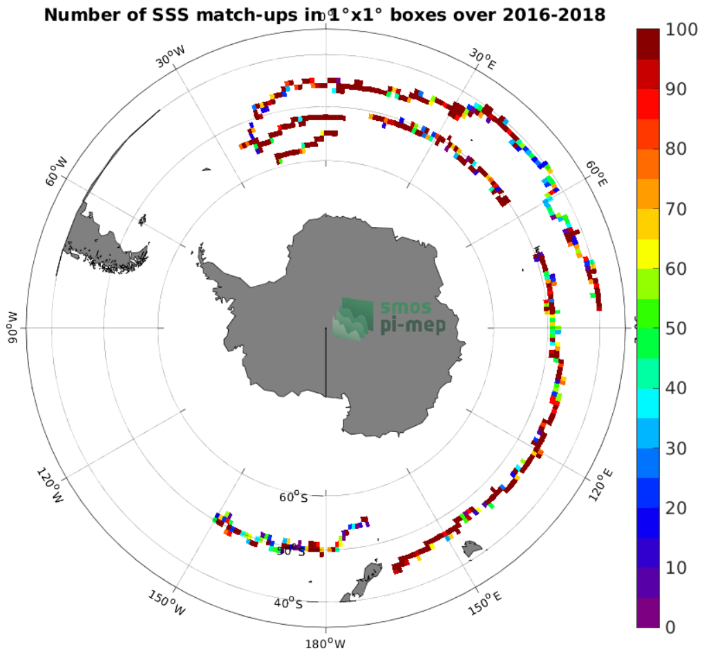
Figure 3: Number of SSS match-ups between Surface drifters SSS and the SMOS SSS L4 v1 - Monthly (CMEMS-CNR) SSS product for the Roaring Forties and Furious Fifties Pi-MEP region over 1^\circ \times 1^\circ boxes and for the full satellite product period.
