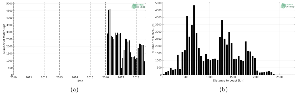
Figure 1: Number of match-ups between Surface drifters and SMOS SSS L4 v1 - Monthly (CMEMS-CNR) SSS as a function of time (a) and as function of the distance to coast (b) over the Roaring Forties and Furious Fifties Pi-MEP region and for the full satellite product period.
