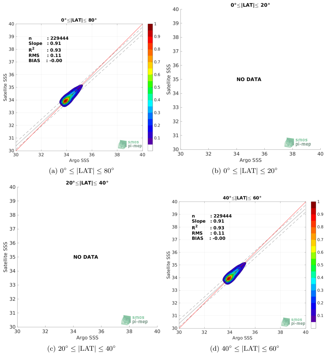
Figure 9: Contour maps of the concentration of SMOS SSS L4 v1 - Monthly (CMEMS-CNR) SSS (y-axis) versus Argo SSS (x-axis) at match-up pairs for different latitude bands. For each plot, the red line shows x=y . The black thin and dashed lines indicate a linear fit through the data cloud and the \pm 95\% confidence levels, respectively. The number match-up pairs n , the slope and R^2 coefficient of the linear fit, the root mean square (RMS) and the mean bias between satellite and in situ data are indicated for each latitude band in each plots.
