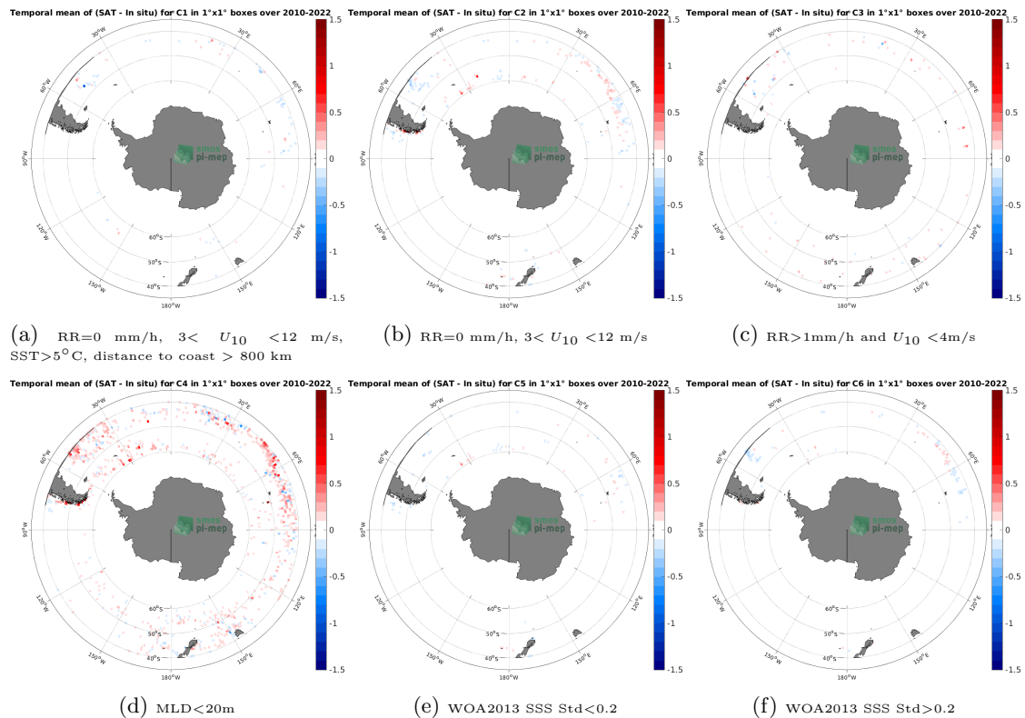
Figure 12: Temporal mean gridded over spatial boxes of size 1^{\circ}\times 1^{\circ} of \Delta\text{SSS} (SMOS SSS L4 v1 - Monthly (CMEMS-CNR) - Argo) for 6 different subdatasets corresponding to:RR=0 mm/h, 3 < U_{10} < 12 m/s, SST > 5^{\circ}\text{C} , distance to coast > 800 km (a), RR=0 mm/h, 3 < U_{10} < 12 m/s (b), RR > 1\text{mm/h} and U_{10} < 4\text{m/s} (c),MLD < 20\text{m} (d),WOA2013 SSS Std < 0.2 (e),WOA2013 SSS Std > 0.2 (f).
