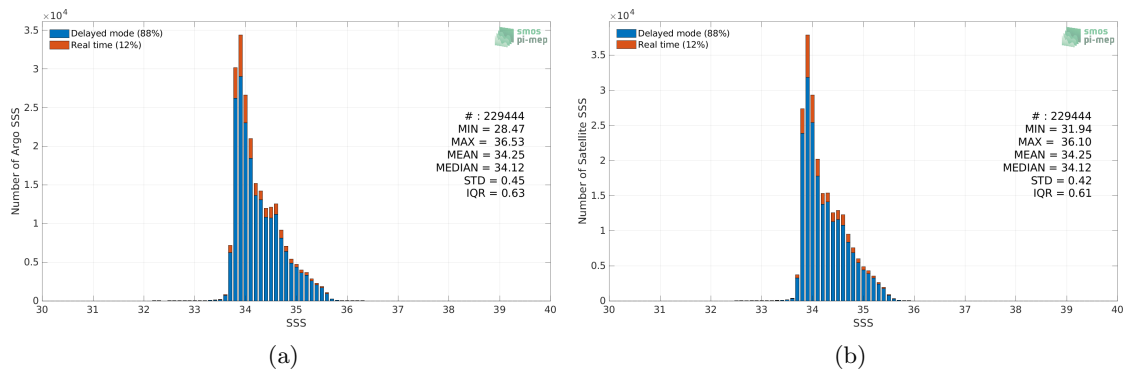
Figure 2: Histograms of SSS from Argo (a) and SMOS SSS L4 v1 - Monthly (CMEMS-CNR) (b) considering all match-up pairs per bins of 0.1 over the Roaring Forties and Furious Fifties Pi-MEP region and for the full satellite product period.
