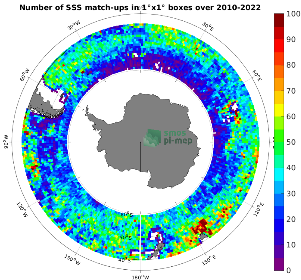
Figure 4: Number of SSS match-ups between Argo SSS and the SMOS SSS L4 v1 - Monthly (CMEMS-CNR) SSS product for the Roaring Forties and Furious Fifties Pi-MEP region over 1^\circ \times 1^\circ boxes and for the full satellite product period.
