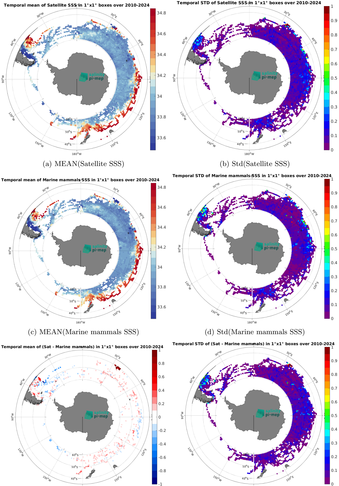
Figure 7: Temporal mean (left) and Std (right) of SSS from SMOS SSS L4 v1 - Daily (CMEMS-CNR) (top), Marine mammals (middle), and of \Delta SSS (Satellite - Marine mammals). Only match-up pairs are used to generate these maps.
