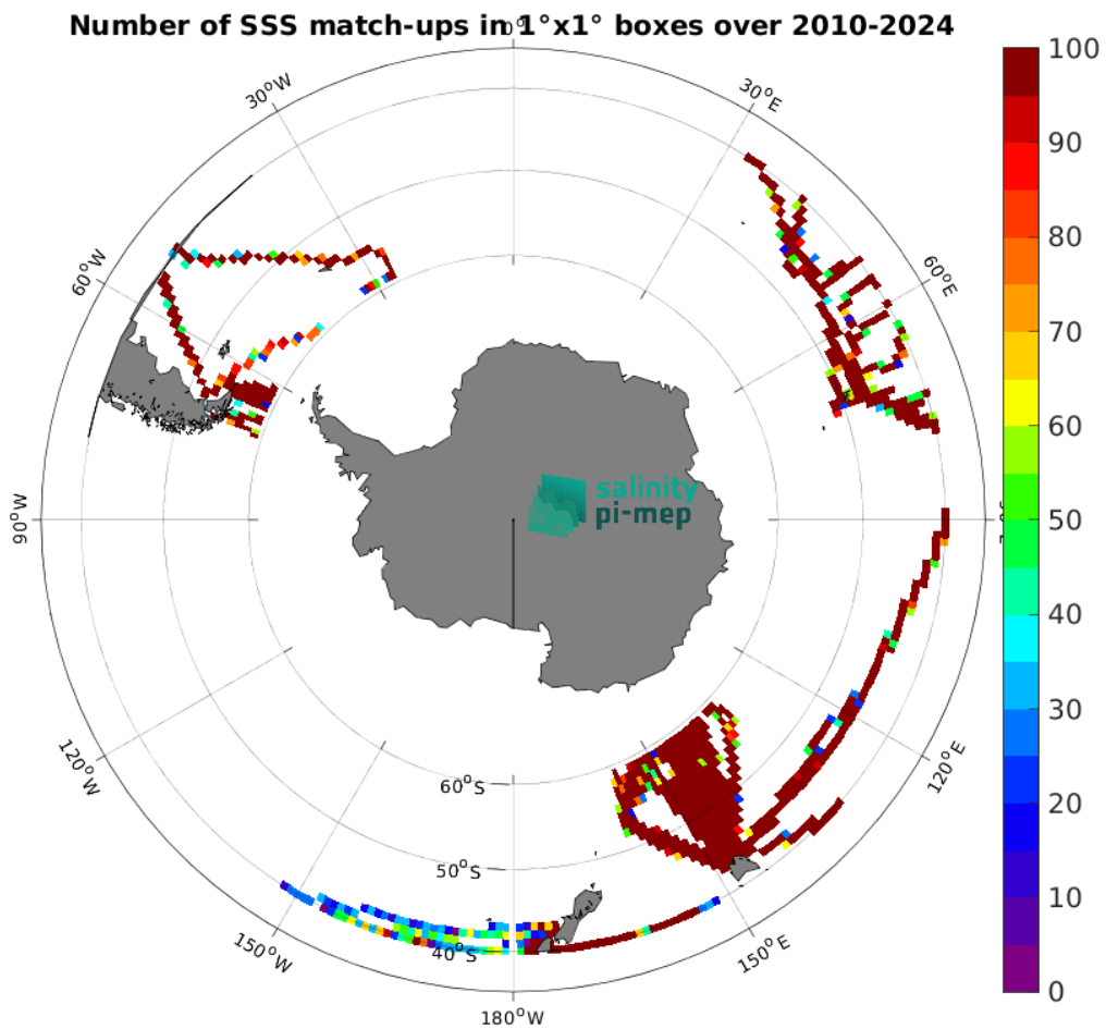
Figure 5: Number of SSS match-ups between TSG (LEGOS-DM) SSS and the SMOS SSS L4 OI v346 - Weekly (CMEMS-CATDS-LOPS) SSS product for the Roaring Forties and Furious Fifties Pi-MEP region over 1^\circ \times 1^\circ boxes and for the full satellite product period.
