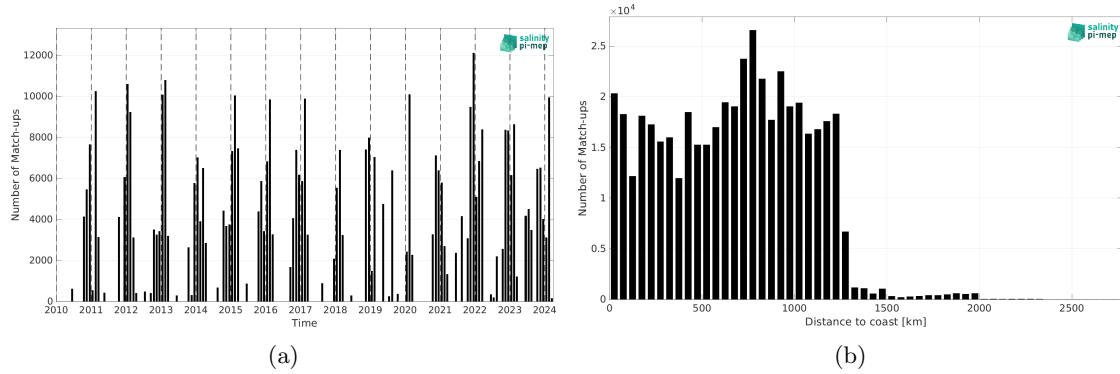
Figure 2: Number of match-ups between TSG (LEGOS-DM) and SMOS SSS L4 OI v346 - Weekly (CMEMS-CATDS-LOPS) SSS as a function of time (a) and as function of the distance to coast (b) over the Roaring Forties and Furious Fifties Pi-MEP region and for the full satellite product period.
