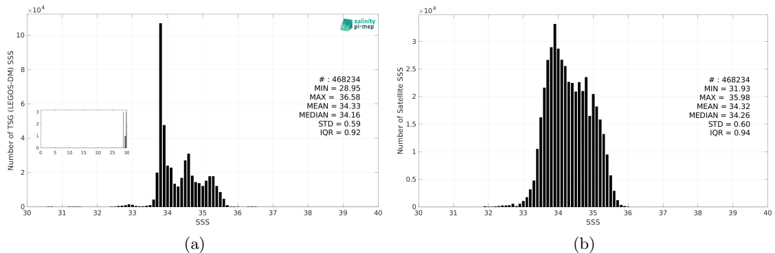
Figure 3: Histograms of SSS from TSG (LEGOS-DM) (a) and SMOS SSS L4 OI v346 - Weekly (CMEMS-CATDS-LOPS) (b) considering all match-up pairs per bins of 0.1 over the Roaring Forties and Furious Fifties Pi-MEP region and for the full satellite product period.
