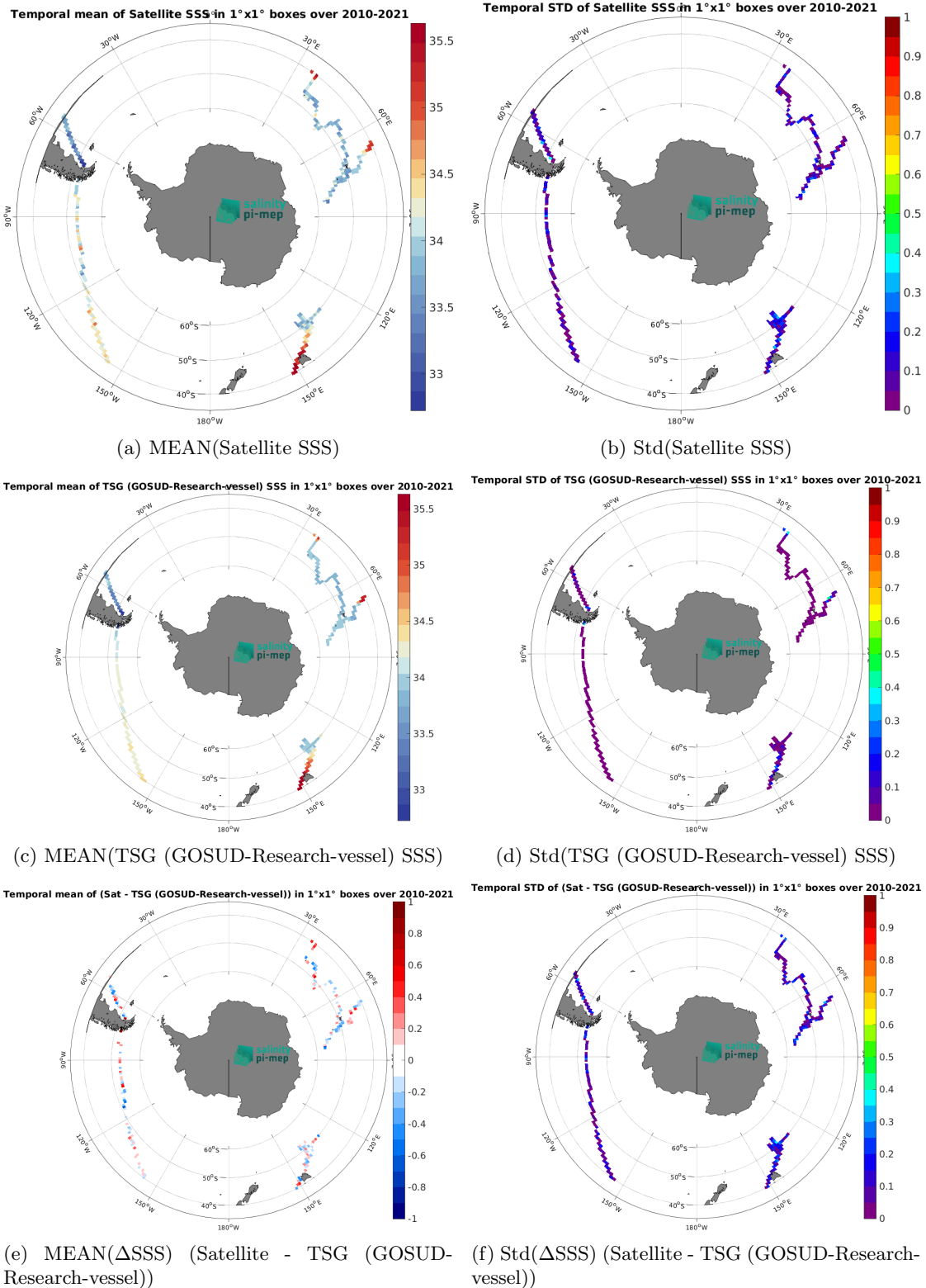
Figure 7: Temporal mean (left) and Std (right) of SSS from SMOS SSS L4 OI v346 - Weekly (CMEMS-CATDS-LOPS) (top), TSG (GOSUD-Research-vessel) (middle), and of \Delta SSS (Satellite - TSG (GOSUD-Research-vessel)). Only matched-up pairs are used to generate these maps.
