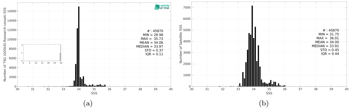
Figure 3: Histograms of SSS from TSG (GOSUD-Research-vessel) (a) and SMOS SSS L4 OI v346 - Weekly (CMEMS-CATDS-LOPS) (b) considering all match-up pairs per bins of 0.1 over the Roaring Forties and Furious Fifties Pi-MEP region and for the full satellite product period.
