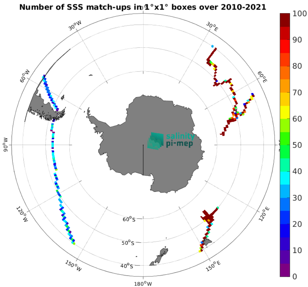
Figure 5: Number of SSS match-ups between TSG (GOSUD-Research-vessel) SSS and the SMOS SSS L4 OI v346 - Weekly (CMEMS-CATDS-LOPS) SSS product for the Roaring Forties and Furious Fifties Pi-MEP region over 1^\circ \times 1^\circ boxes and for the full satellite product period.
