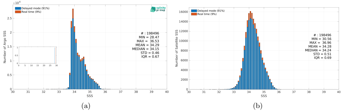
Figure 3: Histograms of SSS from Argo (a) and SMOS SSS L4 OI v346 - Weekly (CMEMS-CATDS-LOPS) (b) considering all match-up pairs per bins of 0.1 over the Roaring Forties and Furious Fifties Pi-MEP region and for the full satellite product period.
