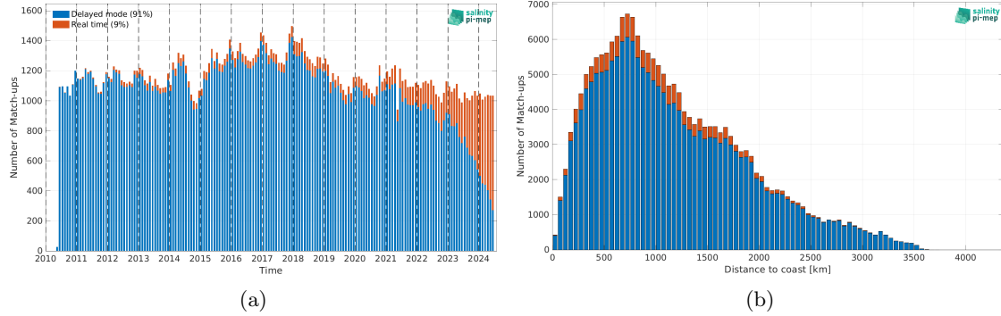
Figure 2: Number of match-ups between Argo and SMOS SSS L4 OI v346 - Weekly (CMEMS-CATDS-LOPS) SSS as a function of time (a) and as function of the distance to coast (b) over the Roaring Forties and Furious Fifties Pi-MEP region and for the full satellite product period.
