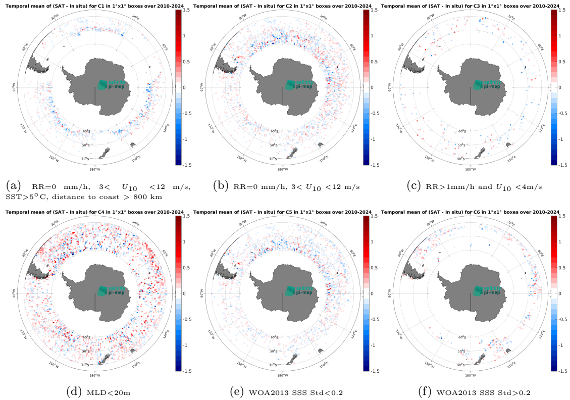
Figure 14: Temporal mean gridded over spatial boxes of size 1^\circ \times 1^\circ of \Delta\text{SSS} (SMOS SSS L4 OI v346 - Weekly (CMEMS-CATDS-LOPS) - Argo) for 6 different subdatasets corresponding to:RR=0 mm/h, 3 < U_{10} < 12 m/s, SST>5°C, distance to coast > 800 km (a), RR=0 mm/h, 3 < U_{10} < 12 m/s (b), RR>1mm/h and U_{10} < 4 m/s (c),MLD<20m (d),WOA2013 SSS Std<0.2 (e),WOA2013 SSS Std>0.2 (f).
