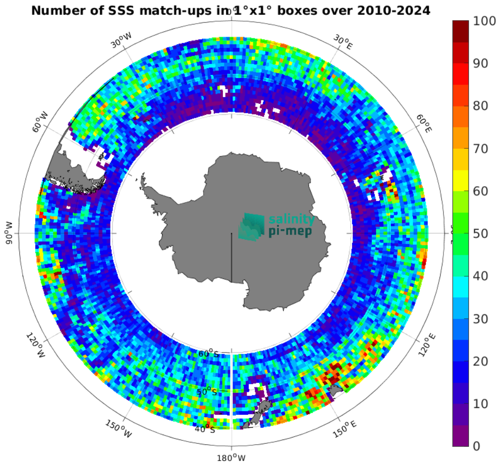
Figure 5: Number of SSS match-ups between Argo SSS and the SMOS SSS L4 OI v346 - Weekly (CMEMS-CATDS-LOPS) SSS product for the Roaring Forties and Furious Fifties Pi-MEP region over 1^\circ \times 1^\circ boxes and for the full satellite product period.
