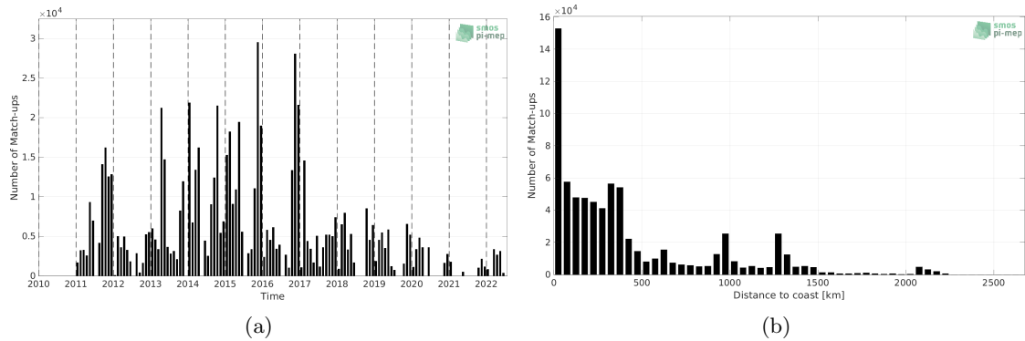
Figure 1: Number of match-ups between TSG (SAMOS) and SMOS SSS L4 OI v342 - Weekly (CMEMS-CATDS-LOPS) SSS as a function of time (a) and as function of the distance to coast (b) over the Roaring Forties and Furious Fifties Pi-MEP region and for the full satellite product period.
