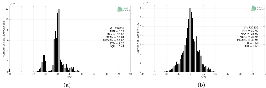
Figure 2: Histograms of SSS from TSG (SAMOS) (a) and SMOS SSS L4 OI v342 - Weekly (CMEMS-CATDS-LOPS) (b) considering all match-up pairs per bins of 0.1 over the Roaring Forties and Furious Fifties Pi-MEP region and for the full satellite product period.
