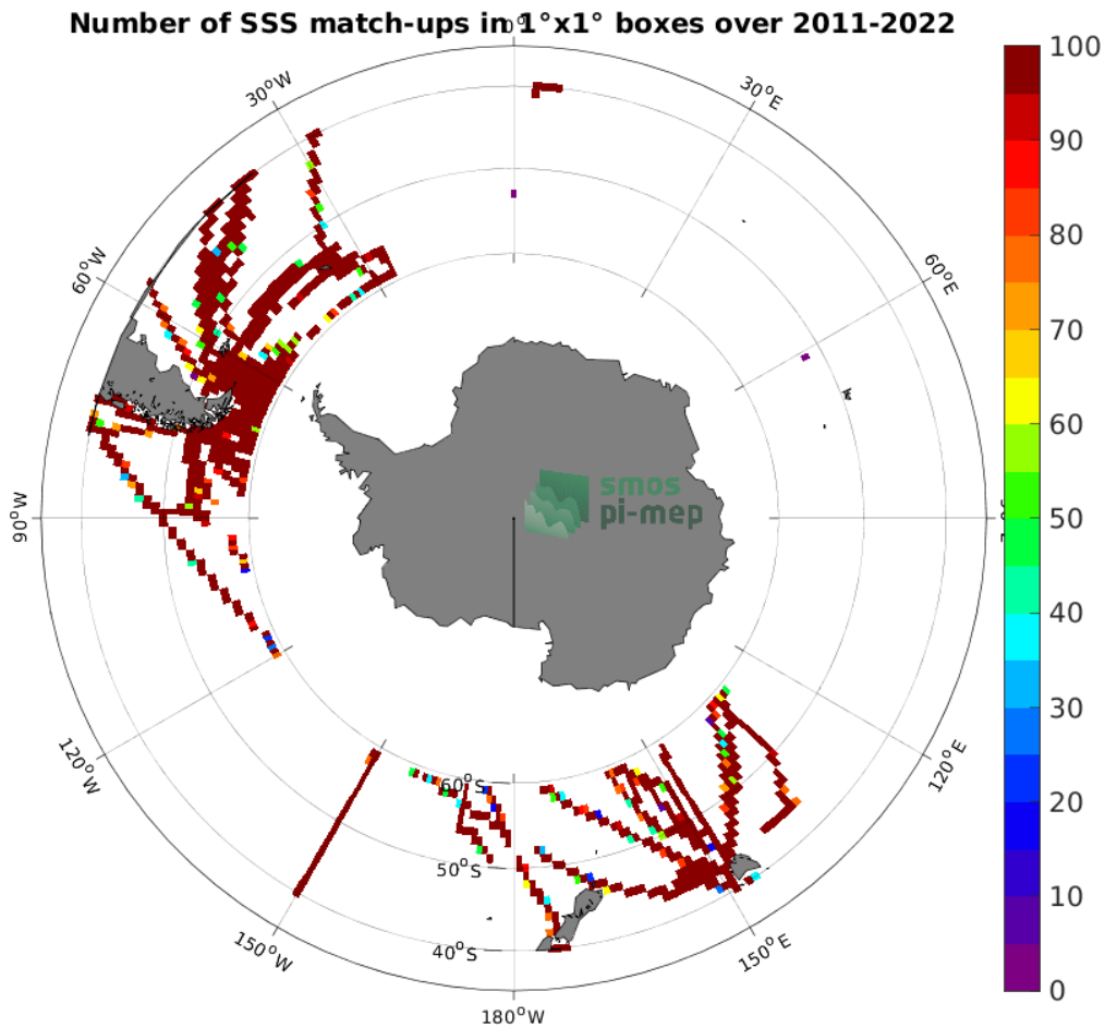
Figure 4: Number of SSS match-ups between TSG (SAMOS) SSS and the SMOS SSS L4 OI v342 - Weekly (CMEMS-CATDS-LOPS) SSS product for the Roaring Forties and Furious Fifties Pi-MEP region over 1^\circ \times 1^\circ boxes and for the full satellite product period.
