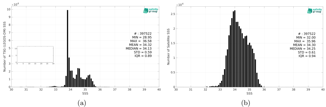
Figure 2: Histograms of SSS from TSG (LEGOS-DM) (a) and SMOS SSS L4 OI v342 - Weekly (CMEMS-CATDS-LOPS) (b) considering all match-up pairs per bins of 0.1 over the Roaring Forties and Furious Fifties Pi-MEP region and for the full satellite product period.
