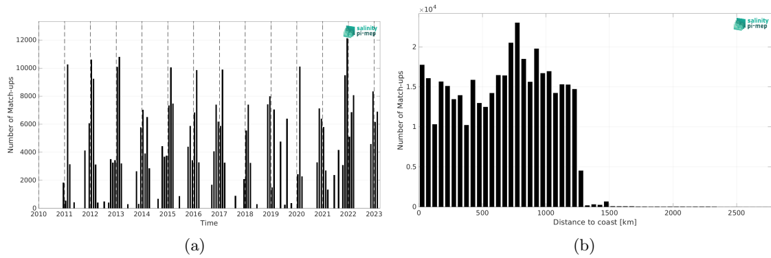
Figure 1: Number of match-ups between TSG (LEGOS-DM) and SMOS SSS L4 OI v342 - Weekly (CMEMS-CATDS-LOPS) SSS as a function of time (a) and as function of the distance to coast (b) over the Roaring Forties and Furious Fifties Pi-MEP region and for the full satellite product period.
