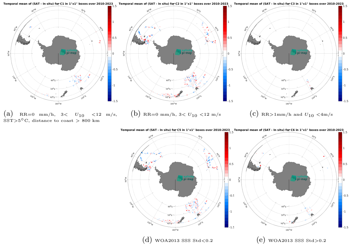
Figure 12: Temporal mean gridded over spatial boxes of size 1^{\circ}\times 1^{\circ} of \Delta\text{SSS} (SMOS SSS L4 OI v342 - Weekly (CMEMS-CATDS-LOPS) - TSG (LEGOS-DM)) for 5 different subdatasets corresponding to:RR=0 mm/h, 3 < U_{10} < 12 m/s, SST >5^{\circ}\text{C} , distance to coast > 800 km (a), RR=0 mm/h, 3 < U_{10} < 12 m/s (b), RR >1 mm/h and U_{10} < 4 m/s (c), WOA2013 SSS Std <0.2 (d), WOA2013 SSS Std >0.2 (e).
