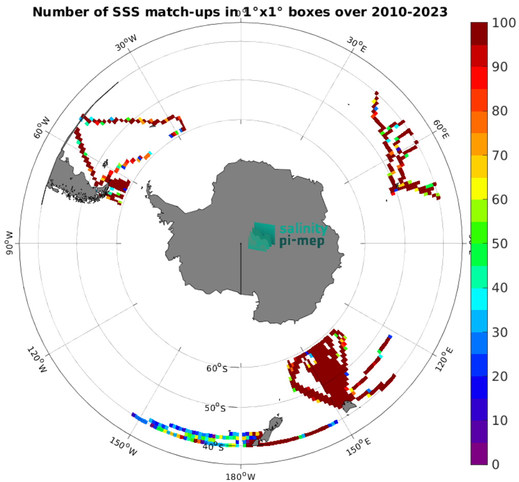
Figure 4: Number of SSS match-ups between TSG (LEGOS-DM) SSS and the SMOS SSS L4 OI v342 - Weekly (CMEMS-CATDS-LOPS) SSS product for the Roaring Forties and Furious Fifties Pi-MEP region over 1^\circ \times 1^\circ boxes and for the full satellite product period.
