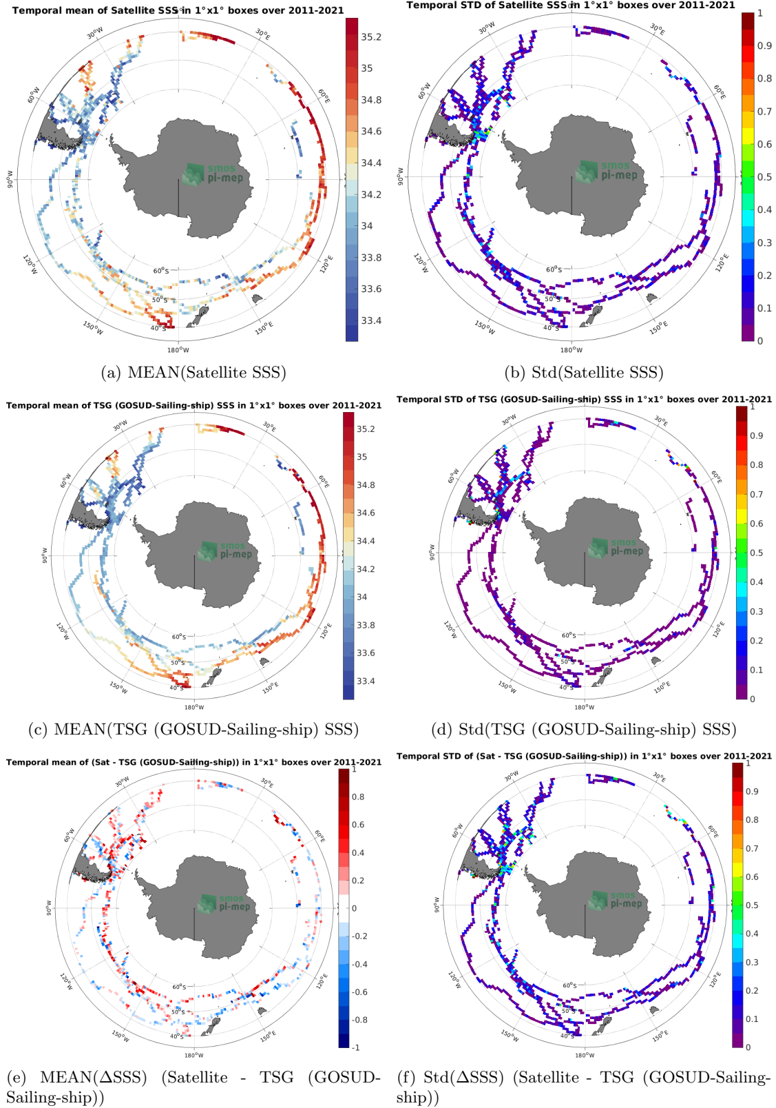
Figure 6: Temporal mean (left) and Std (right), of SSS from SMOS SSS L4 OI v342 - Weekly (CMEMS-CATDS-LOPS) (top), TSG (GOSUD-Sailing-ship) (middle), and of \Delta SSS (Satellite - TSG (GOSUD-Sailing-ship)). Only match-up pairs are used to generate these maps.
