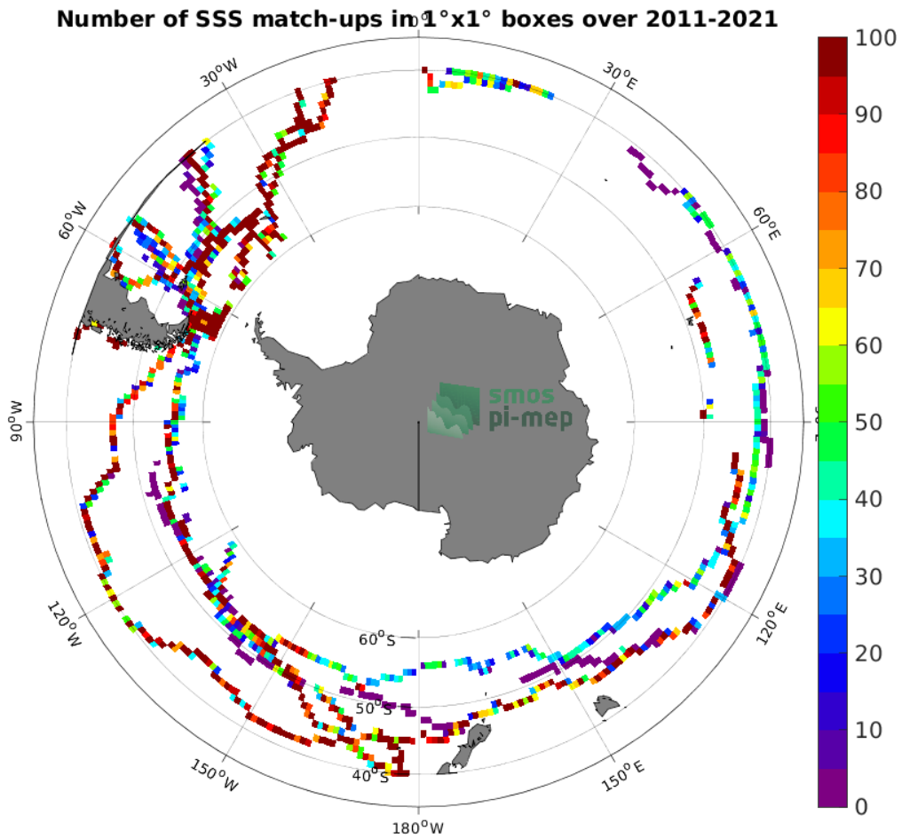
Figure 4: Number of SSS match-ups between TSG (GOSUD-Sailing-ship) SSS and the SMOS SSS L4 OI v342 - Weekly (CMEMS-CATDS-LOPS) SSS product for the Roaring Forties and Furious Fifties Pi-MEP region over 1^\circ \times 1^\circ boxes and for the full satellite product period.
