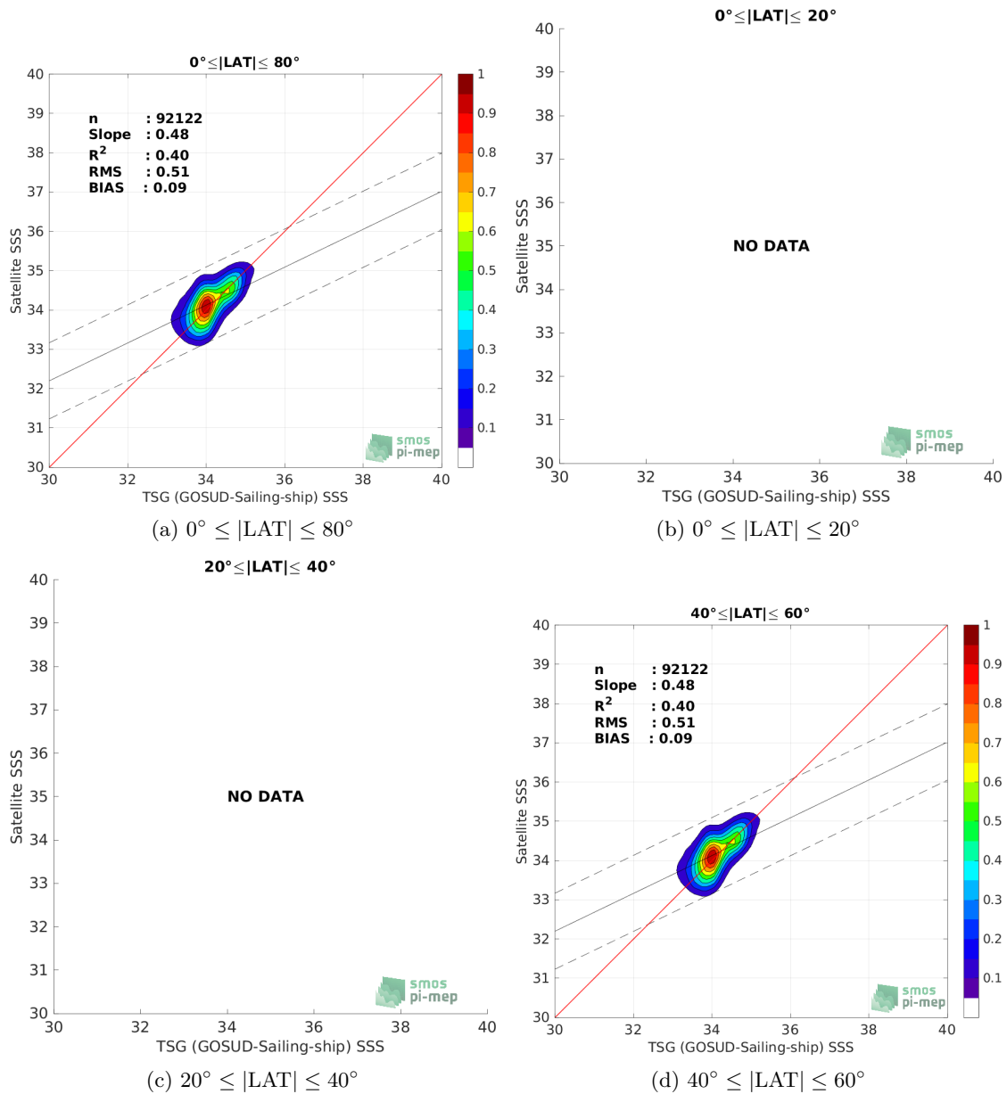
Figure 9: Contour maps of the concentration of SMOS SSS L4 OI v342 - Weekly (CMEMS-CATDS-LOPS) SSS (y-axis) versus TSG (GOSUD-Sailing-ship) SSS (x-axis) at match-up pairs for different latitude bands. For each plot, the red line shows x=y . The black thin and dashed lines indicate a linear fit through the data cloud and the \pm 95\% confidence levels, respectively. The number match-up pairs n , the slope and R^2 coefficient of the linear fit, the root mean square (RMS) and the mean bias between satellite and in situ data are indicated for each latitude band in each plots.
