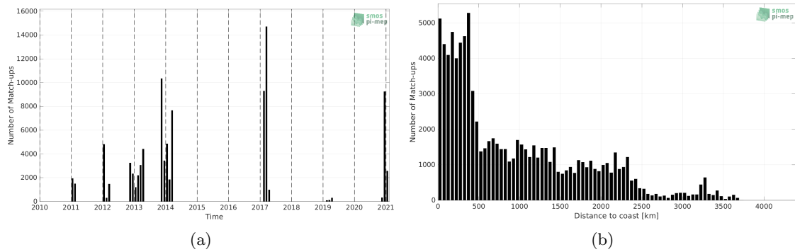
Figure 1: Number of match-ups between TSG (GOSUD-Sailing-ship) and SMOS SSS L4 OI v342 - Weekly (CMEMS-CATDS-LOPS) SSS as a function of time (a) and as function of the distance to coast (b) over the Roaring Forties and Furious Fifties Pi-MEP region and for the full satellite product period.
