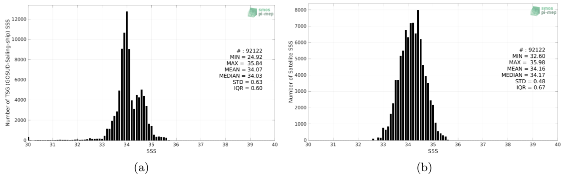
Figure 2: Histograms of SSS from TSG (GOSUD-Sailing-ship) (a) and SMOS SSS L4 OI v342 - Weekly (CMEMS-CATDS-LOPS) (b) considering all match-up pairs per bins of 0.1 over the Roaring Forties and Furious Fifties Pi-MEP region and for the full satellite product period.
