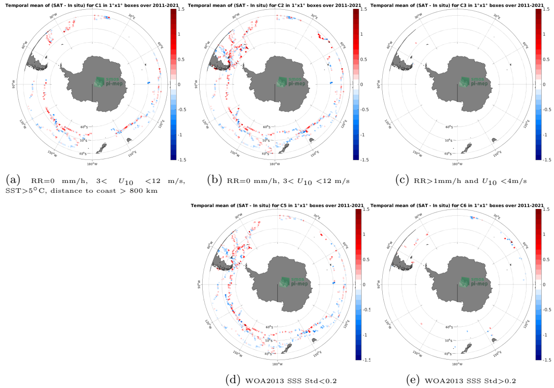
Figure 12: Temporal mean gridded over spatial boxes of size 1^\circ \times 1^\circ of \Delta\text{SSS} (SMOS SSS L4 OI v342 - Weekly (CMEMS-CATDS-LOPS) - TSG (GOSUD-Sailing-ship)) for 5 different sub-datasets corresponding to: RR=0 mm/h, 3 < U_{10} < 12 m/s, SST > 5^\circ\text{C} , distance to coast > 800 km (a), RR=0 mm/h, 3 < U_{10} < 12 m/s (b), RR > 1 mm/h and U_{10} < 4 m/s (c), WOA2013 SSS Std < 0.2 (d), WOA2013 SSS Std > 0.2 (e).
