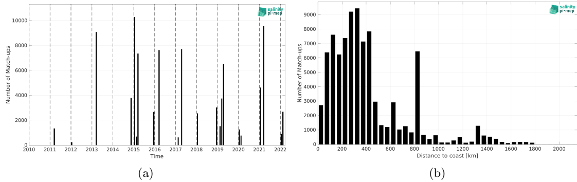
Figure 1: Number of match-ups between TSG (CSIC-UTM) and SMOS SSS L4 OI v342 - Weekly (CMEMS-CATDS-LOPS) SSS as a function of time (a) and as function of the distance to coast (b) over the Roaring Forties and Furious Fifties Pi-MEP region and for the full satellite product period.
