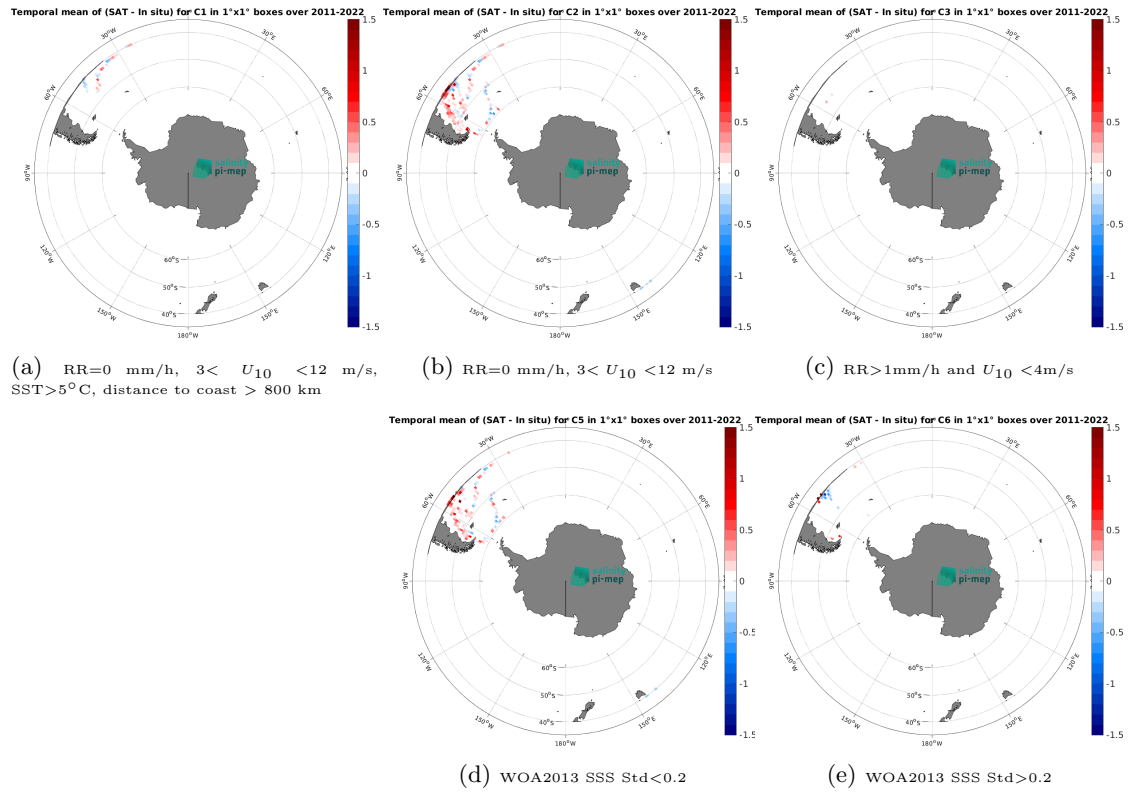
Figure 12: Temporal mean gridded over spatial boxes of size 1^{\circ}\times 1^{\circ} of \Delta\text{SSS} (SMOS SSS L4 OI v342 - Weekly (CMEMS-CATDS-LOPS) - TSG (CSIC-UTM)) for 5 different subdatasets corresponding to:RR=0 mm/h, 3 < U_{10} < 12 m/s, SST >5^{\circ}\text{C} , distance to coast > 800 km (a), RR=0 mm/h, 3 < U_{10} < 12 m/s (b), RR >1 mm/h and U_{10} < 4 m/s (c), WOA2013 SSS Std <0.2 (d), WOA2013 SSS Std >0.2 (e).
