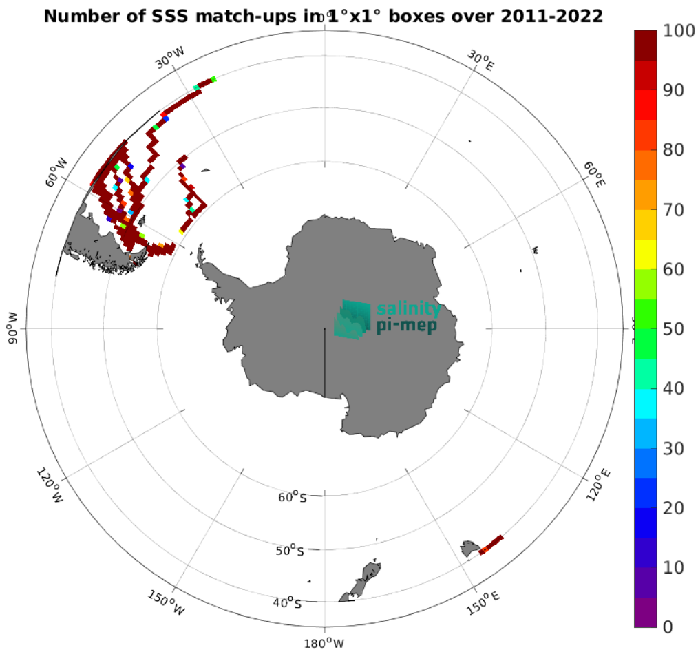
Figure 4: Number of SSS match-ups between TSG (CSIC-UTM) SSS and the SMOS SSS L4 OI v342 - Weekly (CMEMS-CATDS-LOPS) SSS product for the Roaring Forties and Furious Fifties Pi-MEP region over 1^\circ \times 1^\circ boxes and for the full satellite product period.
