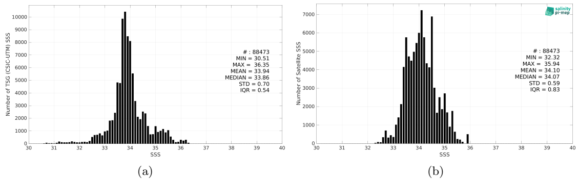
Figure 2: Histograms of SSS from TSG (CSIC-UTM) (a) and SMOS SSS L4 OI v342 - Weekly (CMEMS-CATDS-LOPS) (b) considering all match-up pairs per bins of 0.1 over the Roaring Forties and Furious Fifties Pi-MEP region and for the full satellite product period.
