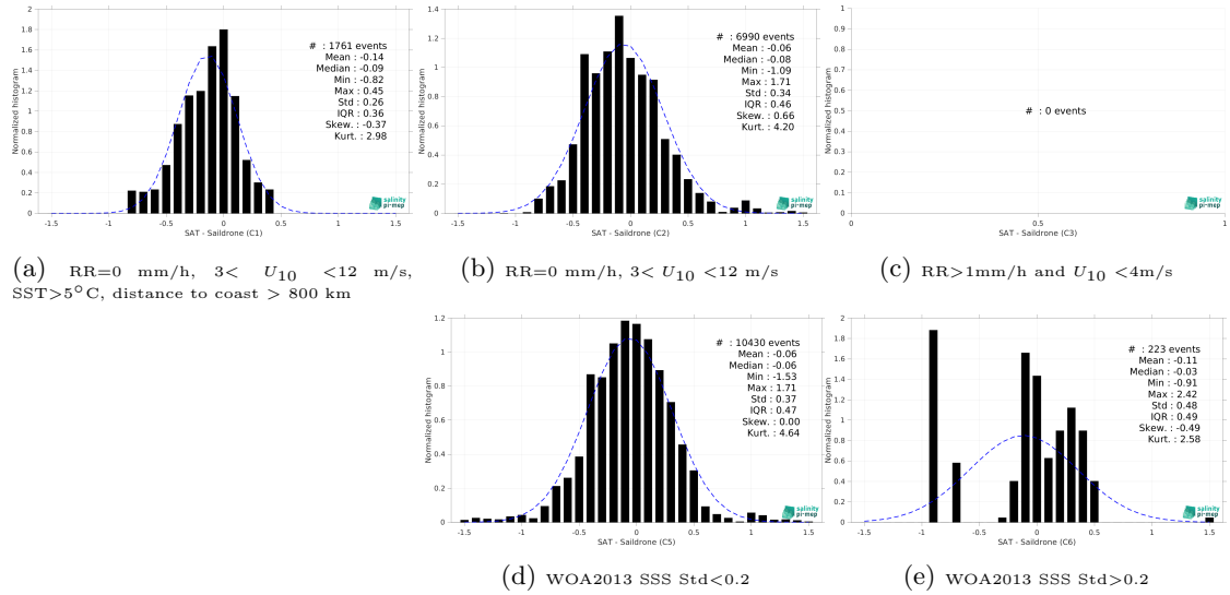
Figure 13: Normalized histogram of \Delta SSS (SMOS SSS L4 OI v342 - Weekly (CMEMS-CATDS-LOPS) - Saldrone) for 5 different subdatasets corresponding to: RR=0 mm/h, 3 < U_{10} < 12 m/s, SST > 5°C, distance to coast > 800 km (a), RR=0 mm/h, 3 < U_{10} < 12 m/s (b), RR > 1mm/h and U_{10} < 4 m/s (c), WOA2013 SSS Std < 0.2 (d), WOA2013 SSS Std > 0.2 (e).
