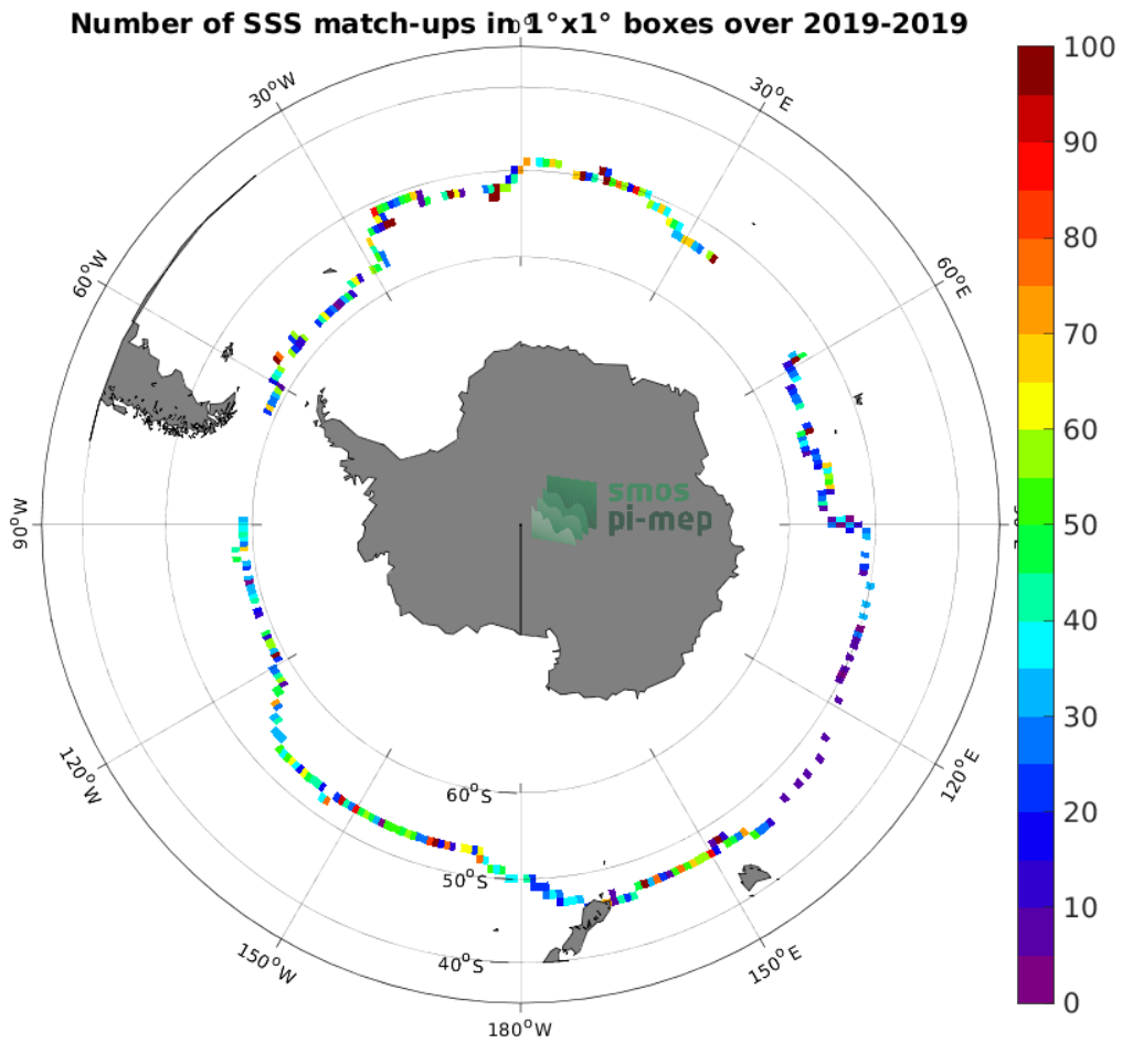
Figure 4: Number of SSS match-ups between Saildrone SSS and the SMOS SSS L4 OI v342 - Weekly (CMEMS-CATDS-LOPS) SSS product for the Roaring Forties and Furious Fifties Pi-MEP region over 1^\circ \times 1^\circ boxes and for the full satellite product period.
