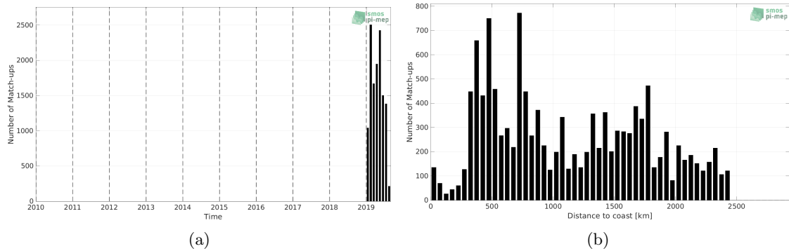
Figure 1: Number of match-ups between Saildrone and SMOS SSS L4 OI v342 - Weekly (CMEMS-CATDS-LOPS) SSS as a function of time (a) and as function of the distance to coast (b) over the Roaring Forties and Furious Fifties Pi-MEP region and for the full satellite product period.
