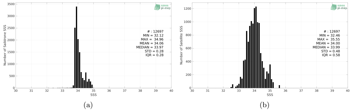
Figure 2: Histograms of SSS from Saildrone (a) and SMOS SSS L4 OI v342 - Weekly (CMEMS-CATDS-LOPS) (b) considering all match-up pairs per bins of 0.1 over the Roaring Forties and Furious Fifties Pi-MEP region and for the full satellite product period.
