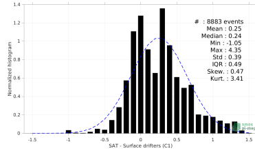
(a) RR=0 mm/h, 3 < U_{10} < 12 m/s, SST>5°C, distance to coast > 800 km
