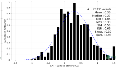
(b) RR=0 mm/h, 3 < U_{10} < 12 m/s
