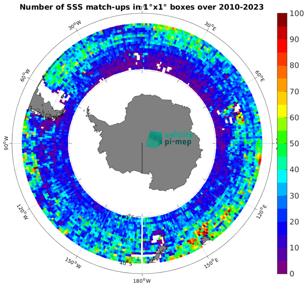
Figure 4: Number of SSS match-ups between Argo SSS and the SMOS SSS L4 OI v342 - Weekly (CMEMS-CATDS-LOPS) SSS product for the Roaring Forties and Furious Fifties Pi-MEP region over 1^{\circ} \times 1^{\circ} boxes and for the full satellite product period.
