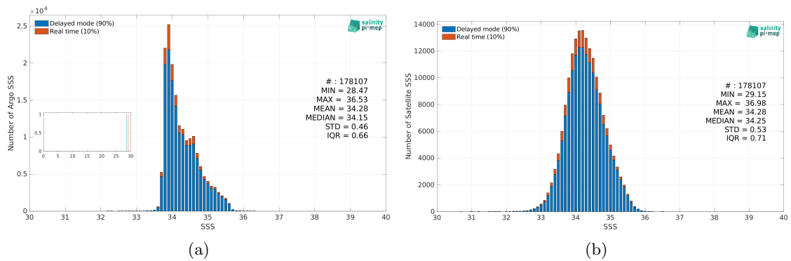
Figure 2: Histograms of SSS from Argo (a) and SMOS SSS L4 OI v342 - Weekly (CMEMS-CATDS-LOPS) (b) considering all match-up pairs per bins of 0.1 over the Roaring Forties and Furious Fifties Pi-MEP region and for the full satellite product period.
