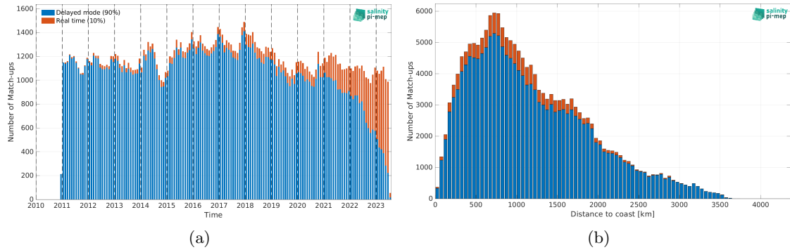
Figure 1: Number of match-ups between Argo and SMOS SSS L4 OI v342 - Weekly (CMEMS-CATDS-LOPS) SSS as a function of time (a) and as function of the distance to coast (b) over the Roaring Forties and Furious Fifties Pi-MEP region and for the full satellite product period.
