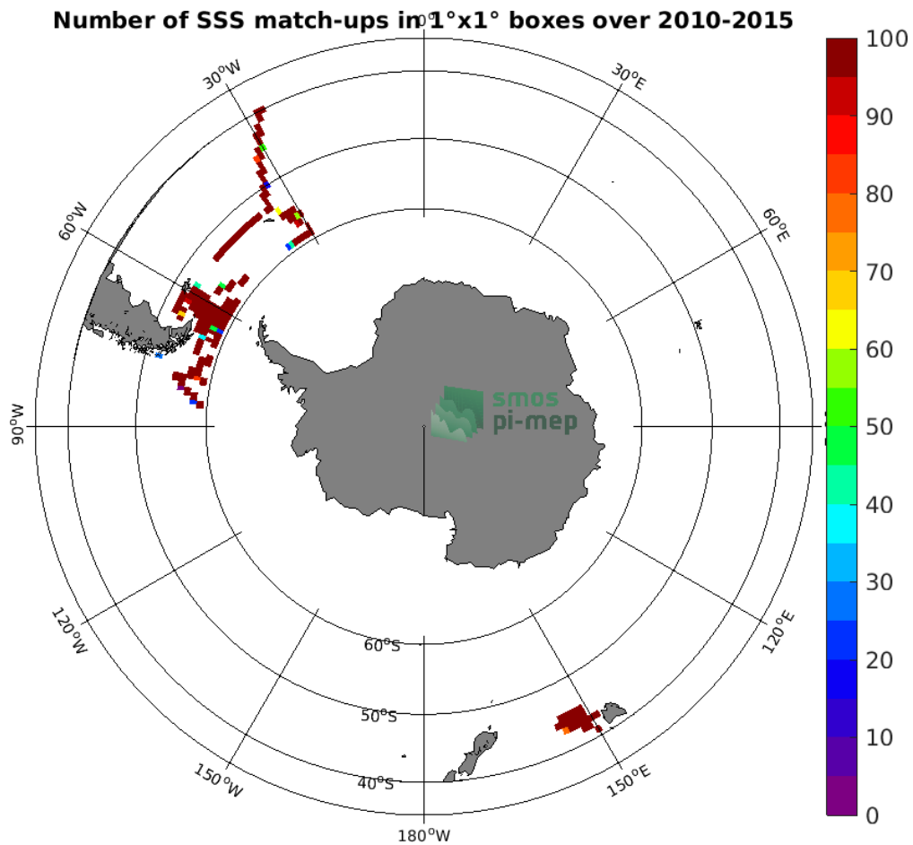
Figure 4: Number of SSS match-ups between TSG (SAMOS) SSS and the SMOS L4 v2 Weekly (CATDS-CECOS-IFREMER) SSS product for the Roaring Forties and Furious Fifties Pi-MEP region over 1°x1° boxes and for the full satellite product period.
