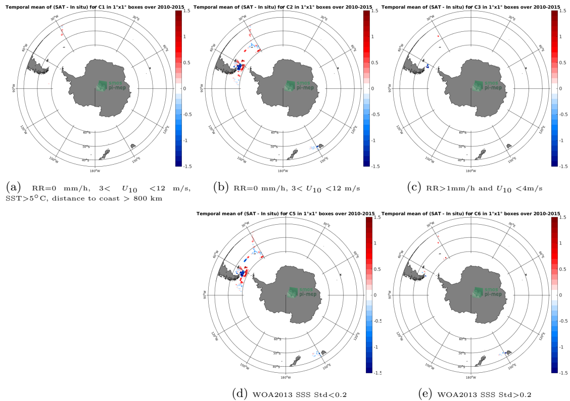
Figure 12: Temporal mean gridded over spatial boxes of size 1^{\circ}\times 1^{\circ} of \Delta\text{SSS} (SMOS-L4-CATDS-CECOS-IFREMER-V2-WEEKLY-0.5DEG - TSG-SAMOS) for 5 different subdatasets corresponding to:RR=0 mm/h, 3 < U_{10} < 12 m/s, SST >5^{\circ}\text{C} , distance to coast > 800 km (a), RR=0 mm/h, 3 < U_{10} < 12 m/s (b), RR >1 mm/h and U_{10} < 4 m/s (c), WOA2013 SSS Std <0.2 (d), WOA2013 SSS Std >0.2 (e).
