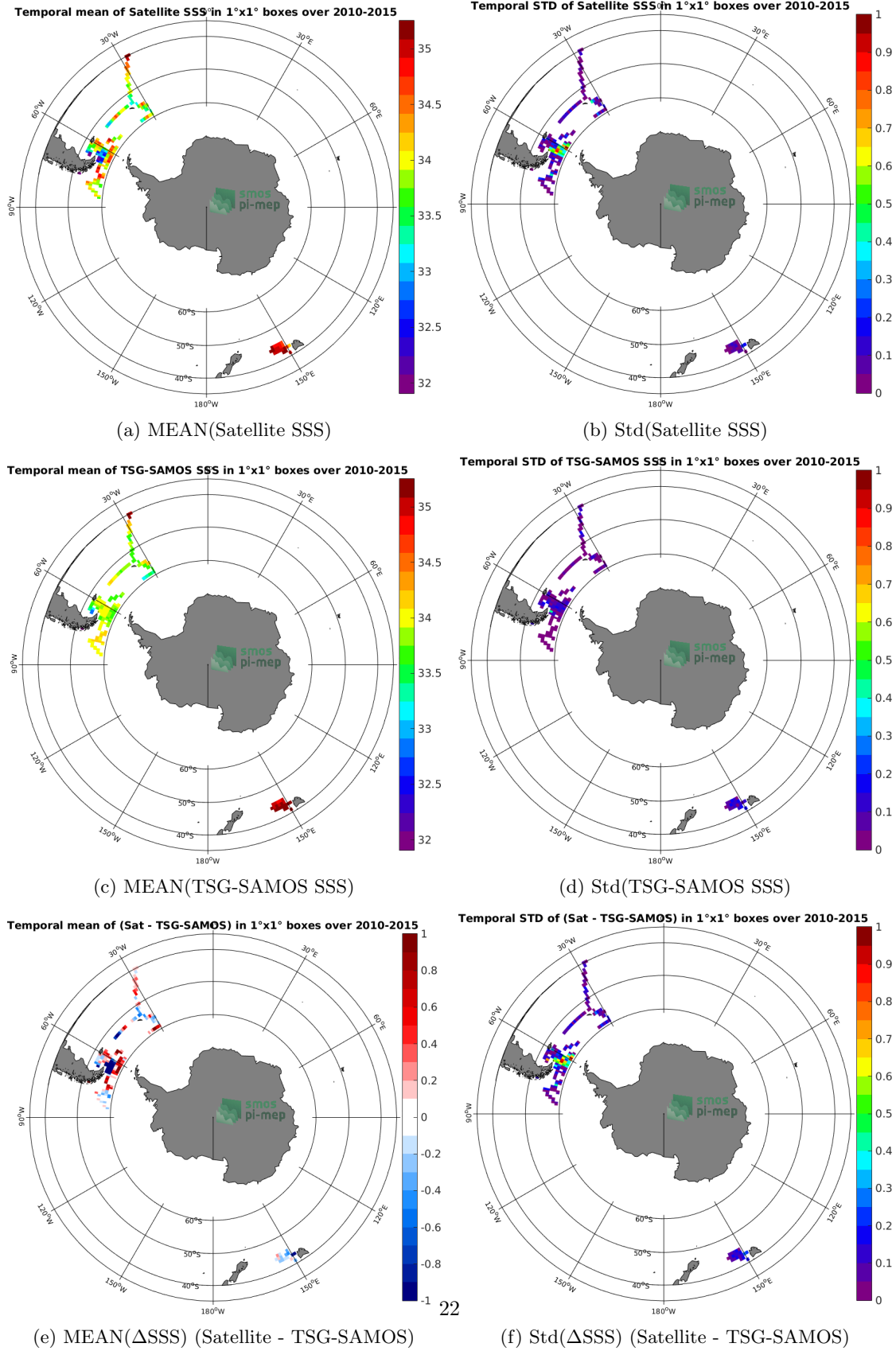
Figure 6: Temporal mean (left) and Std (right) of SSS from SMOS-L4-CATDS-CECOS-IFREMER-V2-WEEKLY-0.5DEG (top), TSG-SAMOS (middle), and of \Delta SSS (Satellite - TSG-SAMOS). Only match-up pairs are used to generate these maps.
