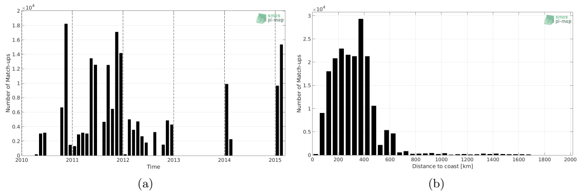
Figure 1: Number of match-ups between TSG-SAMOS and SMOS-L4-CATDS-CECOS-IFREMER-V2-WEEKLY-0.5DEG SSS as a function of time (a) and as function of the distance to coast (b) over the Roaring Forties and Furious Fifties Pi-MEP region and for the full satellite product period.
