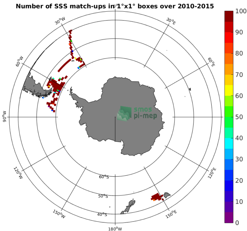
Figure 4: Number of SSS match-ups between TSG-SAMOS SSS and the SMOS-L4-CATDS-CECOS-IFREMER-V2-WEEKLY-0.5DEG SSS product for the Roaring Forties and Furious Fifties Pi-MEP region over 1°x1° boxes and for the full satellite product period.
