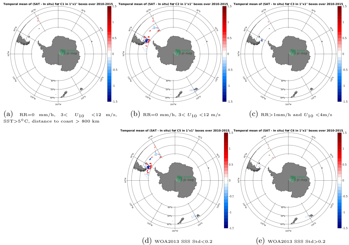
Figure 12: Temporal mean gridded over spatial boxes of size 1^\circ \times 1^\circ of \Delta SSS (SMOS-L4-CATDS-CECOS-IFREMER-V2-WEEKLY-0.5DEG - TSG-SAMOS) for 5 different subdatasets corresponding to: RR=0 mm/h, 3 < U_{10} < 12 m/s, SST > 5^\circ\text{C} , distance to coast > 800 km (a), RR=0 mm/h, 3 < U_{10} < 12 m/s (b), RR > 1 mm/h and U_{10} < 4 m/s (c), WOA2013 SSS Std < 0.2 (d), WOA2013 SSS Std > 0.2 (e).
