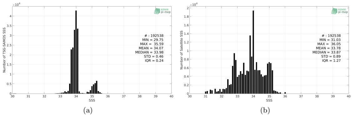
Figure 2: Histograms of SSS from TSG-SAMOS (a) and SMOS-L4-CATDS-CECOS-IFREMER-V2-WEEKLY-0.5DEG (b) considering all match-up pairs per bins of 0.1 over the Roaring Forties and Furious Fifties Pi-MEP region and for the full satellite product period.
