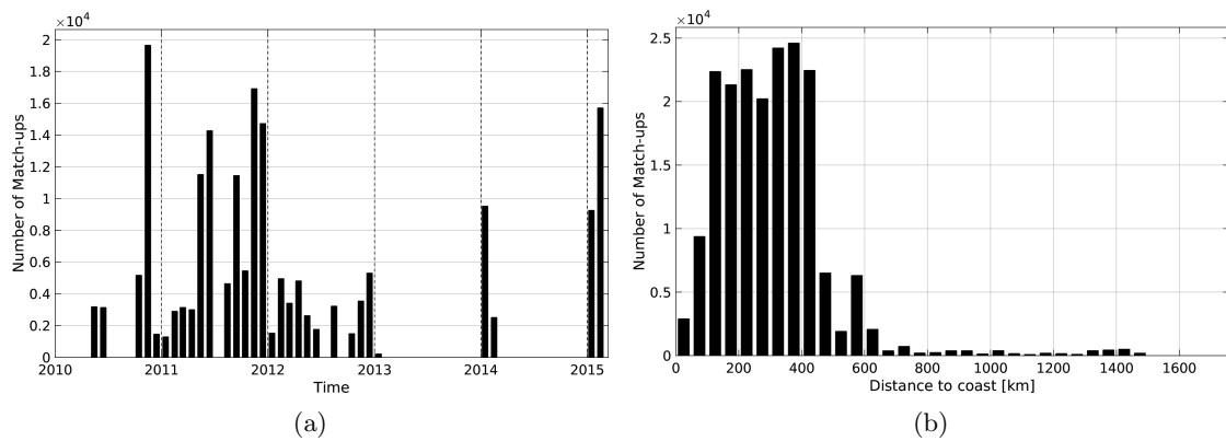
Figure 1: Number of match-ups between TSG-SAMOS and SMOS-L4-CATDS-CECOS-IFREMER-V2-WEEKLY-0.5DEG SSS as a function of time (a) and as function of the distance to coast (b) over the Roaring Forties and Furious Fifties Pi-MEP region and for the full satellite product period.
