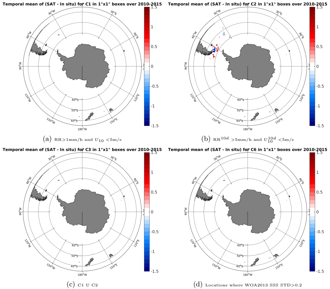
Figure 12: Temporal mean gridded over spatial boxes of size 1^\circ \times 1^\circ of \Delta SSS (SMOS-L4-CATDS-CECOS-IFREMER-V2-WEEKLY-0.5DEG - TSG-SAMOS) for 4 different subdatasets corresponding to: RR > 1\text{mm/h} and U_{10} < 5\text{m/s} (a), RR^{10d} > 5\text{mm/h} and U_{10}^{10d} < 5\text{m/s} (b), C1 U C2 (c), Locations where WOA2013 SSS STD > 0.2 (d).
