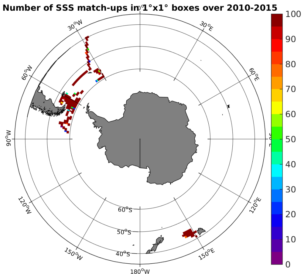
Figure 4: Number of SSS match-ups between TSG-SAMOS SSS and the SMOS-L4-CATDS-CECOS-IFREMER-V2-WEEKLY-0.5DEG SSS product for the Roaring Forties and Furious Fifties Pi-MEP region over 1°x1° boxes and for the full satellite product period.
