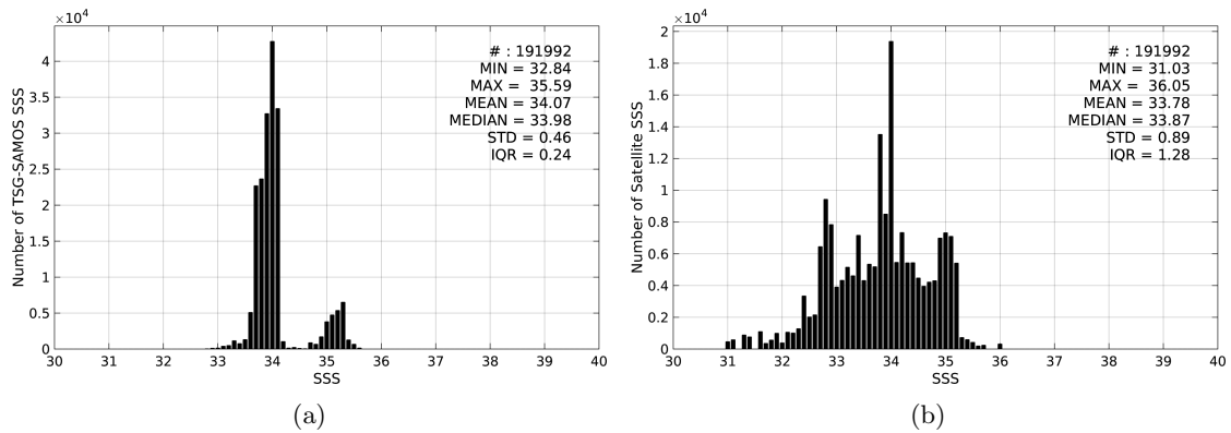
Figure 2: Histograms of SSS from TSG-SAMOS (a) and SMOS-L4-CATDS-CECOS-IFREMER-V2-WEEKLY-0.5DEG (b) considering all match-up pairs per bins of 0.1 over the Roaring Forties and Furious Fifties Pi-MEP region and for the full satellite product period.
