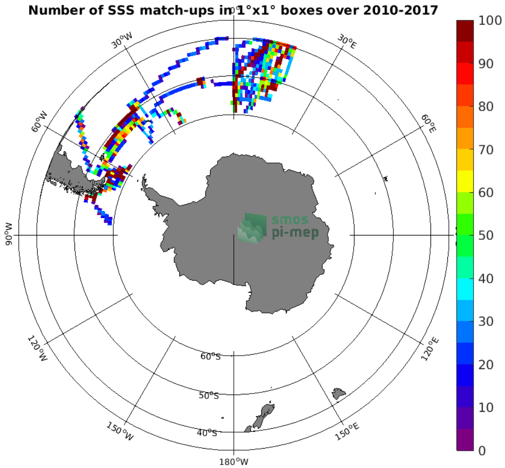
Figure 4: Number of SSS match-ups between TSG (Polarstern) SSS and the SMOS L4 v2 Weekly (CATDS-CECOS-IFREMER) SSS product for the Roaring Forties and Furious Fifties Pi-MEP region over 1°x1° boxes and for the full satellite product period.
