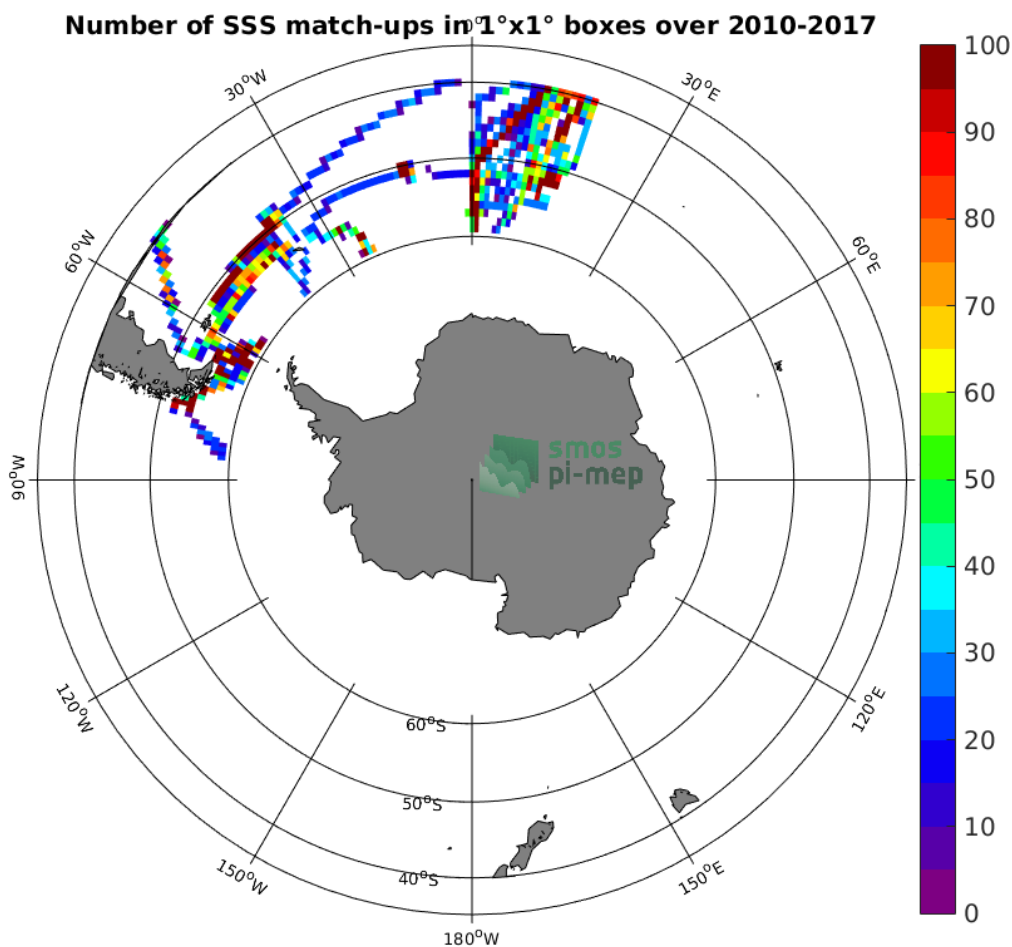
Figure 4: Number of SSS match-ups between TSG-POLARSTERN SSS and the SMOS-L4-CATDS-CECOS-IFREMER-V2-WEEKLY-0.5DEG SSS product for the Roaring Forties and Furious Fifties Pi-MEP region over 1°x1° boxes and for the full satellite product period.
