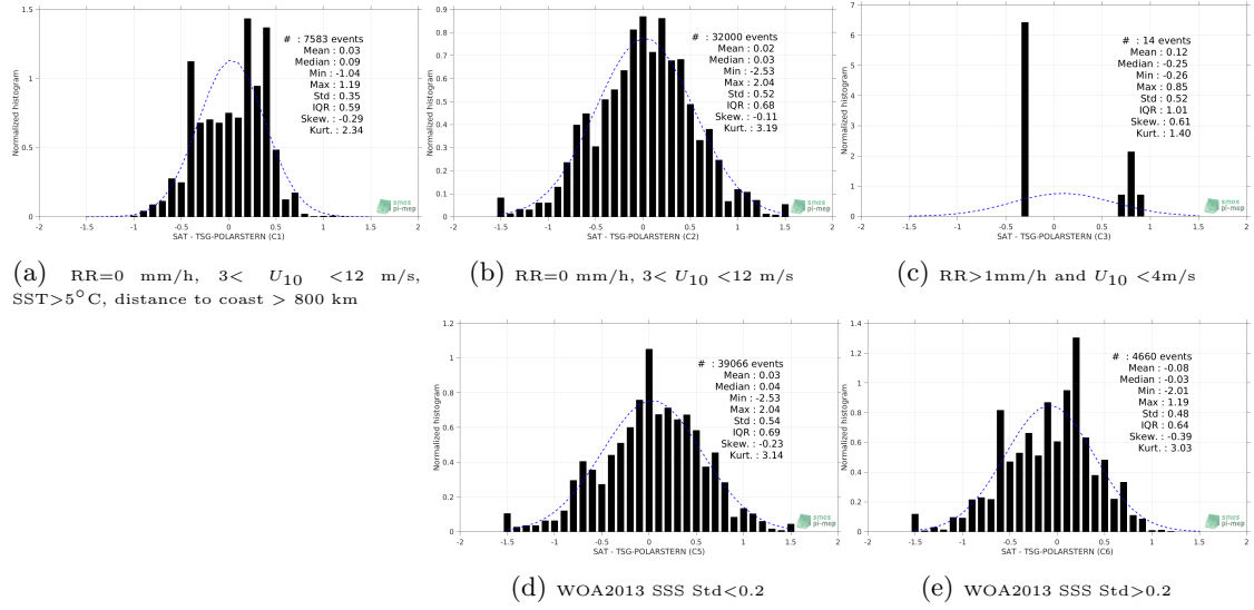
Figure 13: Normalized histogram of \Delta\text{SSS} (SMOS-L4-CATDS-CECOS-IFREMER-V2-WEEKLY-0.5DEG - TSG-POLARSTERN) for 5 different subdatasets corresponding to: RR=0 mm/h, 3 < U_{10} < 12 m/s, SST > 5^{\circ}\text{C} , distance to coast > 800 km (a), RR=0 mm/h, 3 < U_{10} < 12 m/s (b), RR > 1\text{mm/h} and U_{10} < 4\text{m/s} (c), WOA2013 SSS Std < 0.2 (d), WOA2013 SSS Std > 0.2 (e).
