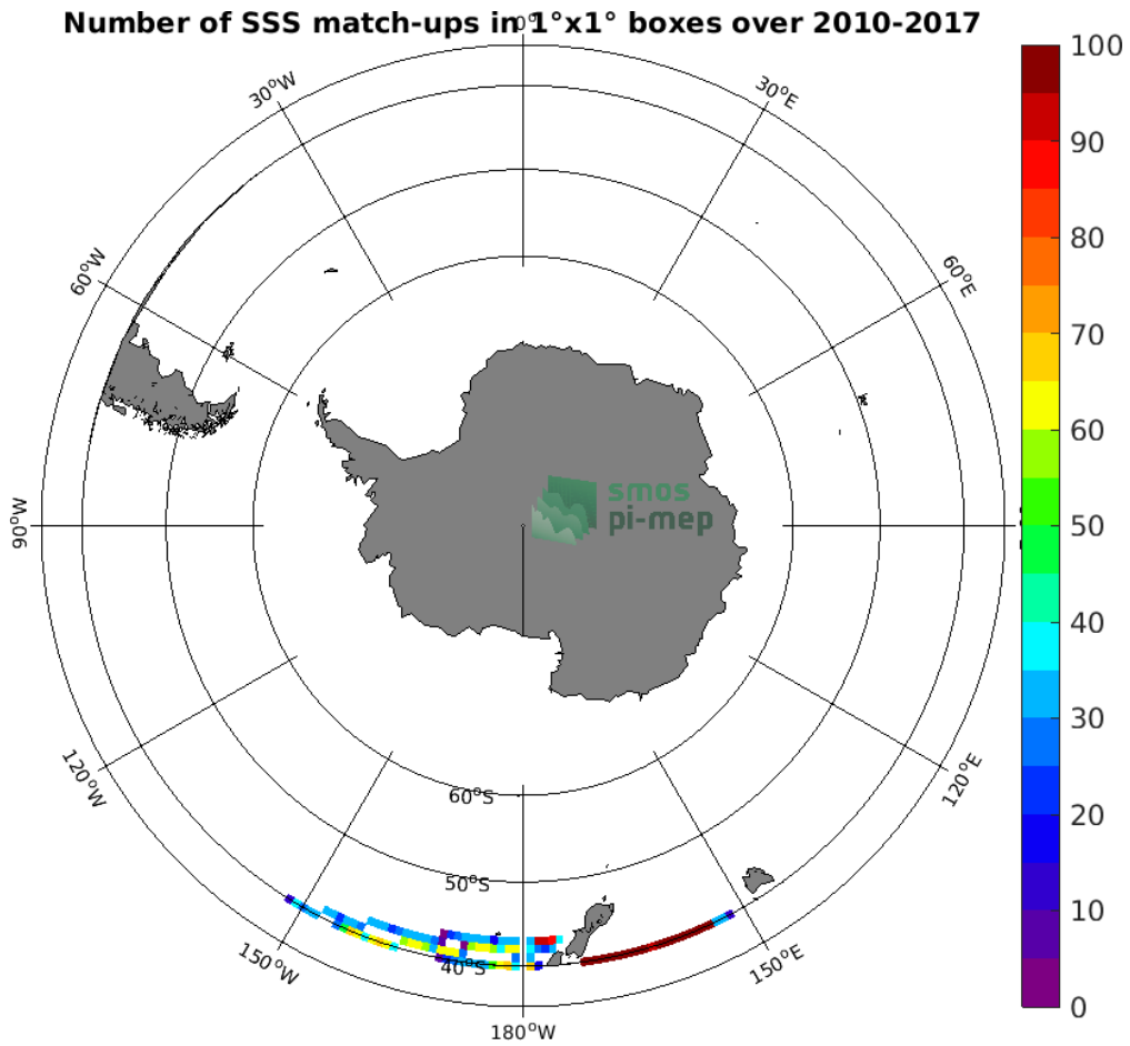
Figure 4: Number of SSS match-ups between TSG (LEGOS-DM) SSS and the SMOS L4 v2 Weekly (CATDS-CECOS-IFREMER) SSS product for the Roaring Forties and Furious Fifties Pi-MEP region over 1^\circ \times 1^\circ boxes and for the full satellite product period.
