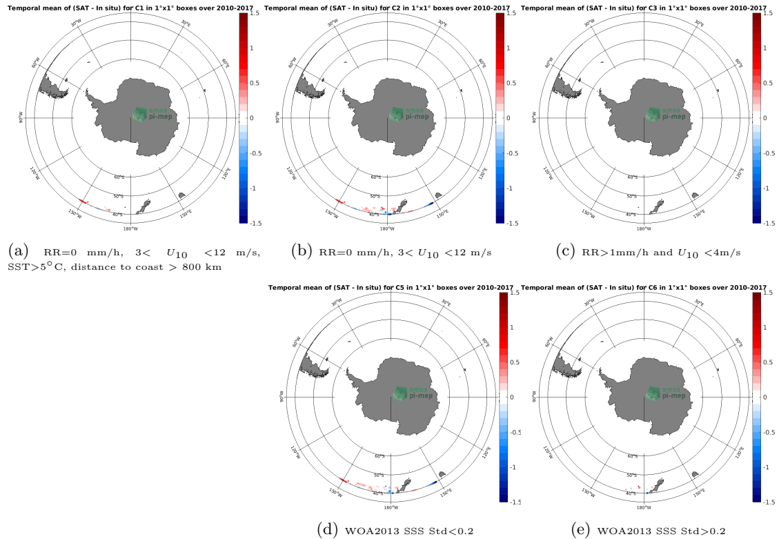
Figure 12: Temporal mean gridded over spatial boxes of size 1^{\circ}\times 1^{\circ} of \Delta\text{SSS} (SMOS L4 v2 Weekly (CATDS-CECOS-IFREMER) - TSG (LEGOS-DM)) for 5 different subdatasets corresponding to:RR=0 mm/h, 3 < U_{10} < 12 m/s, SST >5^{\circ}\text{C} , distance to coast > 800 km (a), RR=0 mm/h, 3 < U_{10} < 12 m/s (b), RR >1 mm/h and U_{10} < 4 m/s (c), WOA2013 SSS Std <0.2 (d), WOA2013 SSS Std >0.2 (e).
