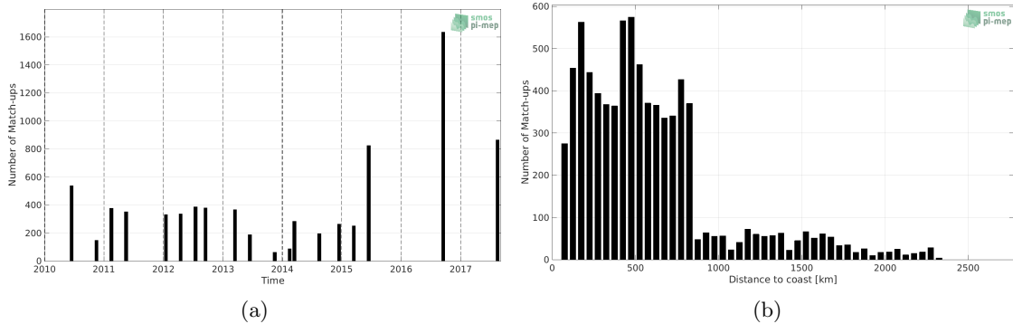
Figure 1: Number of match-ups between TSG (LEGOS-DM) and SMOS L4 v2 Weekly (CATDS-CECOS-IFREMER) SSS as a function of time (a) and as function of the distance to coast (b) over the Roaring Forties and Furious Fifties Pi-MEP region and for the full satellite product period.
