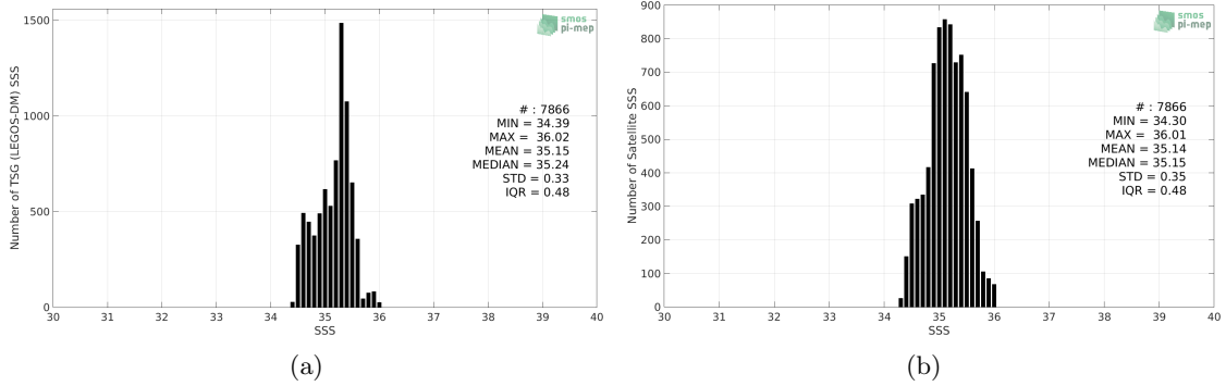
Figure 2: Histograms of SSS from TSG (LEGOS-DM) (a) and SMOS L4 v2 Weekly (CATDS-CECOS-IFREMER) (b) considering all match-up pairs per bins of 0.1 over the Roaring Forties and Furious Fifties Pi-MEP region and for the full satellite product period.
