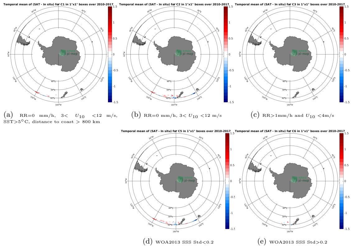
Figure 12: Temporal mean gridded over spatial boxes of size 1^{\circ}\times 1^{\circ} of \Delta\text{SSS} (SMOS-L4-CATDS-CECOS-IFREMER-V2-WEEKLY-0.5DEG - TSG-LEGOS-DM) for 5 different subdatasets corresponding to:RR=0 mm/h, 3 < U_{10} < 12 m/s, SST >5^{\circ}\text{C} , distance to coast > 800 km (a), RR=0 mm/h, 3 < U_{10} < 12 m/s (b), RR >1 mm/h and U_{10} < 4 m/s (c), WOA2013 SSS Std <0.2 (d), WOA2013 SSS Std >0.2 (e).
