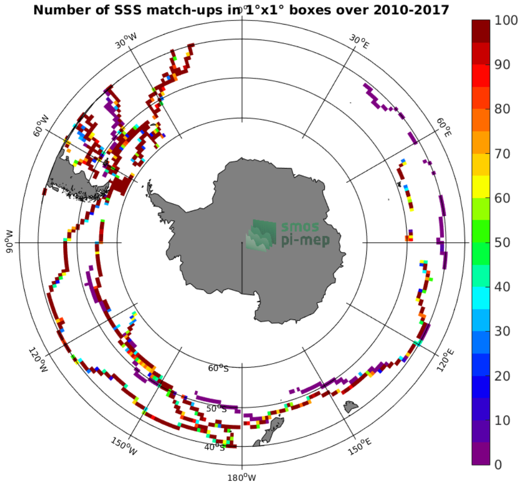
Figure 4: Number of SSS match-ups between TSG-GOSUD-Sailing-ship SSS and the SMOS-L4-CATDS-CECOS-IFREMER-V2-WEEKLY-0.5DEG SSS product for the Roaring Forties and Furious Fifties Pi-MEP region over 1°x1° boxes and for the full satellite product period.
