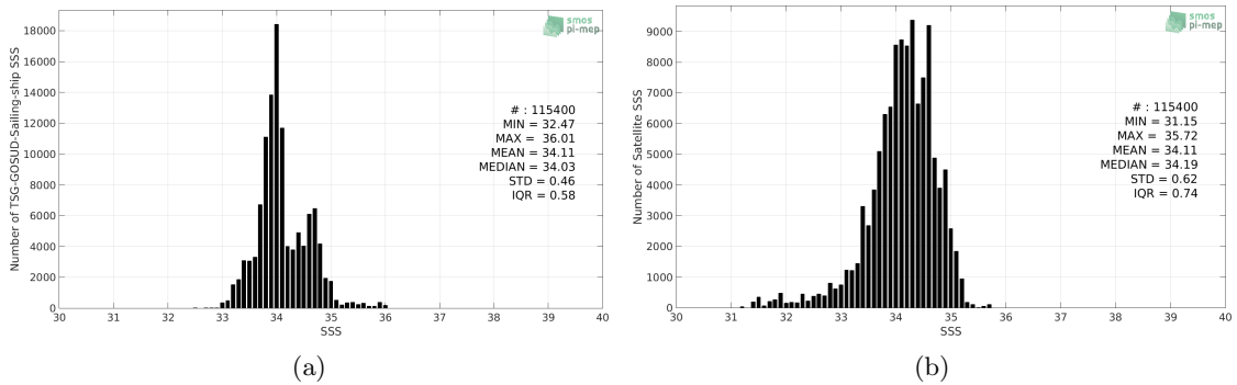
Figure 2: Histograms of SSS from TSG-GOSUD-Sailing-ship (a) and SMOS-L4-CATDS-CECOS-IFREMER-V2-WEEKLY-0.5DEG (b) considering all match-up pairs per bins of 0.1 over the Roaring Forties and Furious Fifties Pi-MEP region and for the full satellite product period.
