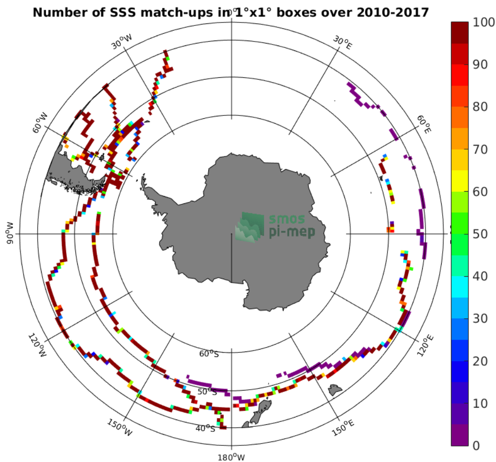
Figure 4: Number of SSS match-ups between TSG-GOSUD-Sailing-ship SSS and the SMOS-L4-CATDS-CECOS-IFREMER-V2-WEEKLY-0.5DEG SSS product for the Roaring Forties and Furious Fifties Pi-MEP region over 1^\circ \times 1^\circ boxes and for the full satellite product period.
