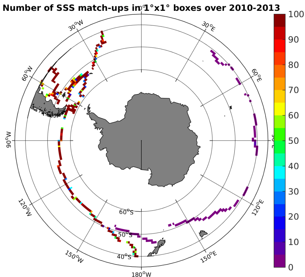
Figure 4: Number of SSS match-ups between TSG-GOSUD-Sailing-ship SSS and the SMOS-L4-CATDS-CECOS-IFREMER-V2-WEEKLY-0.5DEG SSS product for the Roaring Forties and Furious Fifties Pi-MEP region over 1°x1° boxes and for the full satellite product period.
