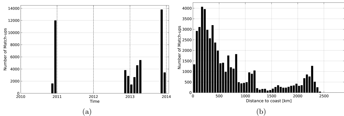
Figure 1: Number of match-ups between TSG-GOSUD-Sailing-ship and SMOS-L4-CATDS-CECOS-IFREMER-V2-WEEKLY-0.5DEG SSS as a function of time (a) and as function of the distance to coast (b) over the Roaring Forties and Furious Fifties Pi-MEP region and for the full satellite product period.
