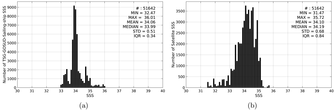
Figure 2: Histograms of SSS from TSG-GOSUD-Sailing-ship (a) and SMOS-L4-CATDS-CECOS-IFREMER-V2-WEEKLY-0.5DEG (b) considering all match-up pairs per bins of 0.1 over the Roaring Forties and Furious Fifties Pi-MEP region and for the full satellite product period.
