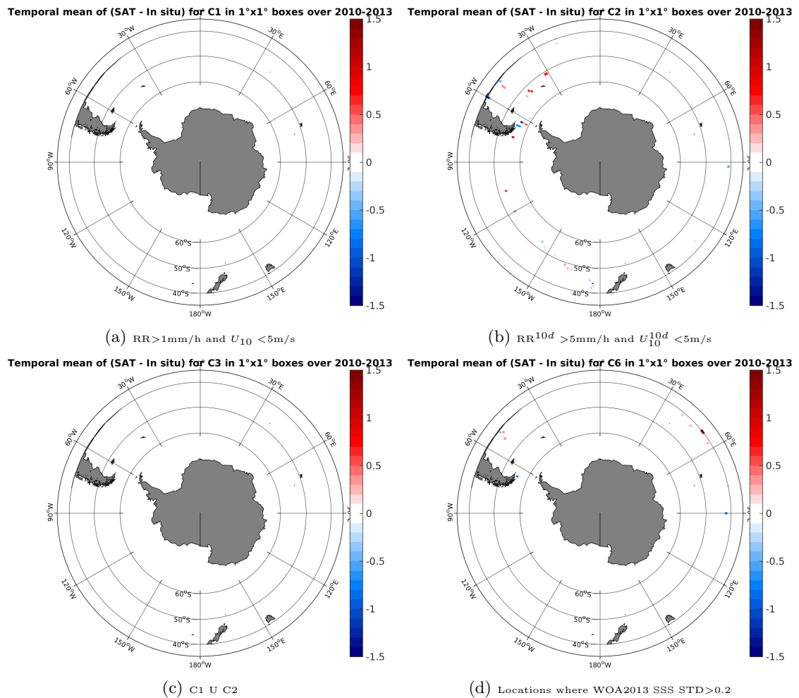
Figure 12: Temporal mean gridded over spatial boxes of size 1^\circ \times 1^\circ of \Delta SSS (SMOS-L4-CATDS-CECOS-IFREMER-V2-WEEKLY-0.5DEG - TSG-GOSUD-Sailing-ship) for 4 different subdatasets corresponding to: RR > 1\text{mm/h} and U_{10} < 5\text{m/s} (a), RR^{10d} > 5\text{mm/h} and U_{10}^{10d} < 5\text{m/s} (b), C1 U C2 (c), Locations where WOA2013 SSS STD > 0.2 (d).
