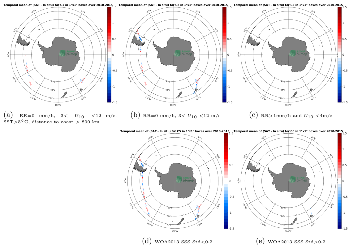
Figure 12: Temporal mean gridded over spatial boxes of size 1^\circ \times 1^\circ of \Delta SSS (SMOS-L4-CATDS-CECOS-IFREMER-V2-WEEKLY-0.5DEG - TSG-GOSUD-Research-vessel) for 5 different sub-datasets corresponding to:RR=0 mm/h, 3 < U_{10} < 12 m/s, SST > 5^\circ\text{C} , distance to coast > 800 km (a), RR=0 mm/h, 3 < U_{10} < 12 m/s (b), RR > 1 mm/h and U_{10} < 4 m/s (c), WOA2013 SSS Std < 0.2 (d), WOA2013 SSS Std > 0.2 (e).
