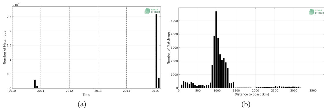
Figure 1: Number of match-ups between TSG-GOSUD-Research-vessel and SMOS-L4-CATDS-CECOS-IFREMER-V2-WEEKLY-0.5DEG SSS as a function of time (a) and as function of the distance to coast (b) over the Roaring Forties and Furious Fifties Pi-MEP region and for the full satellite product period.
