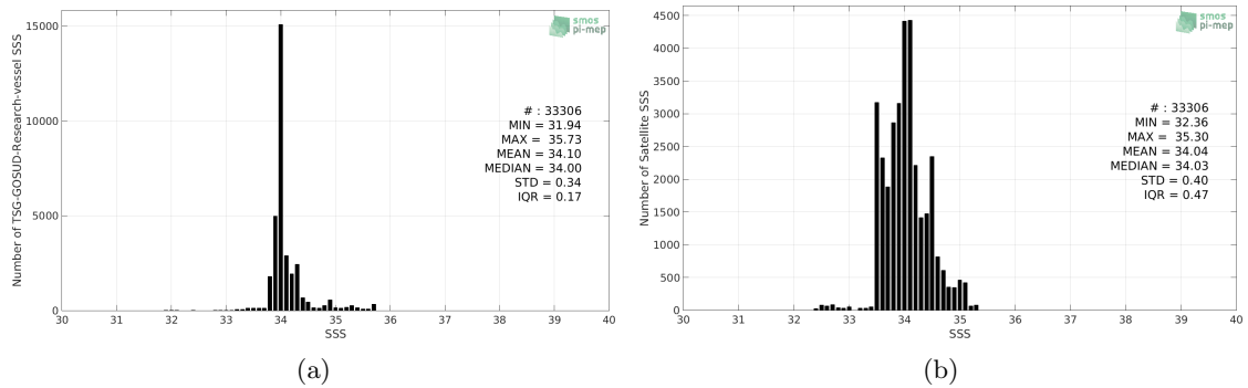
Figure 2: Histograms of SSS from TSG-GOSUD-Research-vessel (a) and SMOS-L4-CATDS-CECOS-IFREMER-V2-WEEKLY-0.5DEG (b) considering all match-up pairs per bins of 0.1 over the Roaring Forties and Furious Fifties Pi-MEP region and for the full satellite product period.
