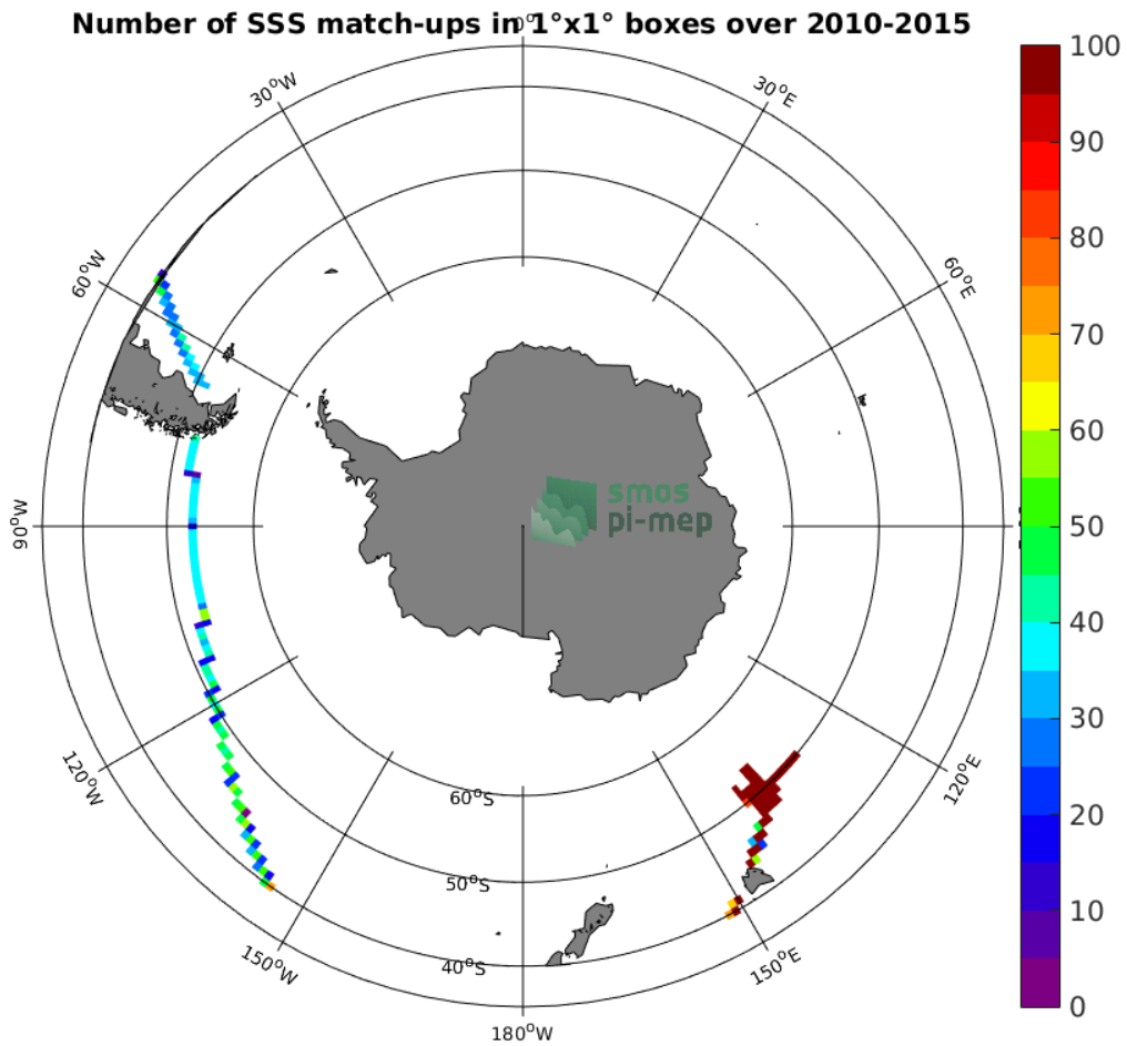
Figure 4: Number of SSS match-ups between TSG-GOSUD-Research-vessel SSS and the SMOS-L4-CATDS-CECOS-IFREMER-V2-WEEKLY-0.5DEG SSS product for the Roaring Forties and Furious Fifties Pi-MEP region over 1°x1° boxes and for the full satellite product period.
