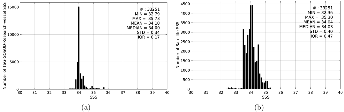
Figure 2: Histograms of SSS from TSG-GOSUD-Research-vessel (a) and SMOS-L4-CATDS-CECOS-IFREMER-V2-WEEKLY-0.5DEG (b) considering all match-up pairs per bins of 0.1 over the Roaring Forties and Furious Fifties Pi-MEP region and for the full satellite product period.
