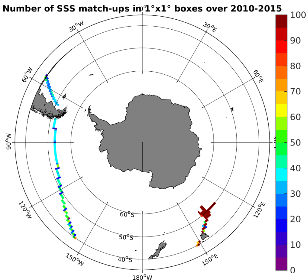
Figure 4: Number of SSS match-ups between TSG-GOSUD-Research-vessel SSS and the SMOS-L4-CATDS-CECOS-IFREMER-V2-WEEKLY-0.5DEG SSS product for the Roaring Forties and Furious Fifties Pi-MEP region over 1°x1° boxes and for the full satellite product period.
