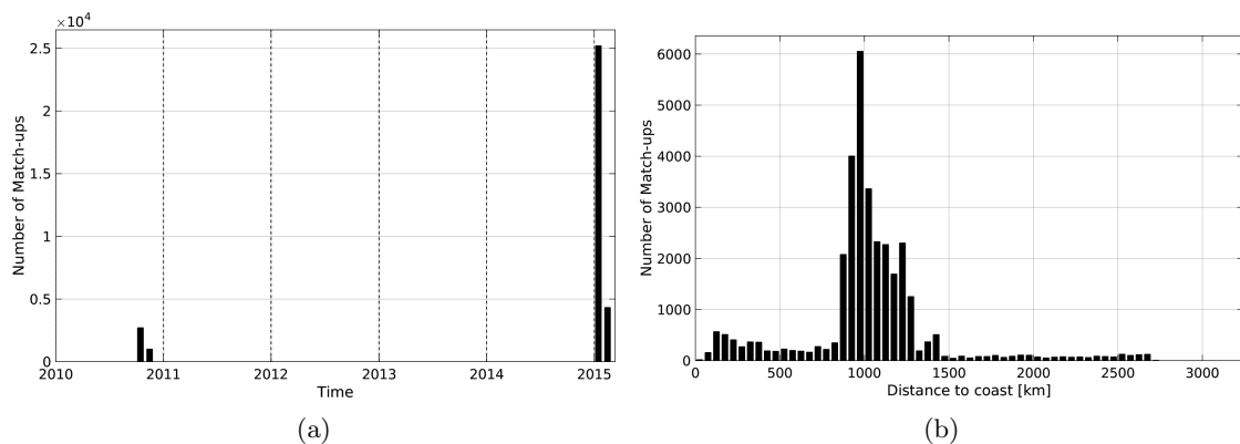
Figure 1: Number of match-ups between TSG-GOSUD-Research-vessel and SMOS-L4-CATDS-CECOS-IFREMER-V2-WEEKLY-0.5DEG SSS as a function of time (a) and as function of the distance to coast (b) over the Roaring Forties and Furious Fifties Pi-MEP region and for the full satellite product period.
