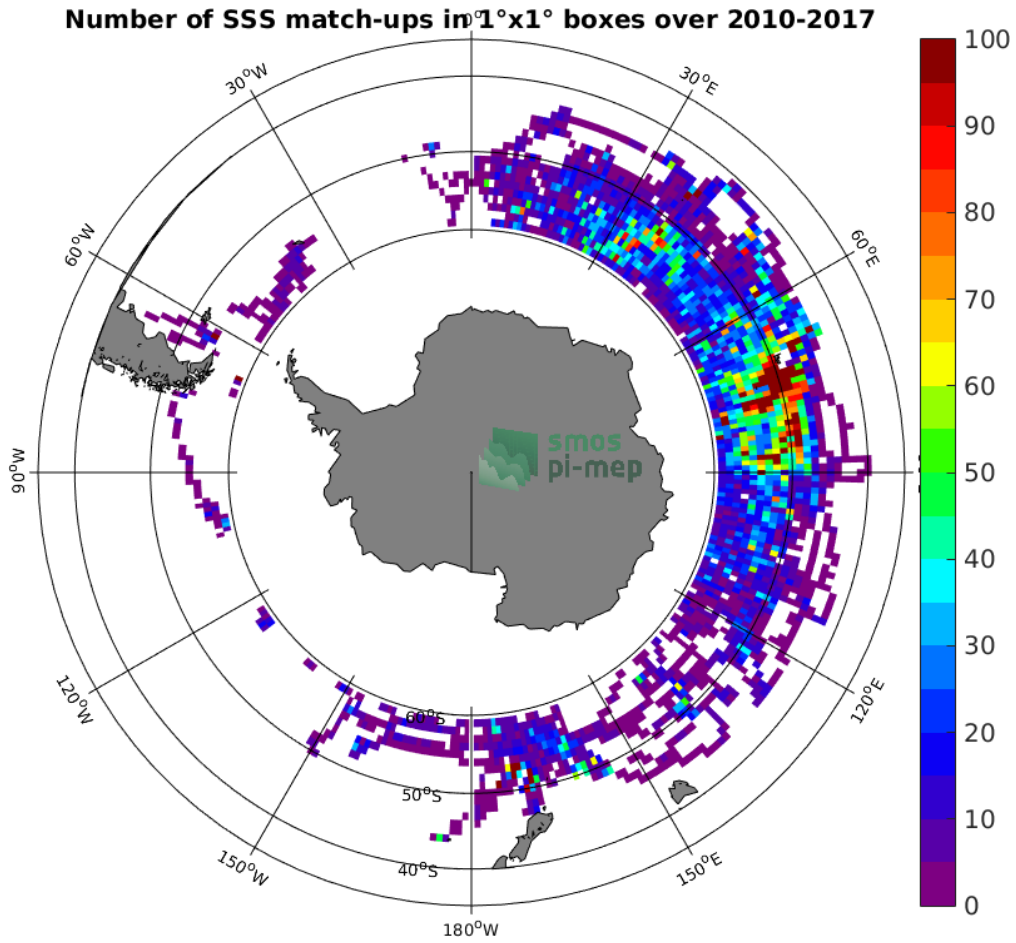
Figure 4: Number of SSS match-ups between Sea mammals SSS and the SMOS-L4-CATDS-CECOS-IFREMER-V2-WEEKLY-0.5DEG SSS product for the Roaring Forties and Furious Fifties Pi-MEP region over 1°x1° boxes and for the full satellite product period.
