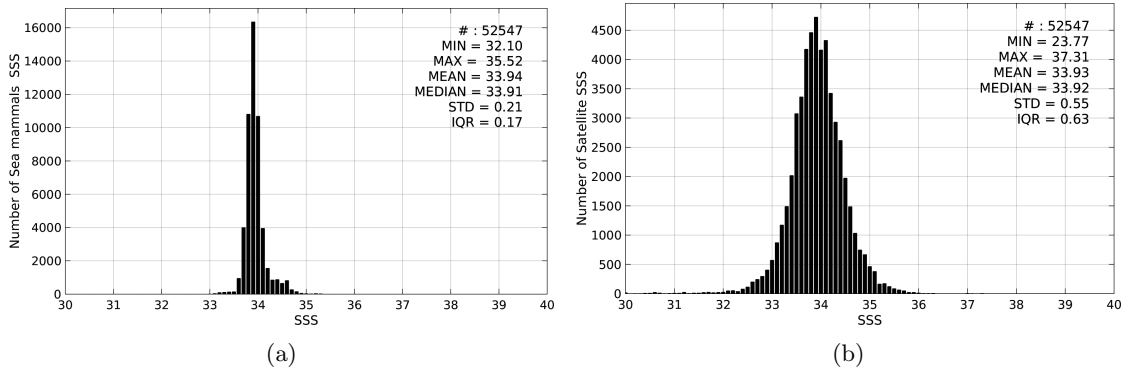
Figure 2: Histograms of SSS from Sea mammals (a) and SMOS-L4-CATDS-CECOS-IFREMER-V2-WEEKLY-0.5DEG (b) considering all match-up pairs per bins of 0.1 over the Roaring Forties and Furious Fifties Pi-MEP region and for the full satellite product period.
