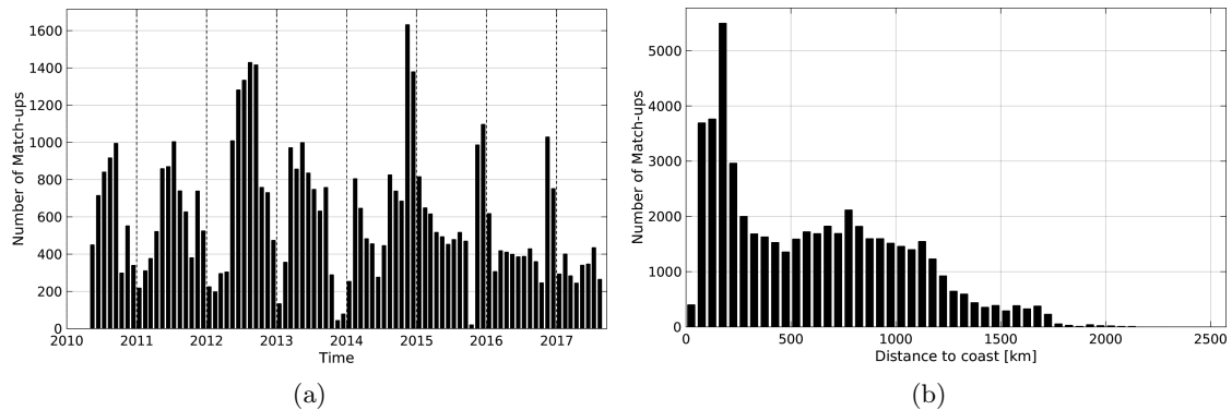
Figure 1: Number of match-ups between Sea mammals and SMOS-L4-CATDS-CECOS-IFREMER-V2-WEEKLY-0.5DEG SSS as a function of time (a) and as function of the distance to coast (b) over the Roaring Forties and Furious Fifties Pi-MEP region and for the full satellite product period.
