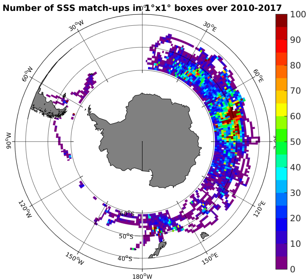
Figure 4: Number of SSS match-ups between Sea mammals SSS and the SMOS-L4-CATDS-CECOS-IFREMER-V2-WEEKLY-0.5DEG SSS product for the Roaring Forties and Furious Fifties Pi-MEP region over 1°x1° boxes and for the full satellite product period.
