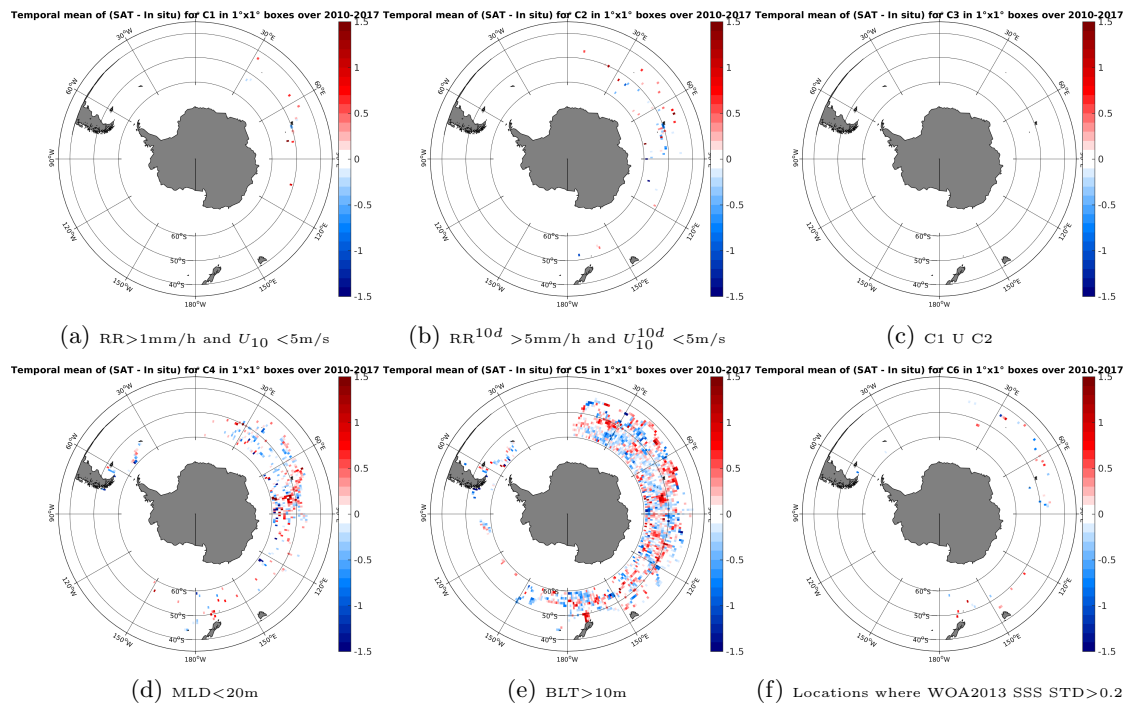
Figure 12: Temporal mean gridded over spatial boxes of size 1^\circ \times 1^\circ of \Delta SSS (SMOS-L4-CATDS-CECOS-IFREMER-V2-WEEKLY-0.5DEG - Sea mammals) for 6 different subdatasets corresponding to: RR > 1\text{mm/h} and U_{10} < 5\text{m/s} (a), RR^{10d} > 5\text{mm/h} and U_{10}^{10d} < 5\text{m/s} (b), C1 U C2 (c), MLD < 20\text{m} (d), BLT > 10\text{m} (e), Locations where WOA2013 SSS STD > 0.2 (f).
