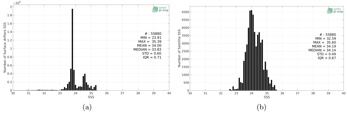
Figure 2: Histograms of SSS from Surface drifters (a) and SMOS L4 v2 Weekly (CATDS-CECOS-IFREMER) (b) considering all match-up pairs per bins of 0.1 over the Roaring Forties and Furious Fifties Pi-MEP region and for the full satellite product period.
