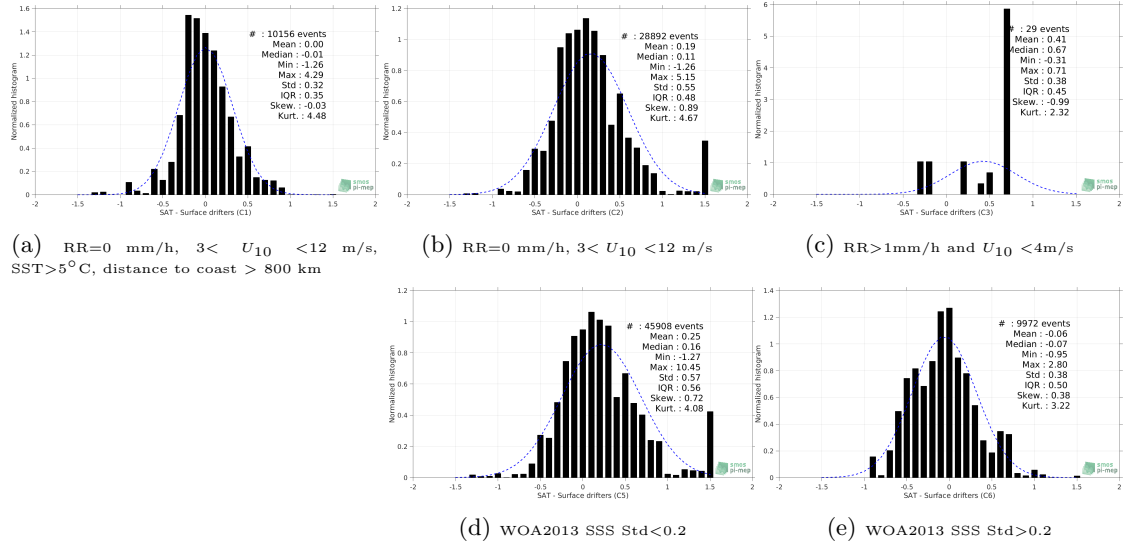
Figure 12: Normalized histogram of \Delta SSS (SMOS-L4-CATDS-CECOS-IFREMER-V2-WEEKLY-0.5DEG - Surface drifters) for 5 different subdatasets corresponding to: RR=0 mm/h, 3 < U_{10} < 12 m/s, SST>5°C, distance to coast > 800 km (a), RR=0 mm/h, 3 < U_{10} < 12 m/s (b), RR>1mm/h and U_{10} < 4 m/s (c), WOA2013 SSS Std<0.2 (d), WOA2013 SSS Std>0.2 (e).
