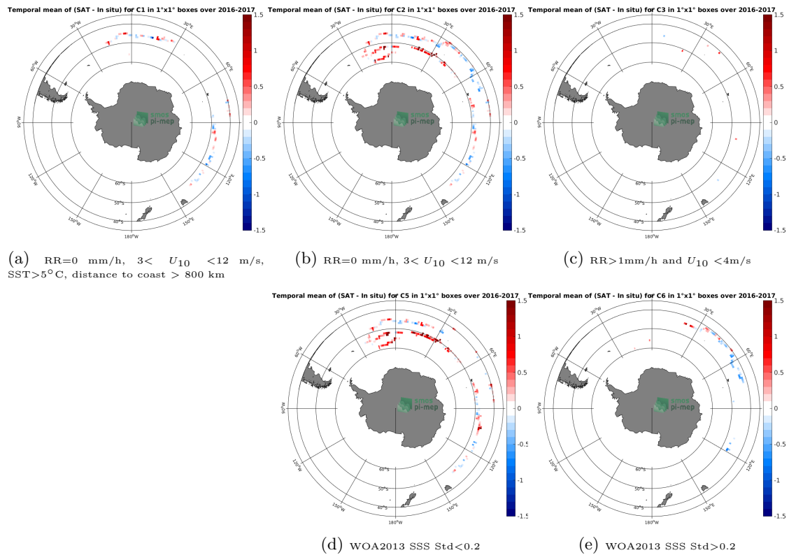
Figure 11: Temporal mean gridded over spatial boxes of size 1^{\circ}\times 1^{\circ} of \Delta\text{SSS} (SMOS-L4-CATDS-CECOS-IFREMER-V2-WEEKLY-0.5DEG - Surface drifters) for 5 different subdatasets corresponding to:RR=0 mm/h, 3 < U_{10} < 12 m/s, SST > 5^{\circ}\text{C} , distance to coast > 800 km (a), RR=0 mm/h, 3 < U_{10} < 12 m/s (b), RR > 1 mm/h and U_{10} < 4 m/s (c), WOA2013 SSS Std < 0.2 (d), WOA2013 SSS Std > 0.2 (e).
