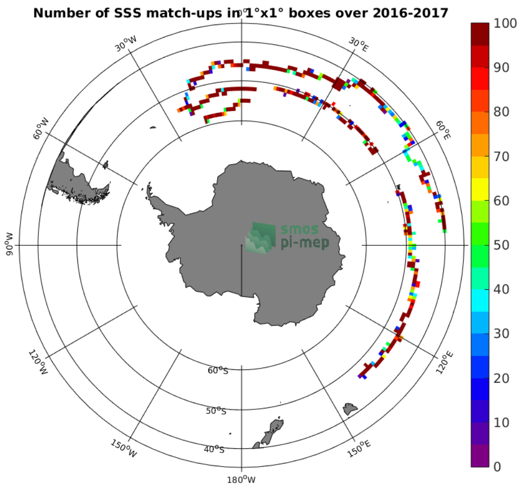
Figure 3: Number of SSS match-ups between Surface drifters SSS and the SMOS-L4-CATDS-CECOS-IFREMER-V2-WEEKLY-0.5DEG SSS product for the Roaring Forties and Furious Fifties Pi-MEP region over 1°x1° boxes and for the full satellite product period.
