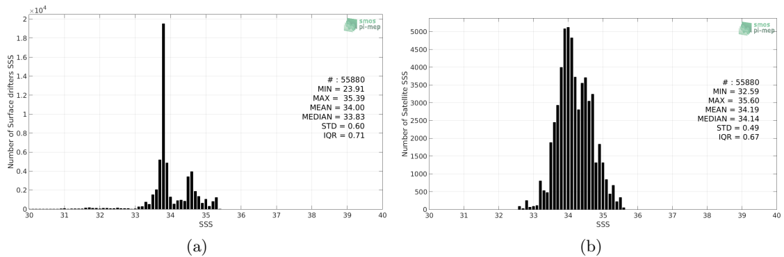
Figure 2: Histograms of SSS from Surface drifters (a) and SMOS-L4-CATDS-CECOS-IFREMER-V2-WEEKLY-0.5DEG (b) considering all match-up pairs per bins of 0.1 over the Roaring Forties and Furious Fifties Pi-MEP region and for the full satellite product period.
