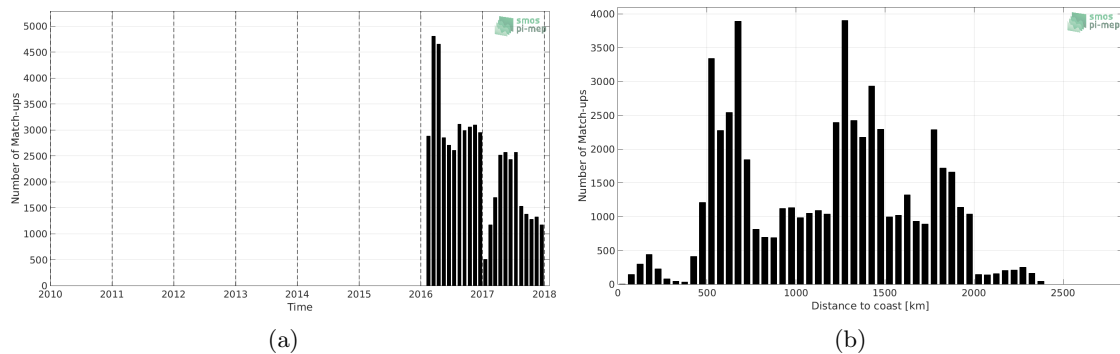
Figure 1: Number of match-ups between Surface drifters and SMOS-L4-CATDS-CECOS-IFREMER-V2-WEEKLY-0.5DEG SSS as a function of time (a) and as function of the distance to coast (b) over the Roaring Forties and Furious Fifties Pi-MEP region and for the full satellite product period.
