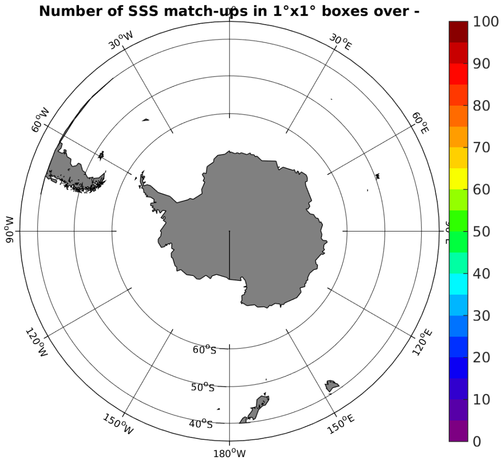
Figure 3: Number of SSS match-ups between Surface drifters SSS and the SMOS-L4-CATDS-CECOS-IFREMER-V2-WEEKLY-0.5DEG SSS product for the Roaring Forties and Furious Fifties Pi-MEP region over 1°x1° boxes and for the full satellite product period.
