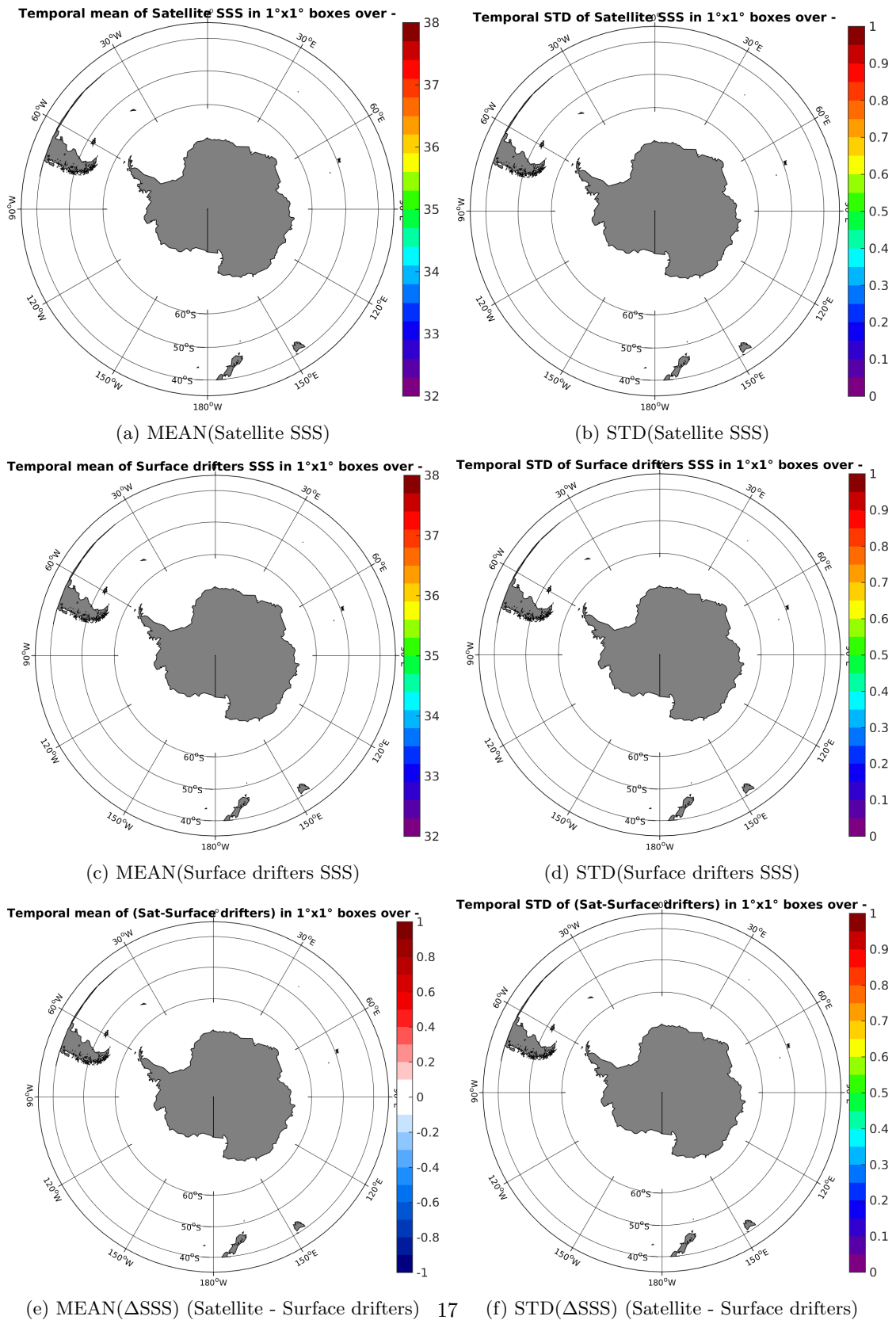
Figure 5: Temporal mean (left) and STD (right) of SSS from SMOS-L4-CATDS-CECOS-IFREMER-V2-WEEKLY-0.5DEG (top), Surface drifters (middle), and of \Delta SSS (Satellite - Surface drifters). Only match-up pairs are used to generate these maps.
