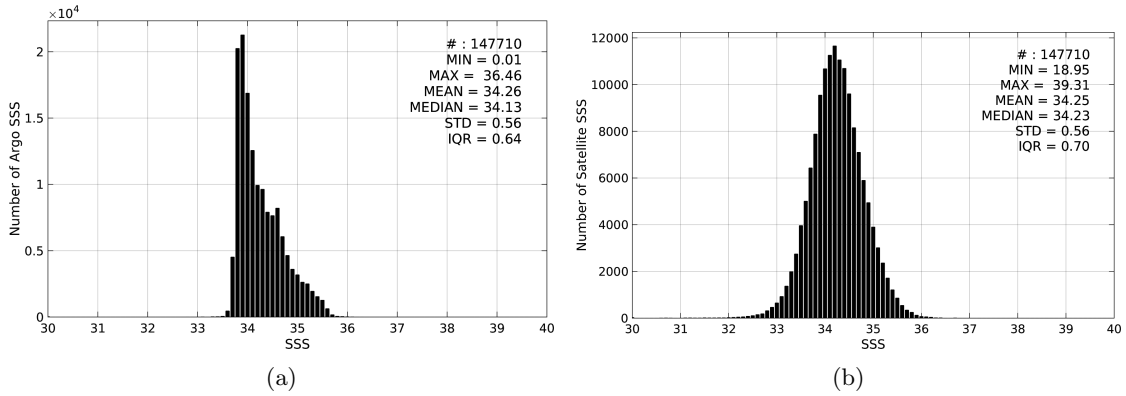
Figure 2: Histograms of SSS from Argo (a) and SMOS-L4-CATDS-CECOS-IFREMER-V2-WEEKLY-0.5DEG (b) considering all match-up pairs per bins of 0.1 over the Roaring Forties and Furious Fifties Pi-MEP region and for the full satellite product period.
