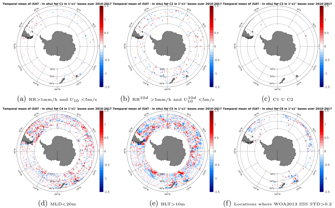
Figure 12: Temporal mean gridded over spatial boxes of size 1^\circ \times 1^\circ of \Delta SSS (SMOS-L4-CATDS-CECOS-IFREMER-V2-WEEKLY-0.5DEG - Argo) for 6 different subdatasets corresponding to: RR > 1\text{mm/h} and U_{10} < 5\text{m/s} (a), RR^{10d} > 5\text{mm/h} and U_{10}^{10d} < 5\text{m/s} (b), C1 U C2 (c), MLD < 20\text{m} (d), BLT > 10\text{m} (e), Locations where WOA2013 SSS STD > 0.2 (f).
