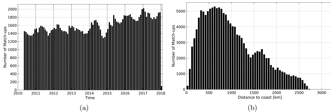
Figure 1: Number of match-ups between Argo and SMOS-L4-CATDS-CECOS-IFREMER-V2-WEEKLY-0.5DEG SSS as a function of time (a) and as function of the distance to coast (b) over the Roaring Forties and Furious Fifties Pi-MEP region and for the full satellite product period.
