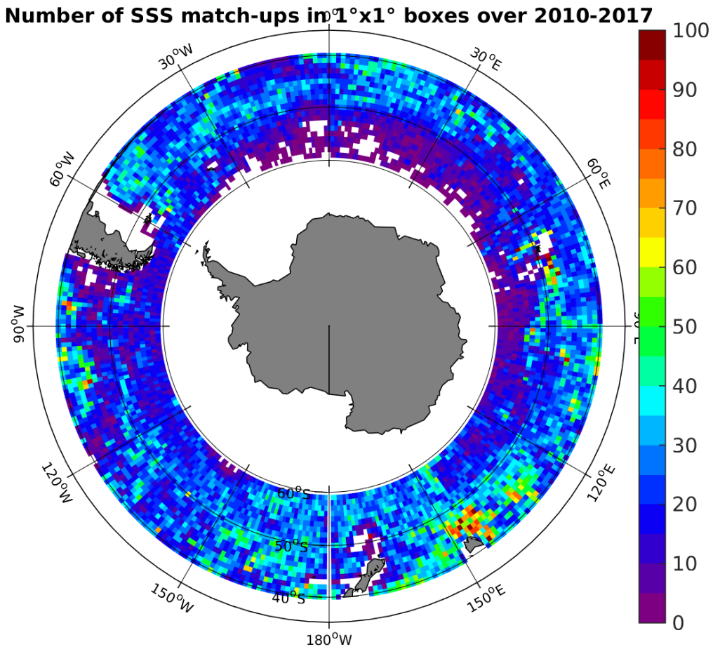
Figure 4: Number of SSS match-ups between Argo SSS and the SMOS-L4-CATDS-CECOS-IFREMER-V2-WEEKLY-0.5DEG SSS product for the Roaring Forties and Furious Fifties Pi-MEP region over 1^\circ \times 1^\circ boxes and for the full satellite product period.
