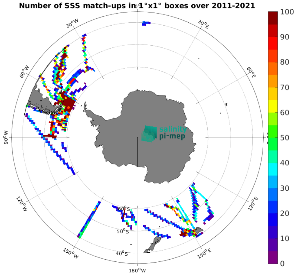
Figure 5: Number of SSS match-ups between TSG (SAMOS) SSS and the SMOS SSS L4 v2 - Daily (BEC) SSS product for the Roaring Forties and Furious Fifties Pi-MEP region over 1^\circ \times 1^\circ boxes and for the full satellite product period.
