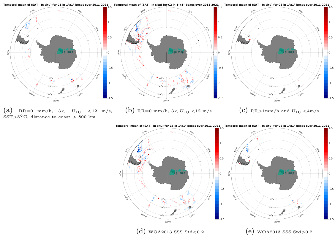
Figure 14: Temporal mean gridded over spatial boxes of size 1^\circ \times 1^\circ of \Delta SSS (SMOS SSS L4 v2 - Daily (BEC) - TSG (SAMOS)) for 5 different subdatasets corresponding to:RR=0 mm/h, 3 < U_{10} < 12 m/s, SST >5^\circ C, distance to coast > 800 km (a), RR=0 mm/h, 3 < U_{10} < 12 m/s (b), RR >1 mm/h and U_{10} < 4 m/s (c), WOA2013 SSS Std <0.2 (d), WOA2013 SSS Std >0.2 (e).
