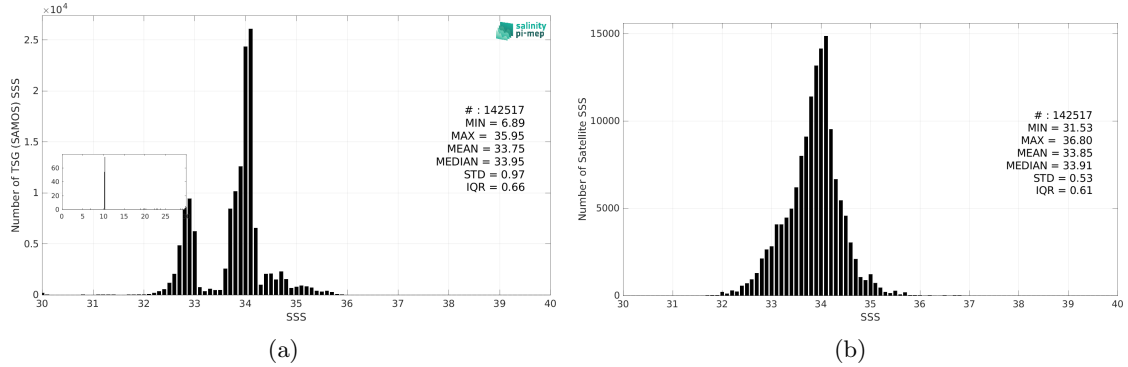
Figure 3: Histograms of SSS from TSG (SAMOS) (a) and SMOS SSS L4 v2 - Daily (BEC) (b) considering all match-up pairs per bins of 0.1 over the Roaring Forties and Furious Fifties Pi-MEP region and for the full satellite product period.
