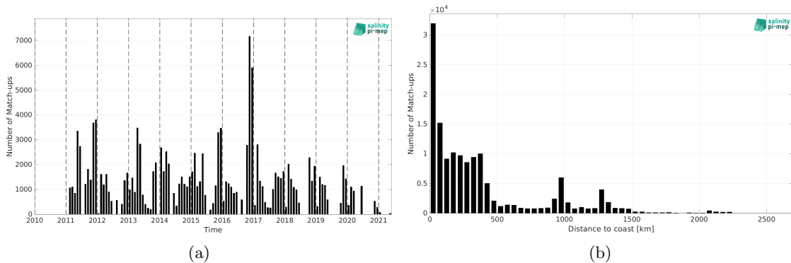
Figure 2: Number of match-ups between TSG (SAMOS) and SMOS SSS L4 v2 - Daily (BEC) SSS as a function of time (a) and as function of the distance to coast (b) over the Roaring Forties and Furious Fifties Pi-MEP region and for the full satellite product period.
