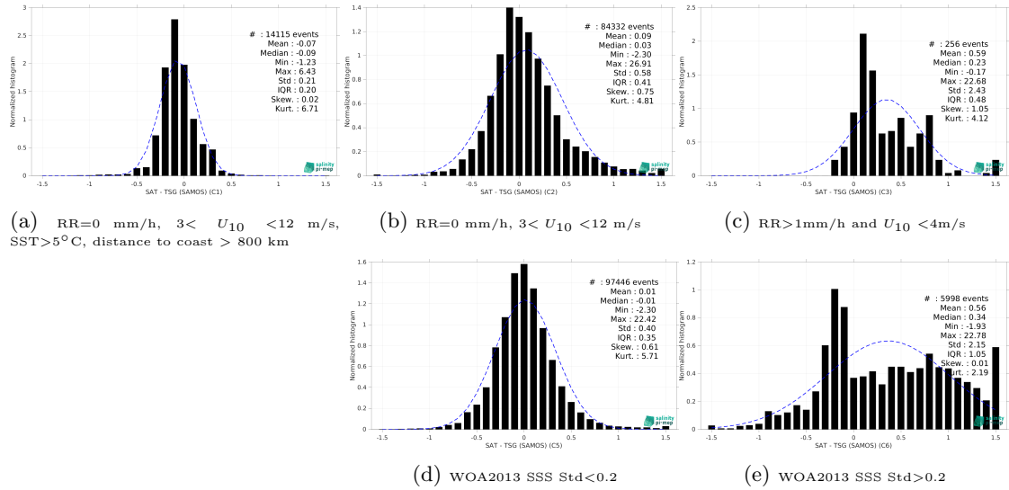
Figure 15: Normalized histogram of \Delta SSS (SMOS SSS L4 v2 - Daily (BEC) - TSG (SAMOS)) for 5 different subdatasets corresponding to: RR=0 mm/h, 3 < U_{10} < 12 m/s, SST>5°C, distance to coast > 800 km (a), RR=0 mm/h, 3 < U_{10} < 12 m/s (b), RR>1mm/h and U_{10} < 4 m/s (c), WOA2013 SSS Std<0.2 (d), WOA2013 SSS Std>0.2 (e).
