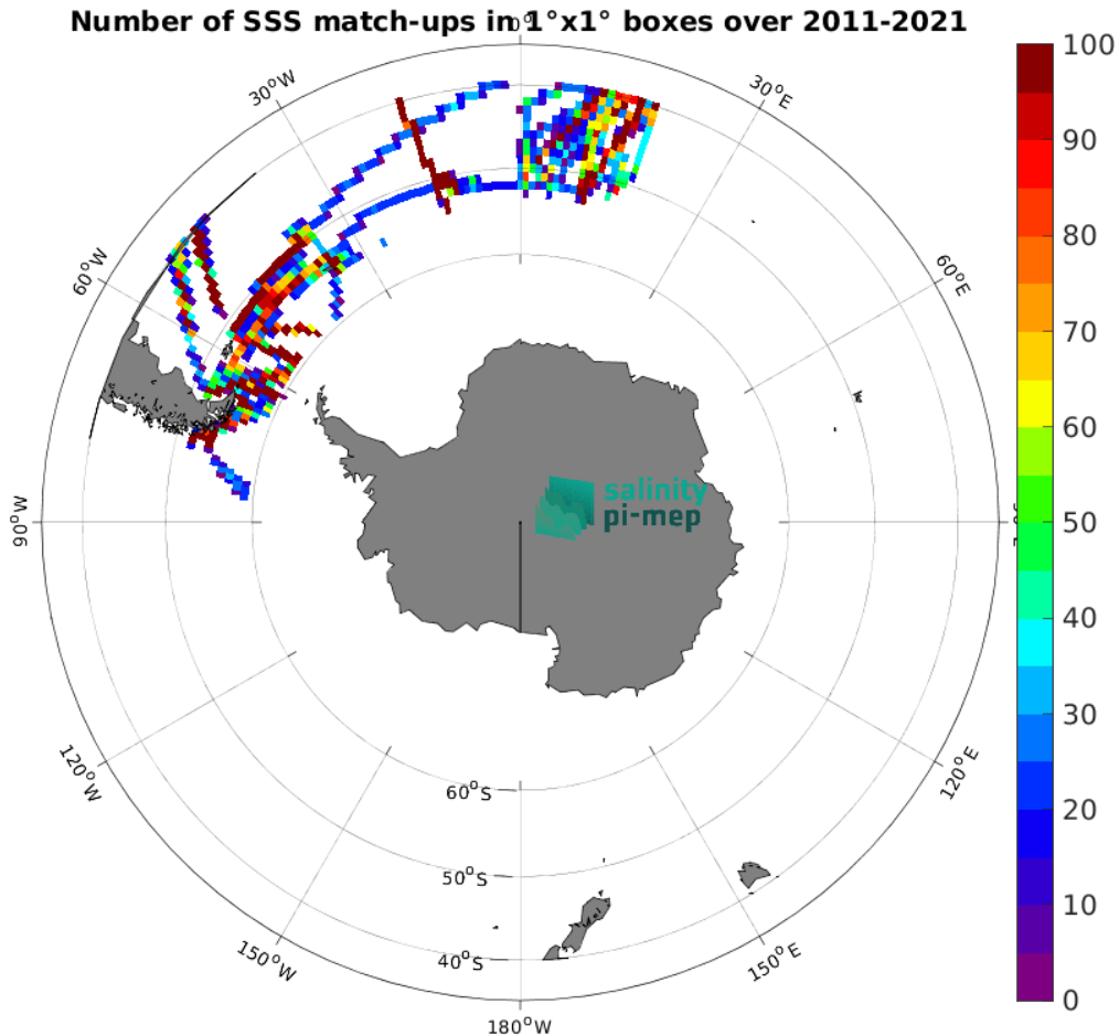
Figure 5: Number of SSS match-ups between TSG (Polarstern) SSS and the SMOS SSS L4 v2 - Daily (BEC) SSS product for the Roaring Forties and Furious Fifties Pi-MEP region over 1^\circ \times 1^\circ boxes and for the full satellite product period.
