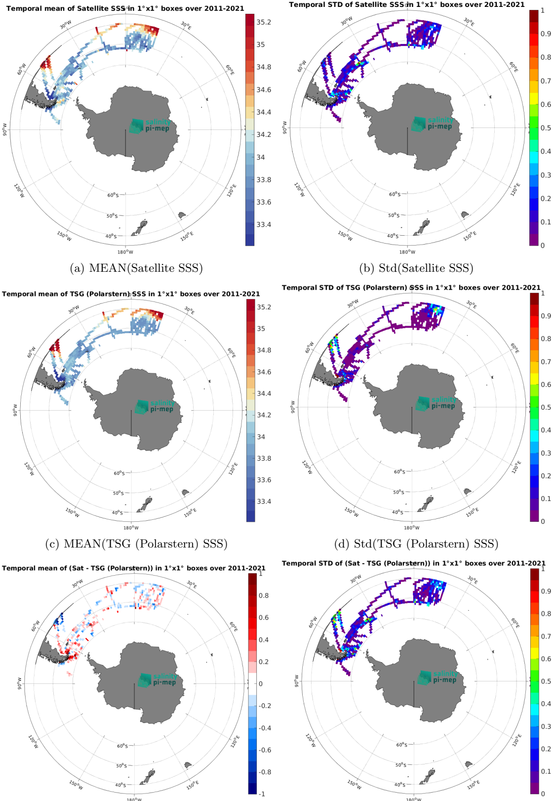
(e) MEAN( \Delta SSS) (Satellite - TSG (Polarstern)) 16 (f) Std( \Delta SSS) (Satellite - TSG (Polarstern)) Figure 7: Temporal mean (left) and Std (right) of SSS from SMOS SSS L4 v2 - Daily (BEC) (top), TSG (Polarstern) (middle), and of \Delta SSS (Satellite - TSG (Polarstern)). Only match-up pairs are used to generate these maps.
