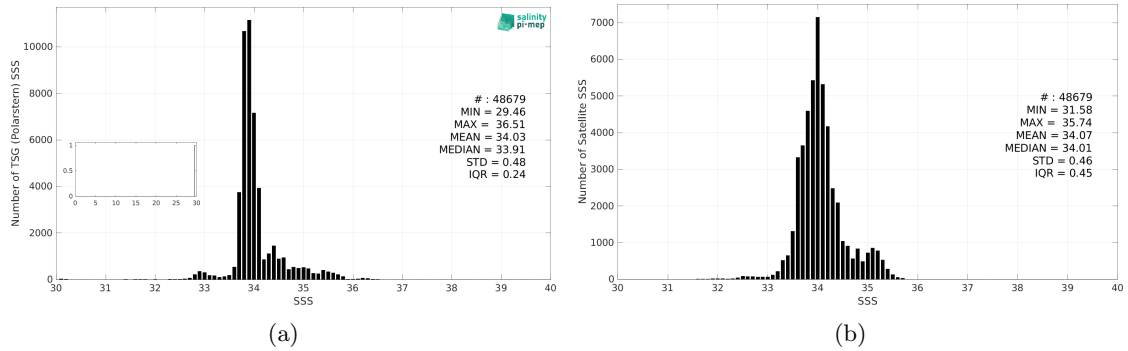
Figure 3: Histograms of SSS from TSG (Polarstern) (a) and SMOS SSS L4 v2 - Daily (BEC) (b) considering all match-up pairs per bins of 0.1 over the Roaring Forties and Furious Fifties Pi-MEP region and for the full satellite product period.
