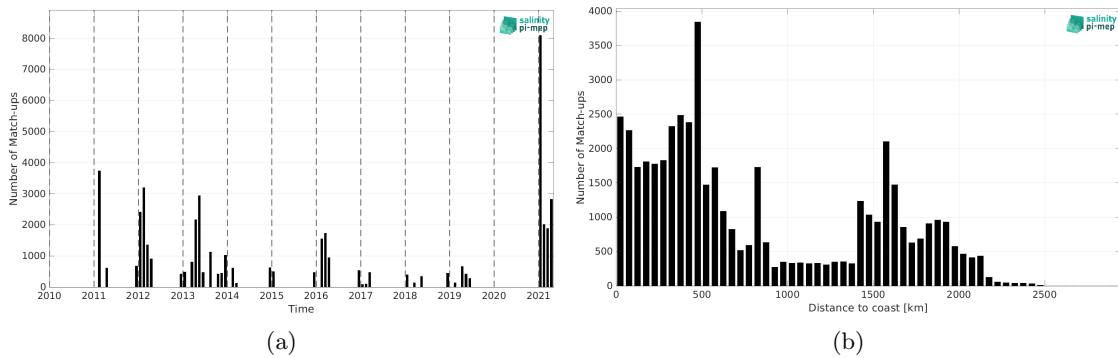
Figure 2: Number of match-ups between TSG (Polarstern) and SMOS SSS L4 v2 - Daily (BEC) SSS as a function of time (a) and as function of the distance to coast (b) over the Roaring Forties and Furious Fifties Pi-MEP region and for the full satellite product period.
