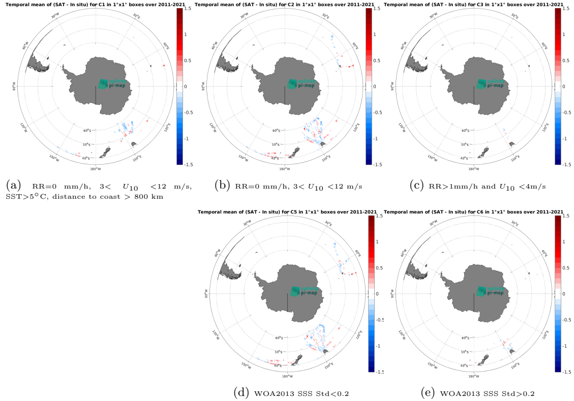
Figure 12: Temporal mean gridded over spatial boxes of size 1^{\circ}\times 1^{\circ} of \Delta\text{SSS} (SMOS SSS L4 v2 - Daily (BEC) - TSG (LEGOS-DM)) for 5 different subdatasets corresponding to: \text{RR}=0 mm/h, 3 < U_{10} < 12 m/s, \text{SST}>5^{\circ}\text{C} , distance to coast > 800 km (a), \text{RR}=0 mm/h, 3 < U_{10} < 12 m/s (b), \text{RR}>1\text{mm/h} and U_{10} < 4\text{m/s} (c), WOA2013 SSS Std < 0.2 (d), WOA2013 SSS Std > 0.2 (e).
